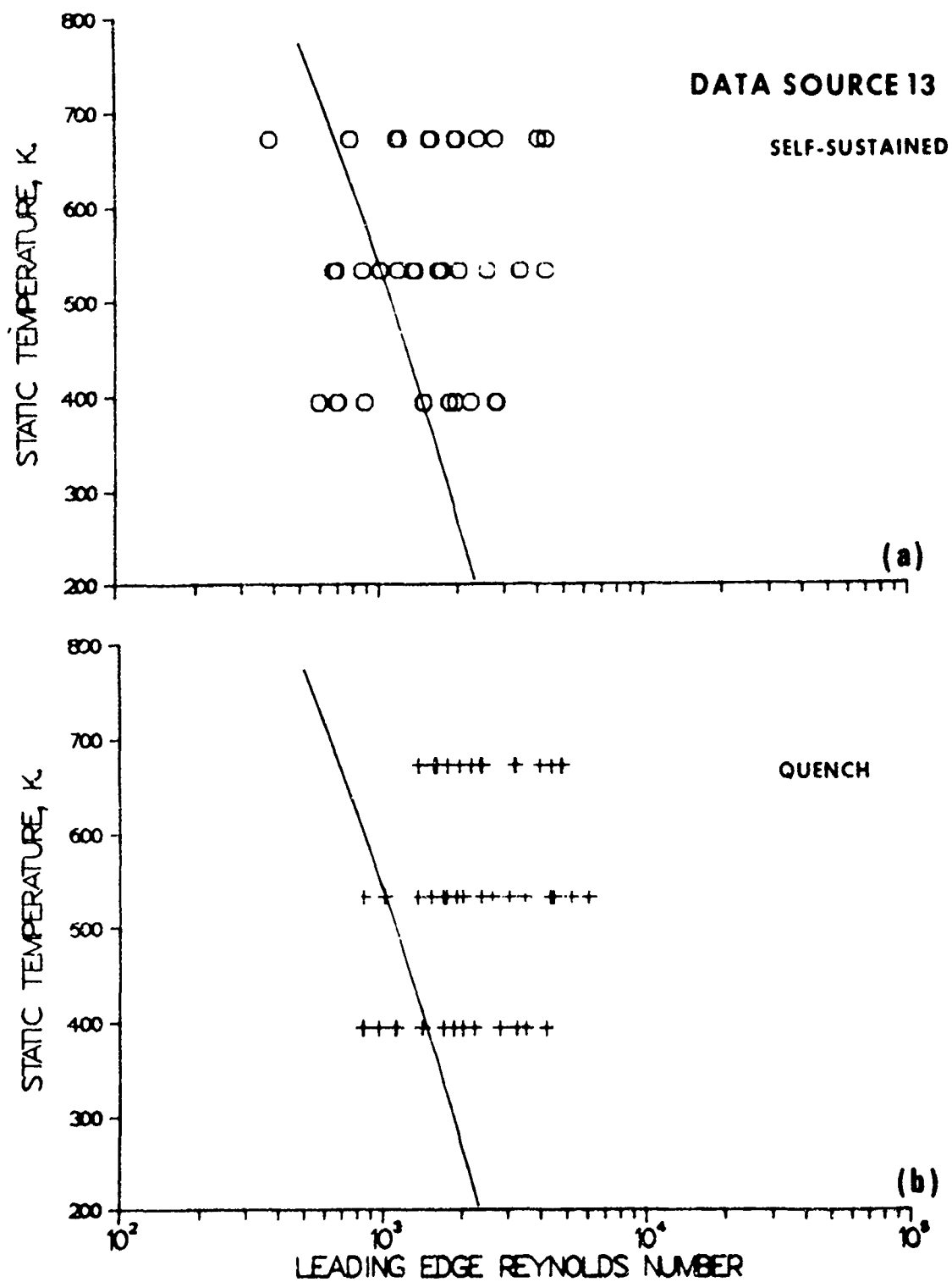
Figure 23. Experimental titanium combustion data from reference 13.
