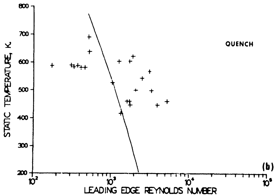
Figure 20. Experimental titanium combustion data from reference 10.
