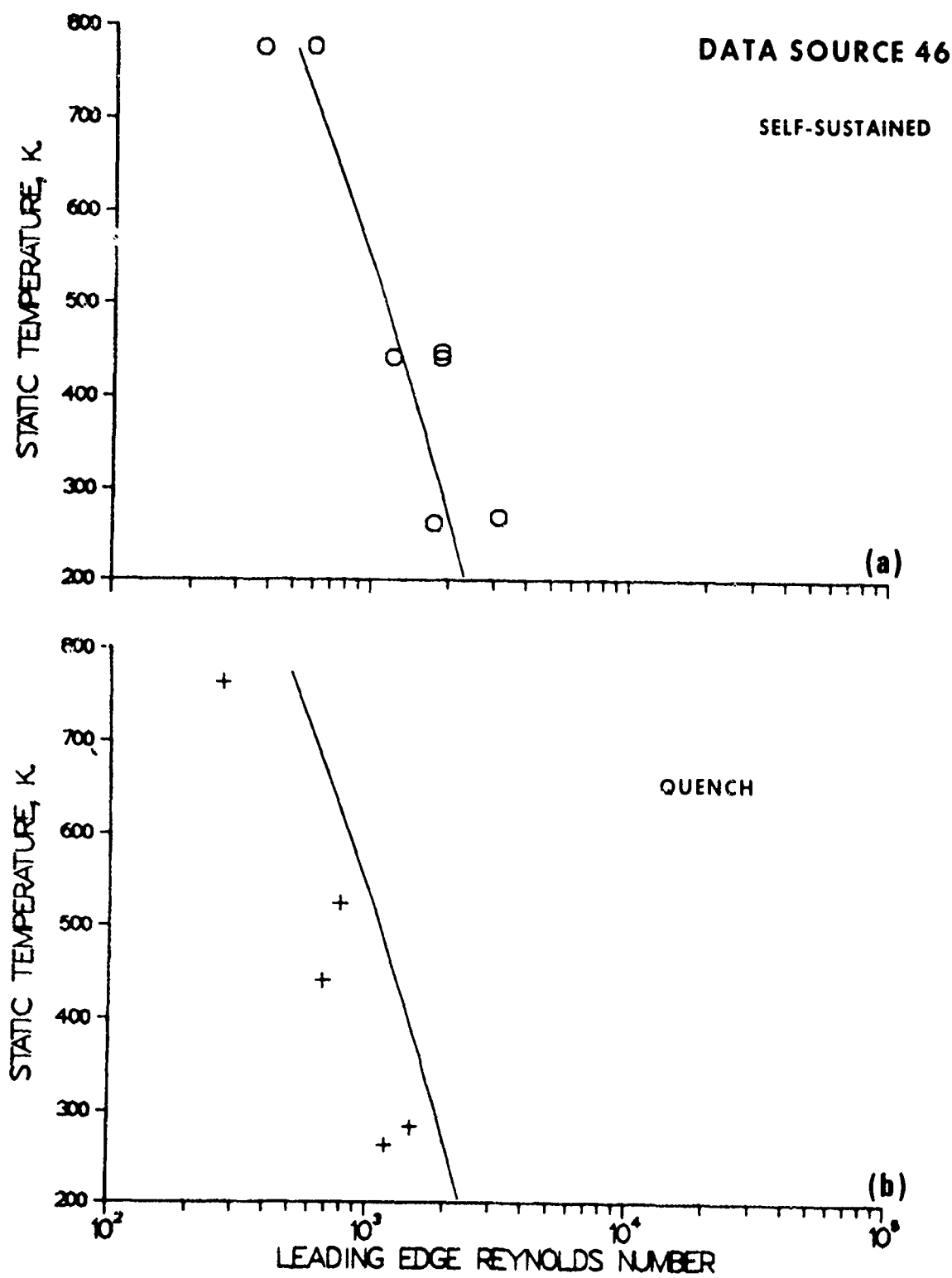
Figure 21. Experimental titanium combustion data from reference 46.
