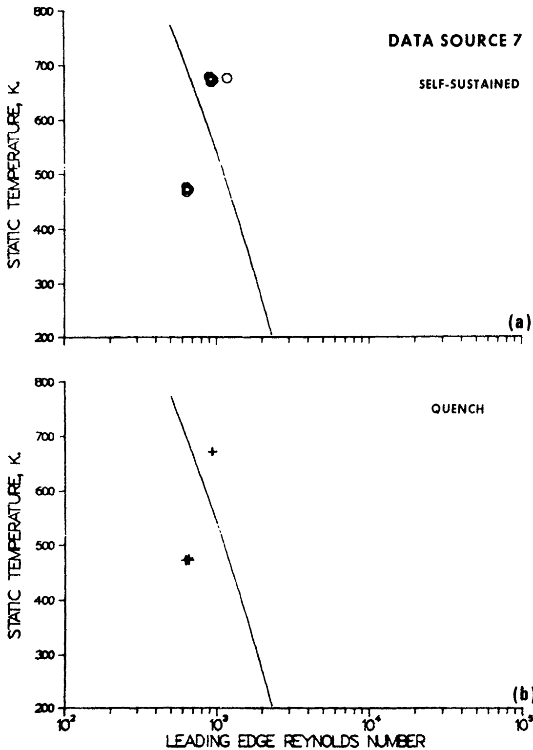
Figure 22. Experimental titanium combustion data from reference 7.
