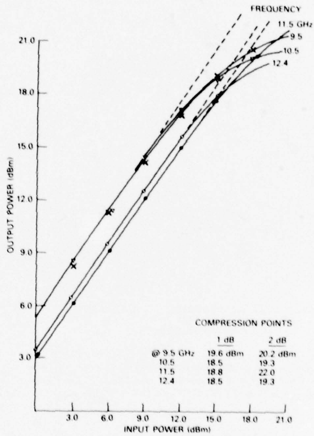
Fig. 24 — Single-ended GaAs MESFET amplifier power response. Device: dual-cell GaAs MESFET. Cell size: 300 \mu\text{m} ( V_w ) \times 0.8 \mu\text{m} ( V_g ). Bias: 6.0 VDC ( V_{DS} ), -0.7 VDC ( V_{GS} ).
