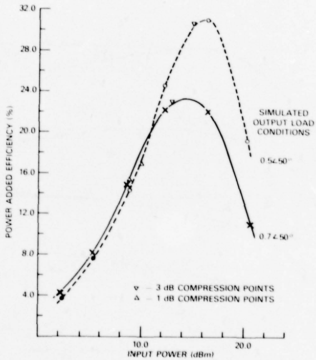
Fig. 10 — Measured power-added efficiency of a single-cell GaAs MESFET. Cell size: 300 \mu\text{m} ( l_w ) \times 1.0 \mu\text{m} ( l_g ). Bias: 8.0 VDC ( V_{DS} ), -1.0 VDC ( V_{GS} ).
