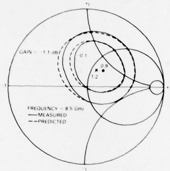
Fig. 5 — Measured and predicted constant power gain contours at 8.5 GHz plotted in the output load reflection plane (input port untuned). Input power: 20 dBm. Device: GaAs MESFET, 600\ \mu\text{m} ( \ell_w ) \times 1.7\ \mu\text{m} ( \ell_g ). Bias: 6.0 VDC ( V_{DS} ), -2.0 VDC ( V_{GS} ).
