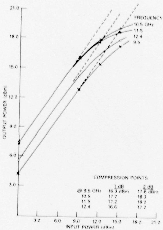
Fig. 21 — Single-ended GaAs MESFET amplifier power response. Device: single-cell GaAs MESFET. Cell size: 300 \mu\text{m} ( V_w ) \times 0.8 \mu\text{m} ( V_g ). Bias: 4.0 VDC ( V_{DS} ), -0.7 VDC ( V_{GS} ).
