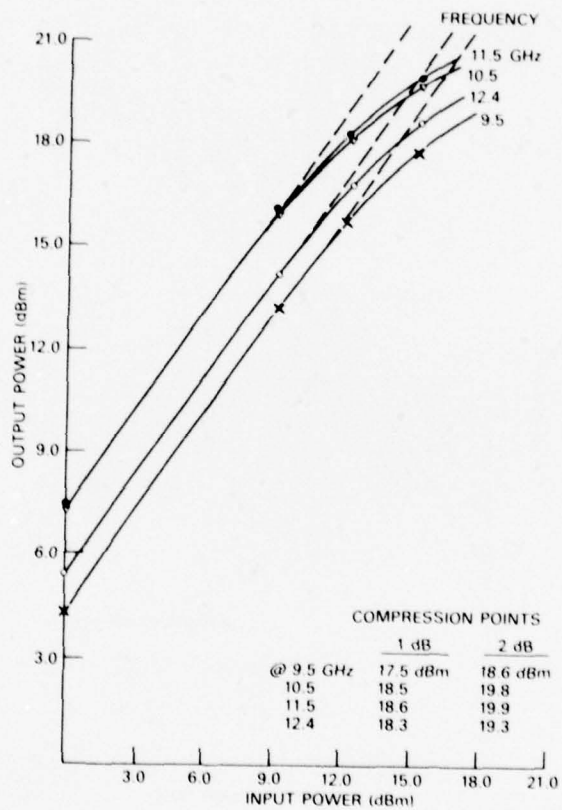
Fig. 22 — Single-ended GaAs MESFET amplifier power response. Device: single-cell GaAs MESFET. Cell size: 300 \mu\text{m} ( \ell_w ) \times 0.8 \mu\text{m} ( \ell_g ). Bias: 6.0 VDC ( V_{DS} ), -0.7 VDC ( V_{GS} ).
