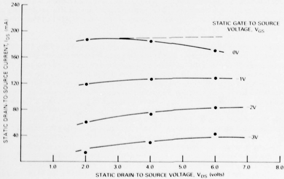
Fig. 20 — Measured static (DC) I_{DS} - V_{DS} curves of a dual-cell GaAs MESFET. Cell size: 300 \mu\text{m} ( \ell_w ) \times 0.8 \mu\text{m} ( \ell_g ).
