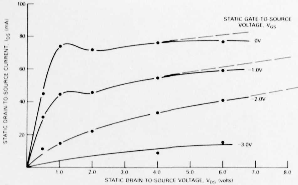
Fig. 19 — Measured static (DC) I_{DS} - V_{DS} curves of a single-cell GaAs MESFET. Cell size: 300 \mu\text{m} ( \ell_w ) \times 0.8 \mu\text{m} ( \ell_g ).
