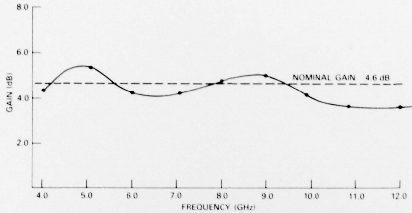
Fig. B7 — Computed 4- to 12-GHz GaAs MESFET amplifier response. Device: Texas Instruments, Inc. GaAs MESFET. Cell Size: 1200 \mu\text{m} ( \ell_w ) \times 1 \mu\text{m} ( \ell_g ). Bias: 6.0 \text{ VDC} ( V_{DS} ), -2.0 \text{ VDC} ( V_{GS} ).
