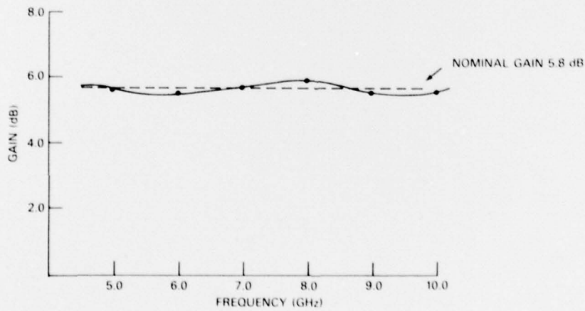
Fig. B8 — Computed 5- to 10-GHz GaAs MESFET amplifier response. Device: Texas Instruments, Inc. GaAs MESFET. Cell size: 1200 \mu\text{m} ( \ell_w ) \times 1 \mu\text{m} ( \ell_g ). Bias: 6.0 \text{ VDC} ( V_{DS} ), -2.0 \text{ VDC} ( V_{GS} ).
