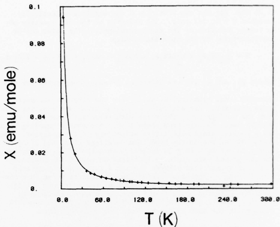
Figure 3. The magnetic susceptibility data for di- \mu -oxobis-[bis(2,2'-bipyridine)manganese (III,IV)]. The experimental data are given by +, and the solid line is the best fit to the expression for an exchange coupled S = 2, 3/2 pair.
