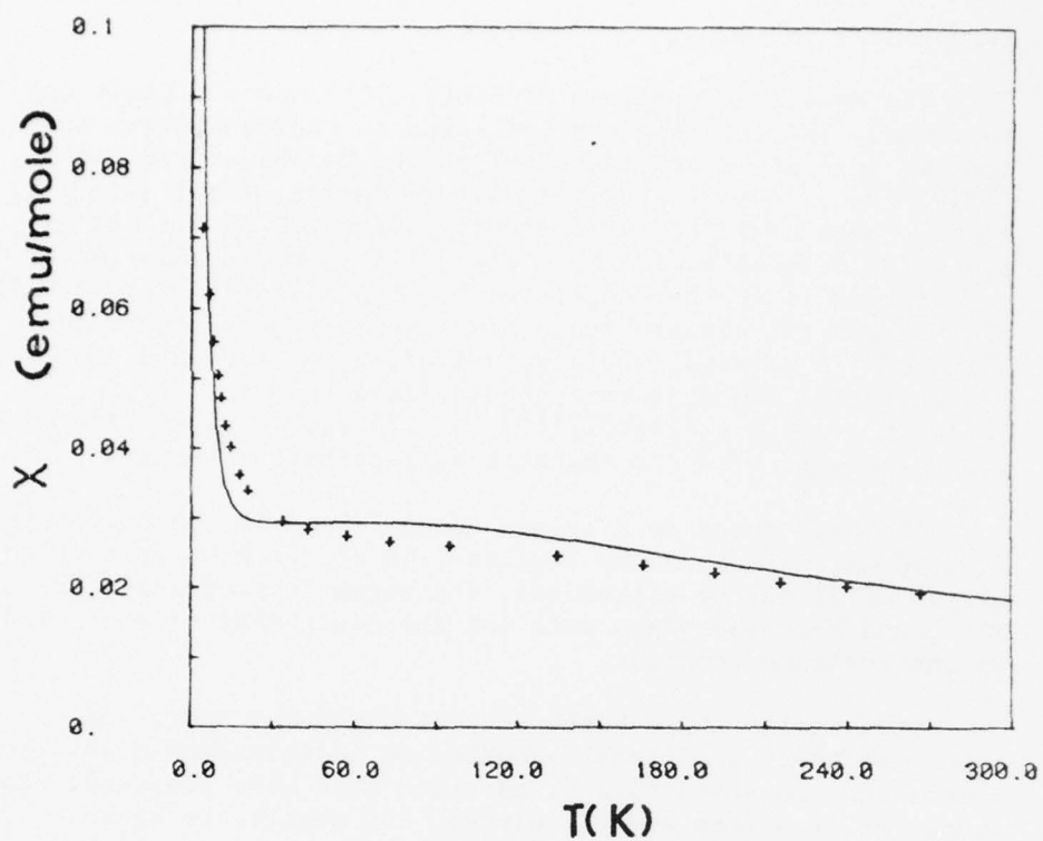
Figure 4. Magnetic susceptibility data for \mu -oxo-bis[salen Fe(III,IV)].
