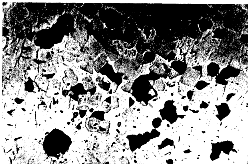
(b) Fired at 3270°F. (Ti and \text{TiB}_2 pre-reacted at 3400°F.) Dark grey areas in center of photo appear brassy under the microscope and are identified as TiO.
