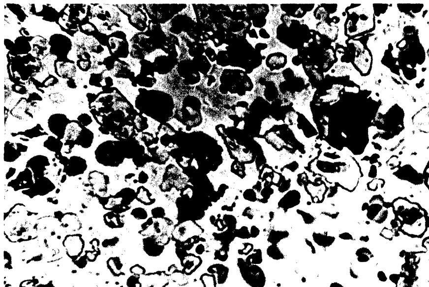
(a) Fired at 3400°F. Etched 10 min. in a solution consisting of 4 parts 48% HF, plus 2 parts conc. HNO 3 plus 94 parts methanol. Dark grey areas are TiO which seems to be more prevalent in regions where voids occur.
