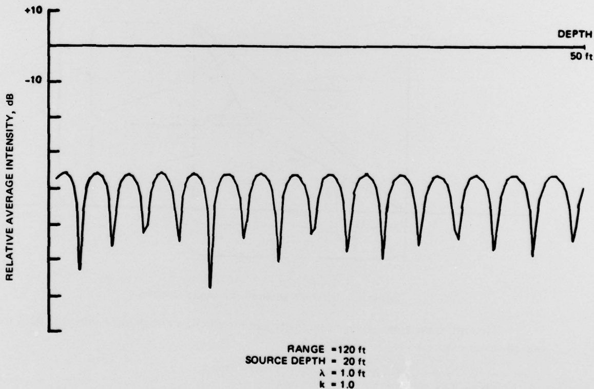
Figure 5. Relative average intensity vs depth for a single source and a point receiver at a fixed distance.
