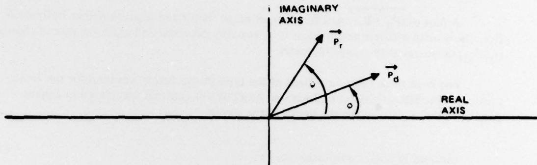
Figure 3. Geometric representation of complex numbers.
