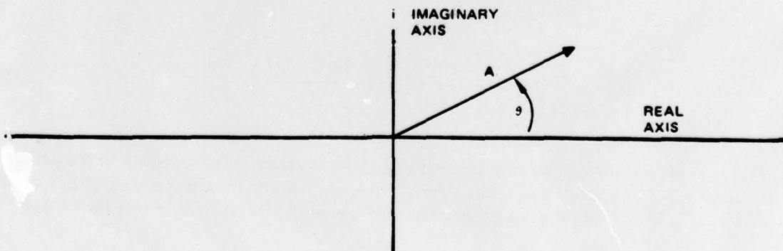
Figure 2. Plot illustrating complex numbers.
