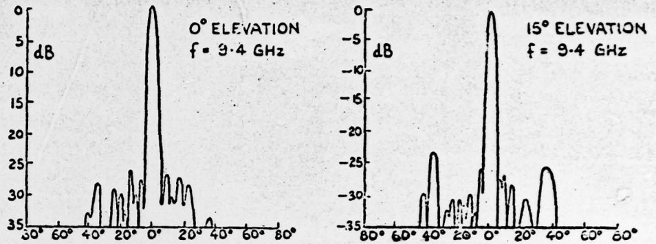
FIG 4a RADIATION PATTERNS OF A LINEAR ARRAY OF 24 SLOTS
