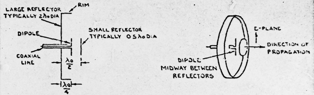
FIG. 2a. SHORT BACKFIRE ANTENNA WITH DIPOLE FEED
