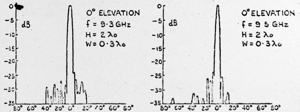
FIG 4c RADIATION PATTERNS OF ARRAY WITH MULTIPLE REFLECTION APERTURE
