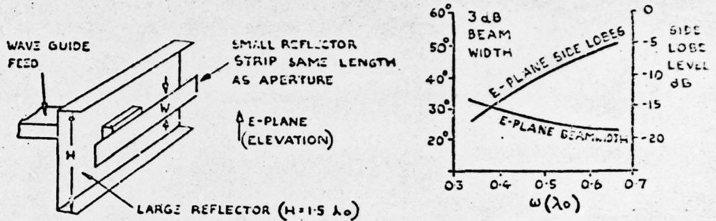
FIG. 3a. WAVEGUIDE FED ANTENNA WITH TROUGH MULTI-REFLECTION APERTURE
