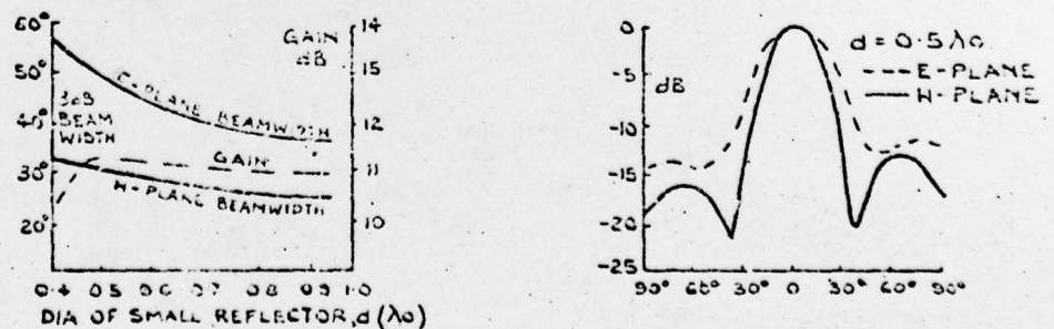
FIG. 2d. RADIATION PROPERTIES OF ANTENNA SHOWN IN FIG. 2b (FLUSH FEED)
