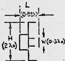
SECTION OF MRA ANTENNA
