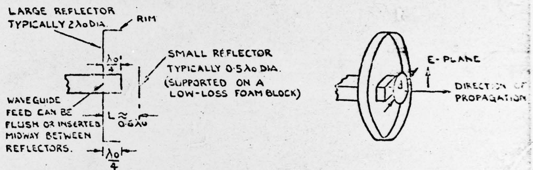
FIG. 2b. WAVEGUIDE FED VERSION OF ANTENNA
