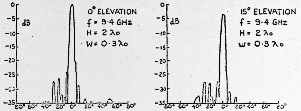
FIG.4b RADIATION PATTERNS OF ARRAY WITH MULTIPLE REFLECTION APERTURE
