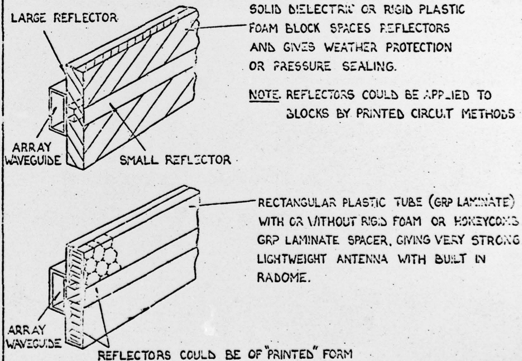
FIG. 6b. POSSIBLE METHODS OF ANTENNA CONSTRUCTION
