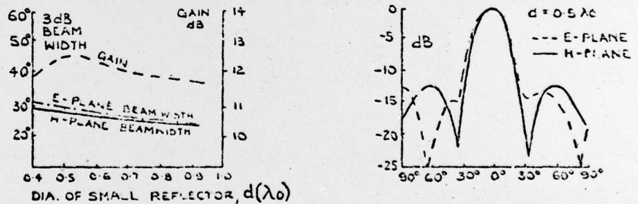
FIG. 2c. RADIATION PROPERTIES OF ANTENNA SHOWN IN FIG. 2b (INSERTED FEED)
