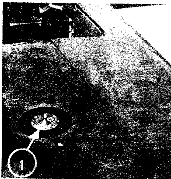
Figure 5 External View of Belly of Test Aircraft Showing Electric Field Meter Detector Head
