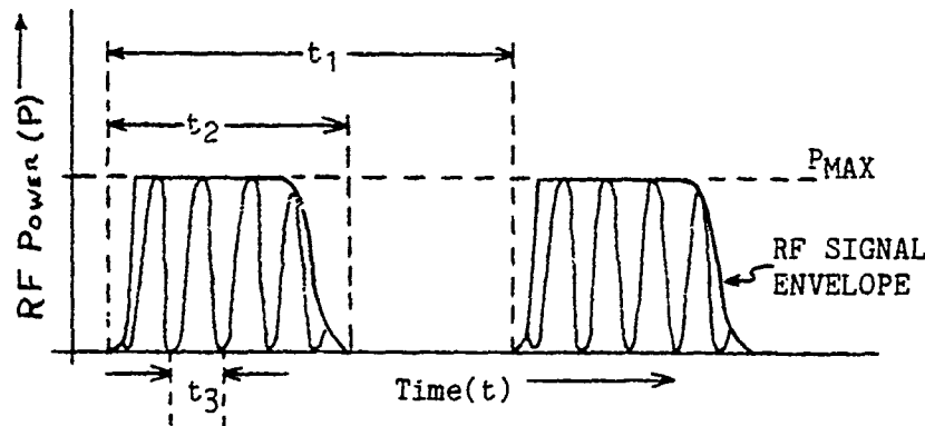
Figure 2.2. RF Energy Pulse Packages. t_1 = 1/PRR , determined by synchronizer, one transmit/receive cycle; t_2 = \text{Pulse Width (PW)} , determined by the modulator; t_3 = 1/f , f is the characteristic frequency of the radar set, determined by the RF generator; P_{MAX} = \text{Maximum Transmitted power} , determined by the modulator and RF power amplifier; RF Signal Envelope, determined by the form of the modulator pulse.
