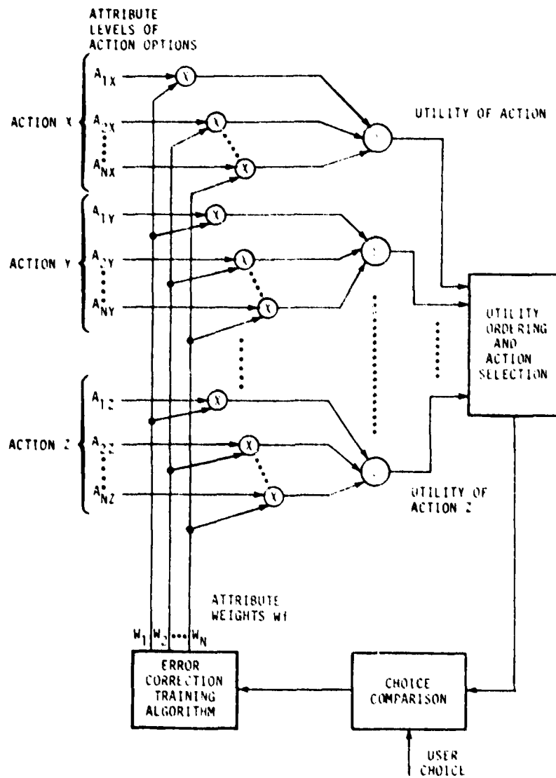
Figure 5. Adaptive Multi-Attribute Decision Mechanism
