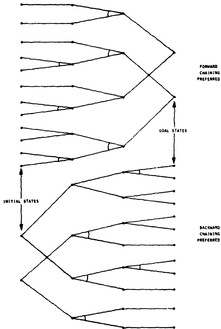
Figure 16. And/Or Graph Shapes for Forward or Backward Chaining
