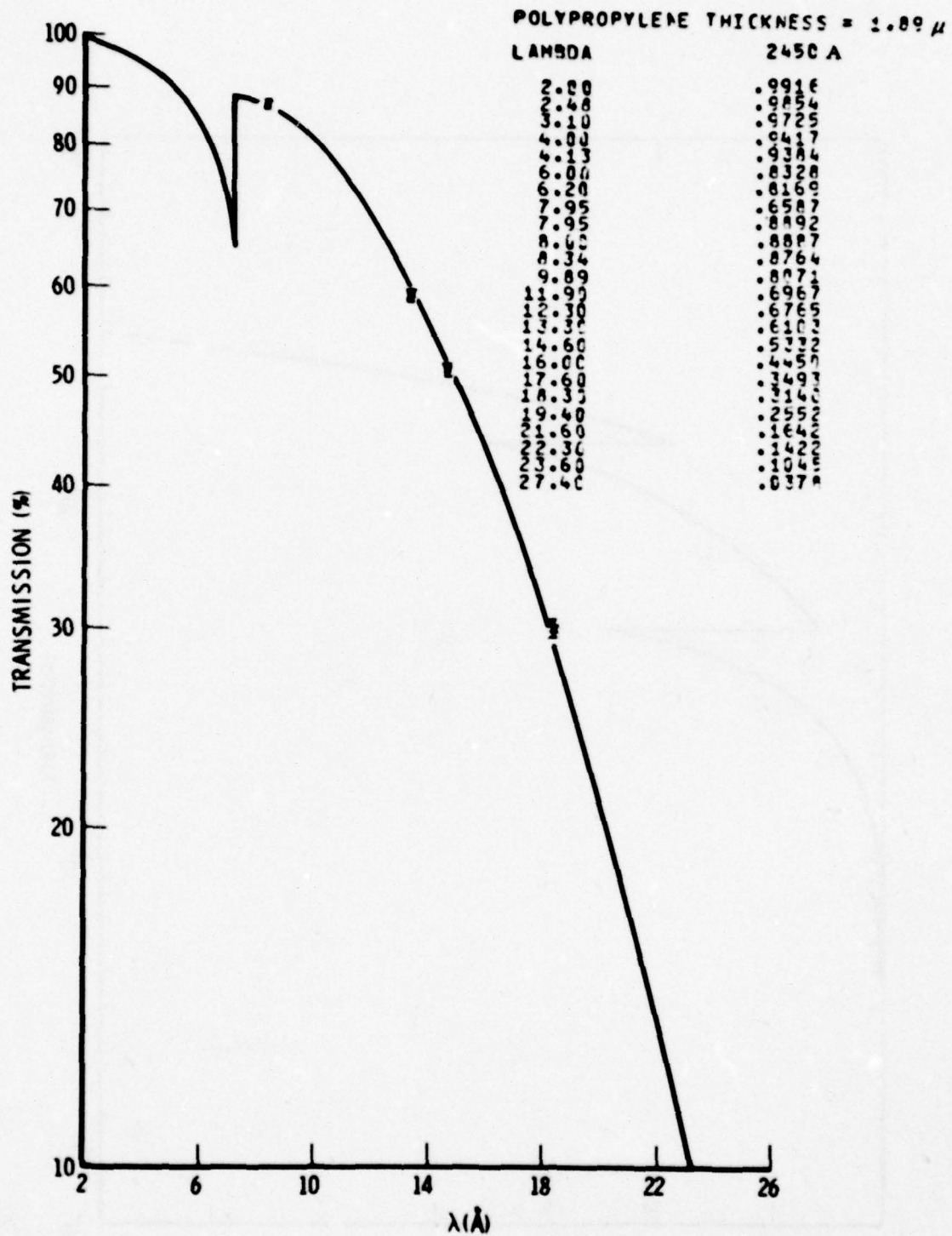
Figure 3.15. Combined Transmission of the Two SOLEX Filters (Flight Unit). The theoretical transmission of a shield consisting of 1.89 \mu m of polypropylene and 2450 Å of aluminum is given by the solid curve and the table insert. Experimental values are also noted.
