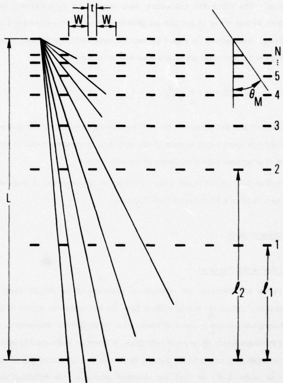
Figure 3.2. Optimum Procedure for Placing Collimator Grids. Each grid just blocks radiation passing through the grid below it.
