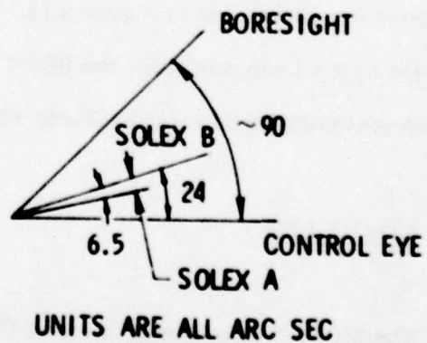
Figure 2.13. CRLS-229 Alignment Summary.
