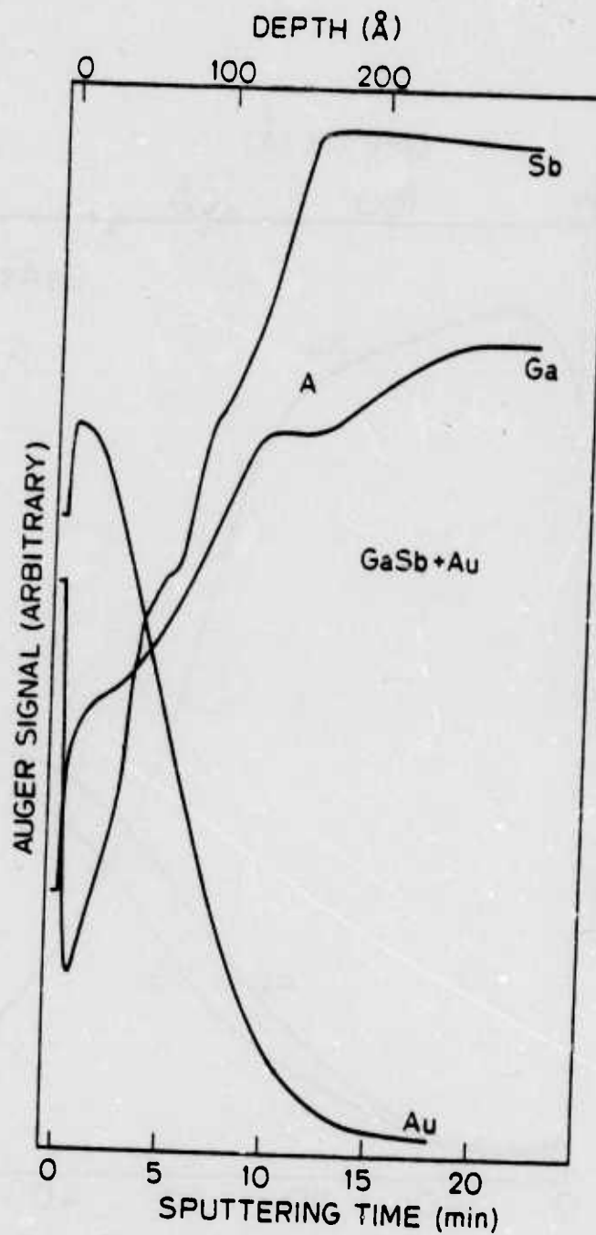
Fig. 4. COMPOSITIONAL DEPTH PROFILE OF Au COVERED GaSb OBTAINED USING AUGER ELECTRONIC SPECTROSCOPY IN COMBINATION WITH ARGON ION ETCHING.
