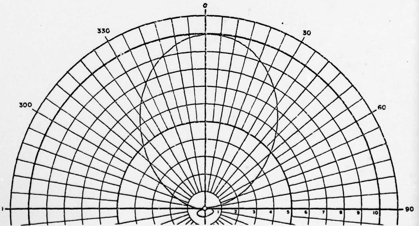
Voltage Patterns, 150 MHz FIGURE A-3
