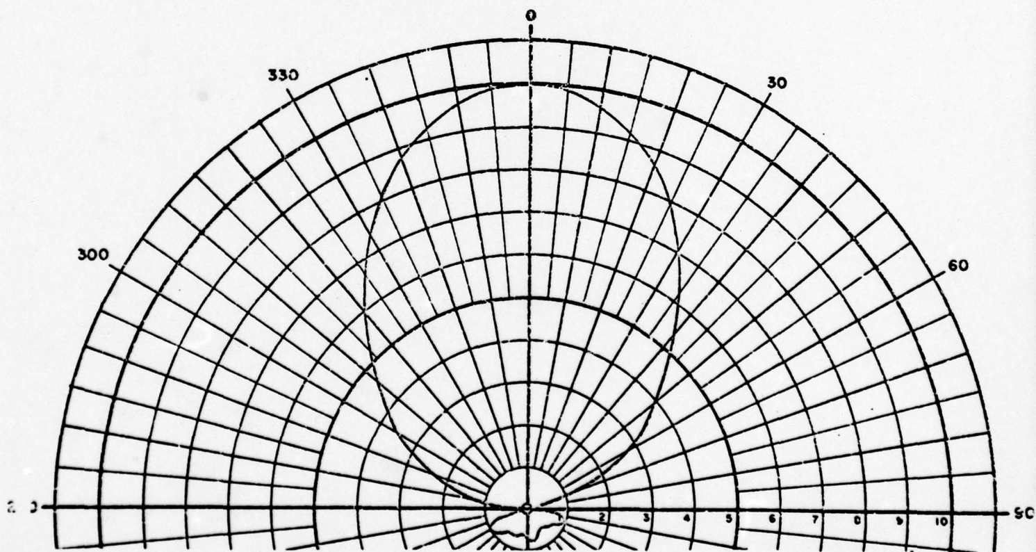
Voltage Patterns, 300 MHz FIGURE A-8
