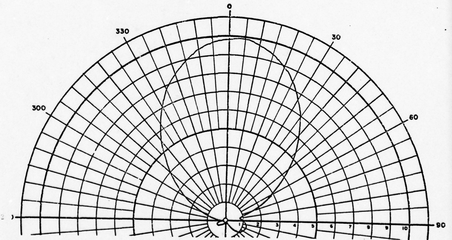
Voltage Patterns, 220 MHz FIGURE A-5
