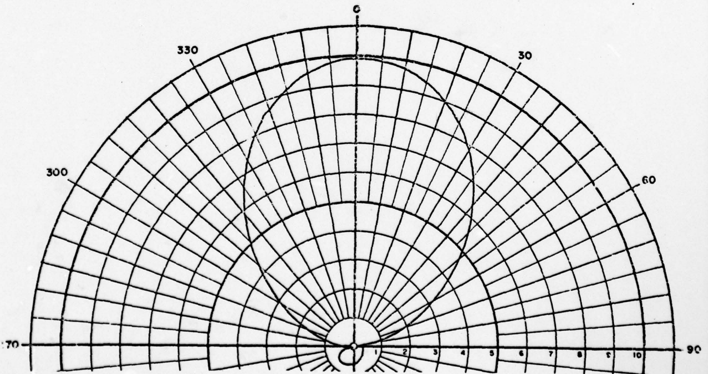
Voltage Patterns, 125 MHz FIGURE A-2
