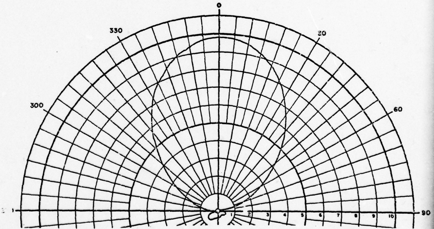
Voltage Patterns, 250 MHz FIGURE A-6
