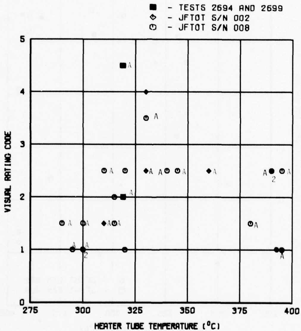
FIGURE 2. VISUAL RATINGS FOR BATCH 32
