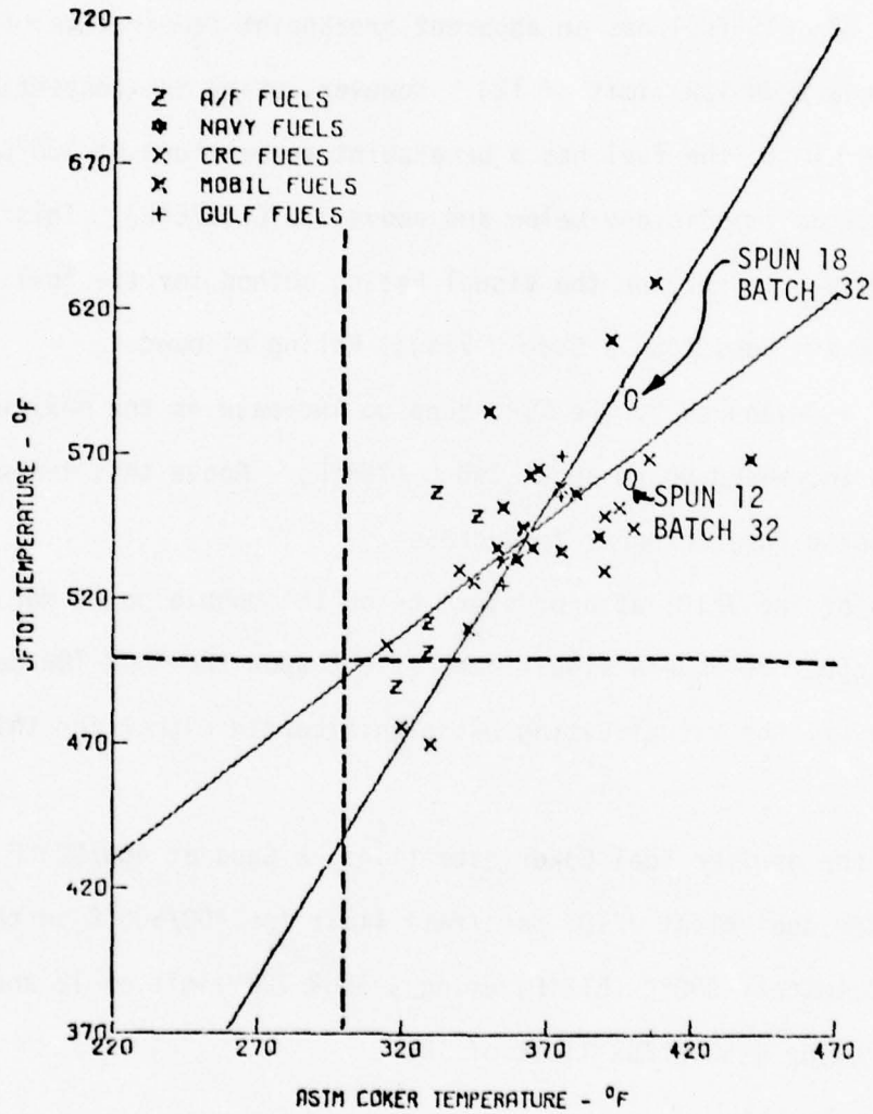
FIGURE 3. SPUN 18 TUBE DEPOSIT RATING CORRELATION RESULTS
