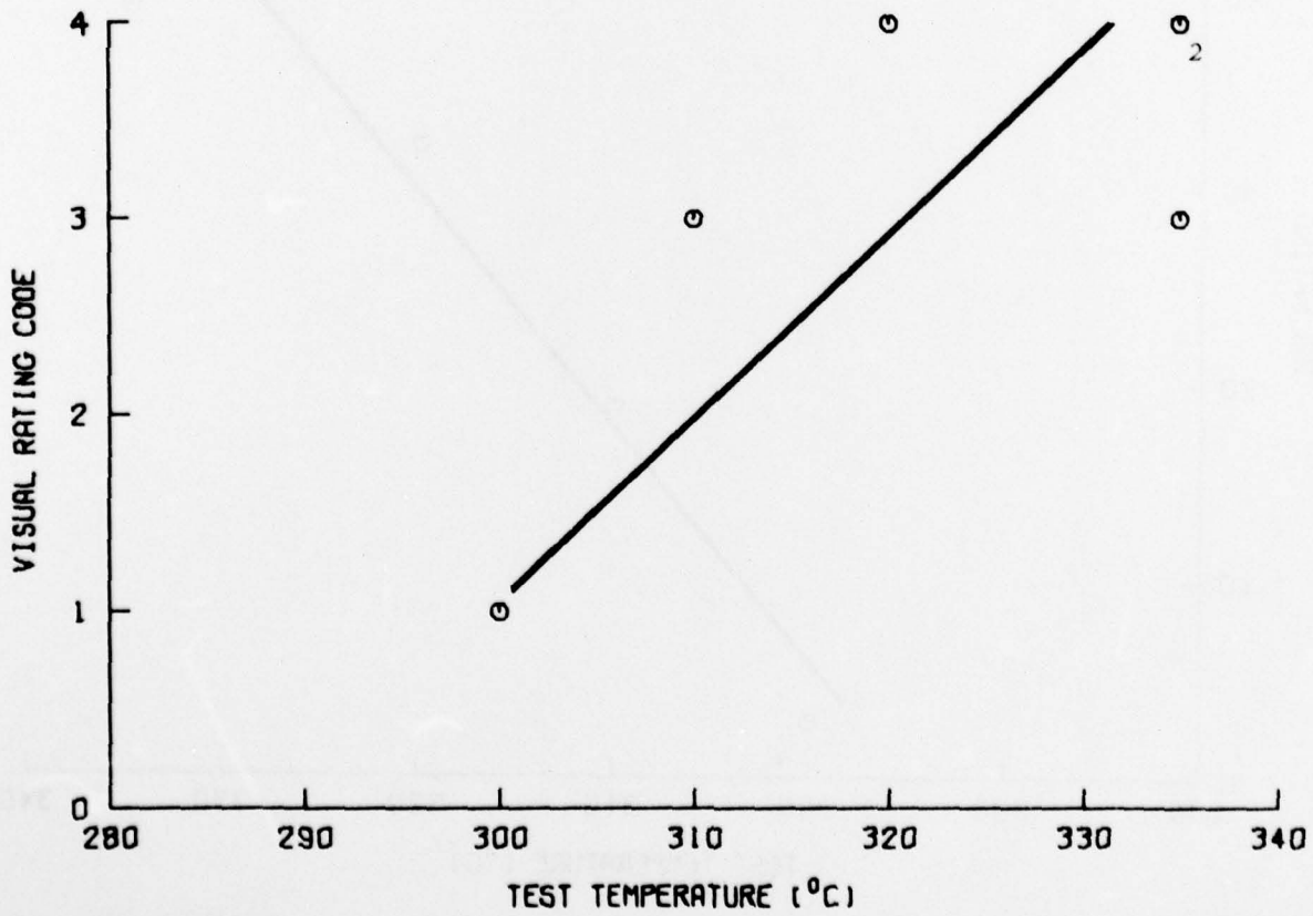
FIGURE 12. SFQLA JFTOT DATA FOR BATCH 79 - VISUAL RATINGS
