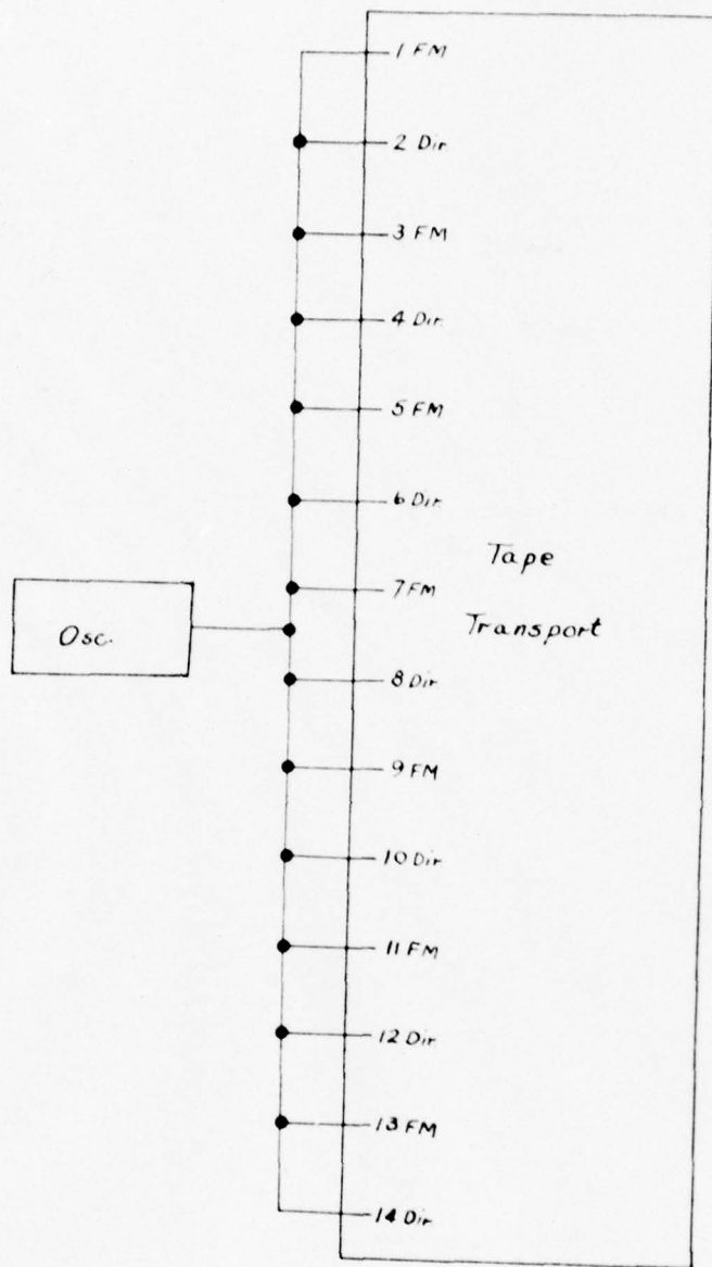
FIGURE 4b Instrumentation Block Diagram for Tape Recorder Calibration
