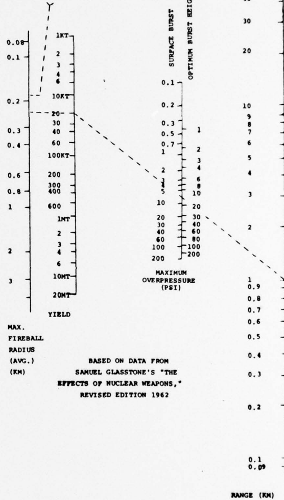
Figure 1. Nomogram for Overpressure and Fireball Radius
