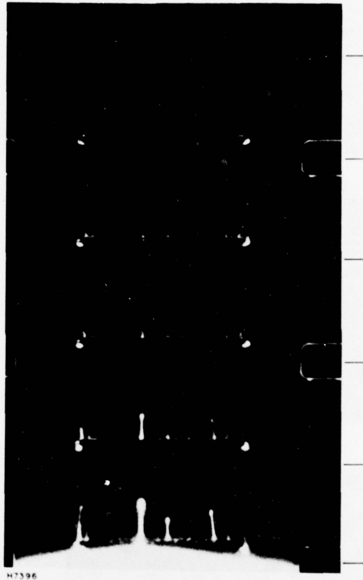
Figure 13 Streamer Growth
