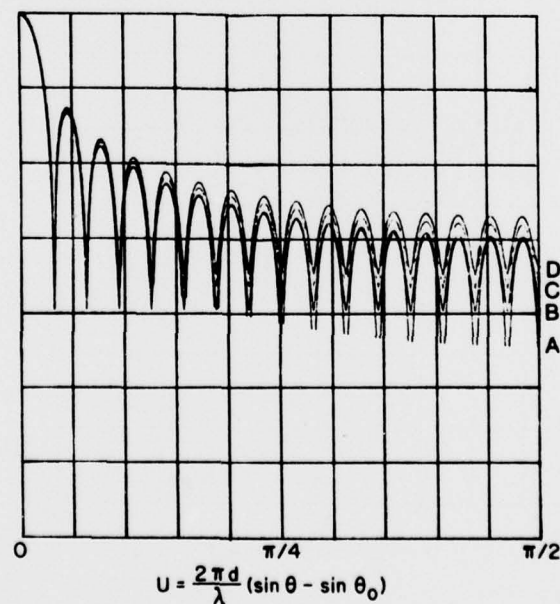
Figure 1. Standard Deviation of Phase Errors, \sigma_\phi = 0 Radians, Probability of Element Failure = 0
