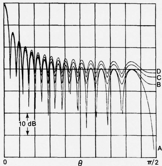
Figure 4. Polar Look Angle = 0 Radians, Azimuthal Look Angle = 0 Radians, Azimuthal Arrival Angle = 0 Radians, and Polar Slice \theta = 0.5\pi Radians
