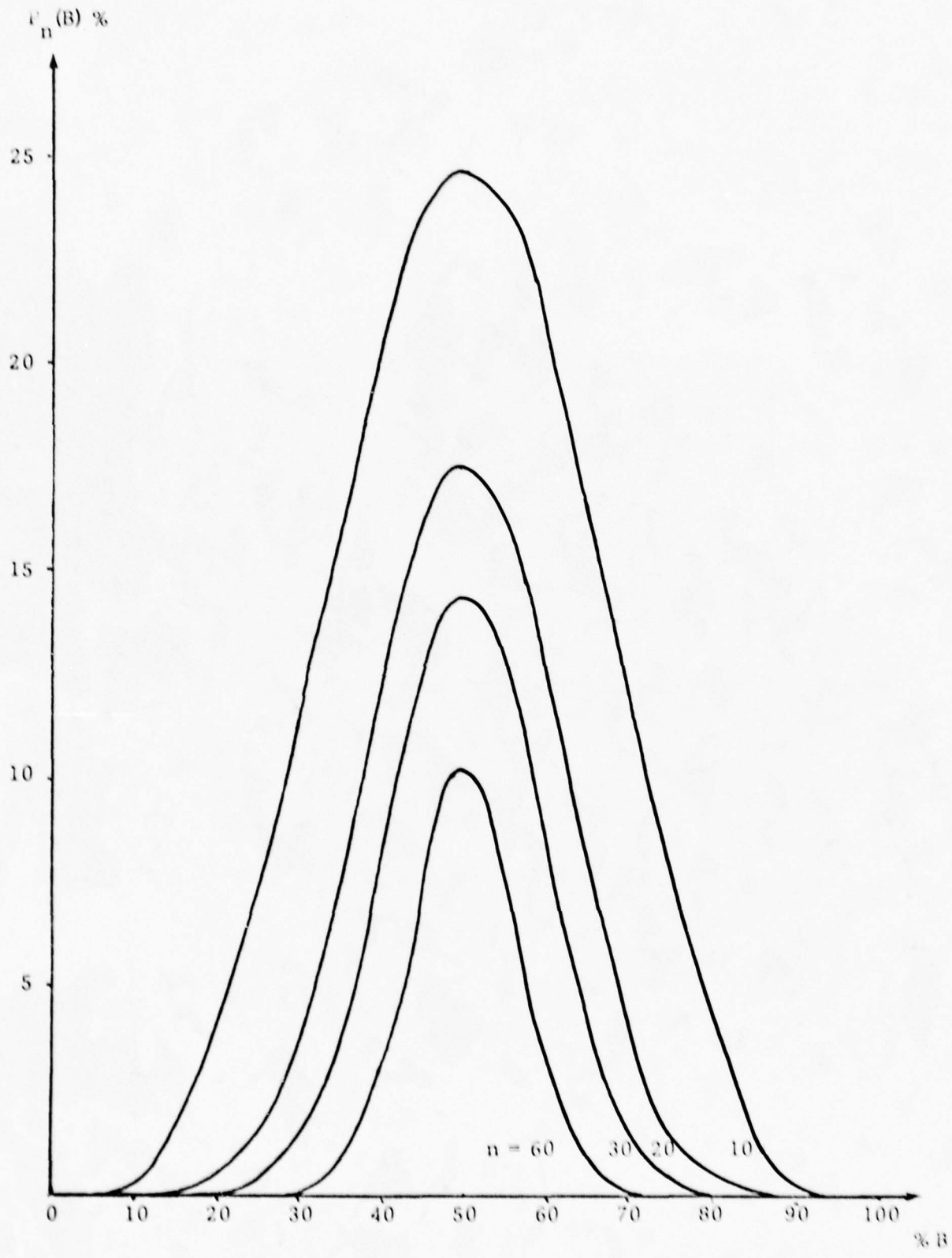
Fig. 18 Curves showing P_n(B) , the probability of B bits out of n bits matching by chance, as a function of B for various values of n .
