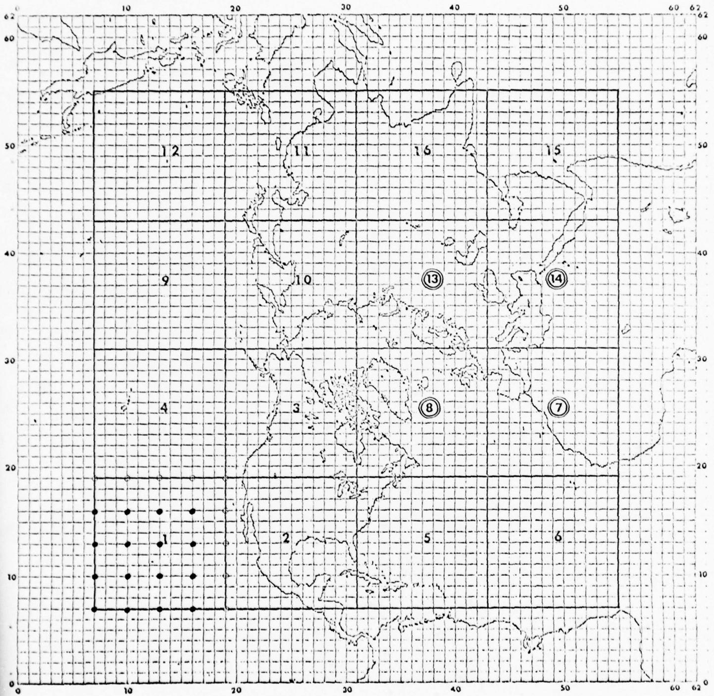
Fig. 17 Greater-Mediterranean Focus for the SV Component Fields. Extractions are made only for the circled-number modules. A double circle indicates fine resolution. A double bar under the number indicates medium resolution. And a single bar under the number indicates coarse resolution for that module.
