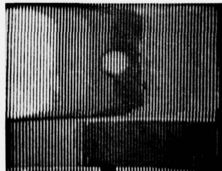
1/64-IN.-DIA HOLE SENSITIVITY 5° C
