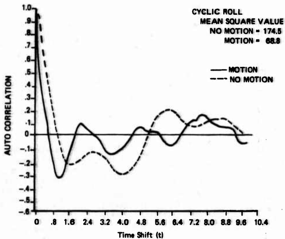
Figure 2-2. Shifts in operator control behavior
