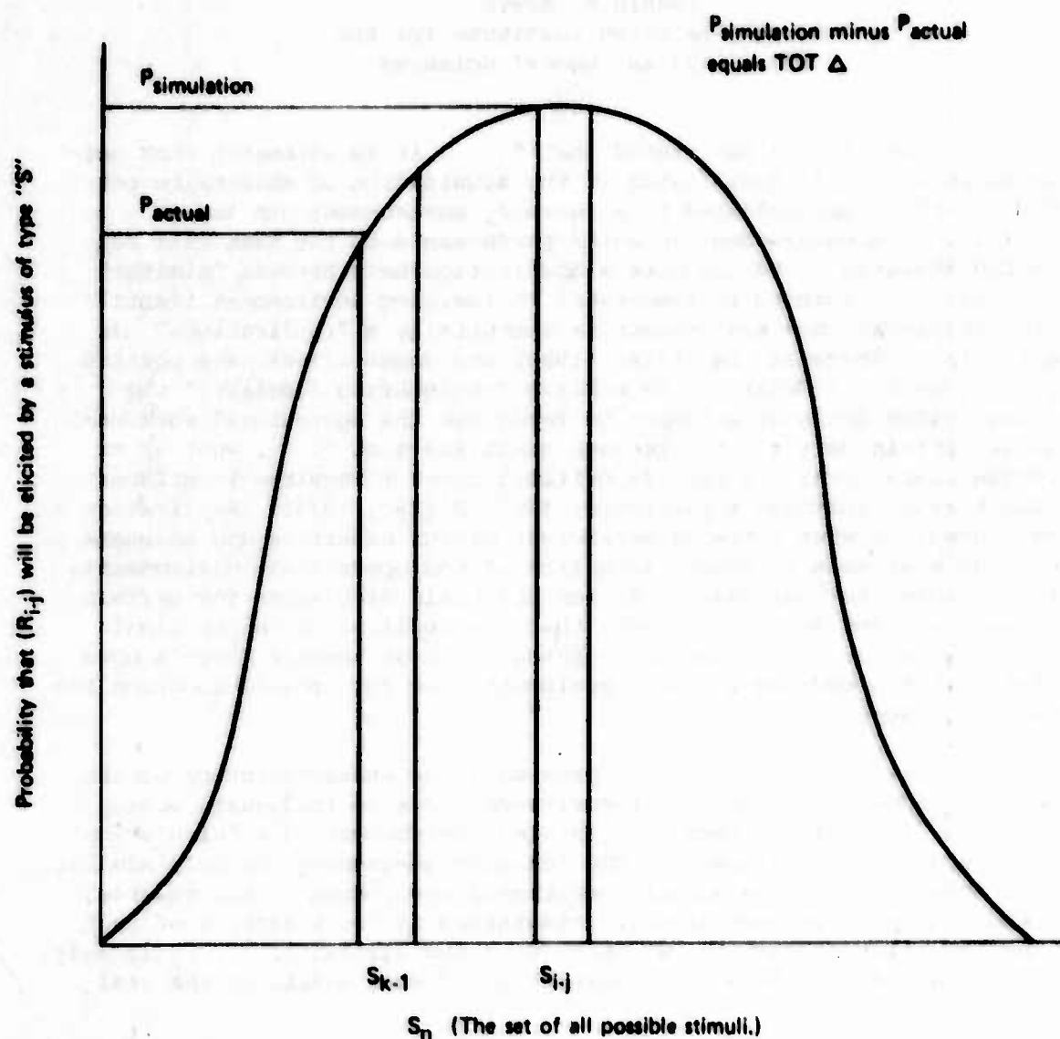
Figure 4-1. Generalization gradient for ( S_{i-j} ).
