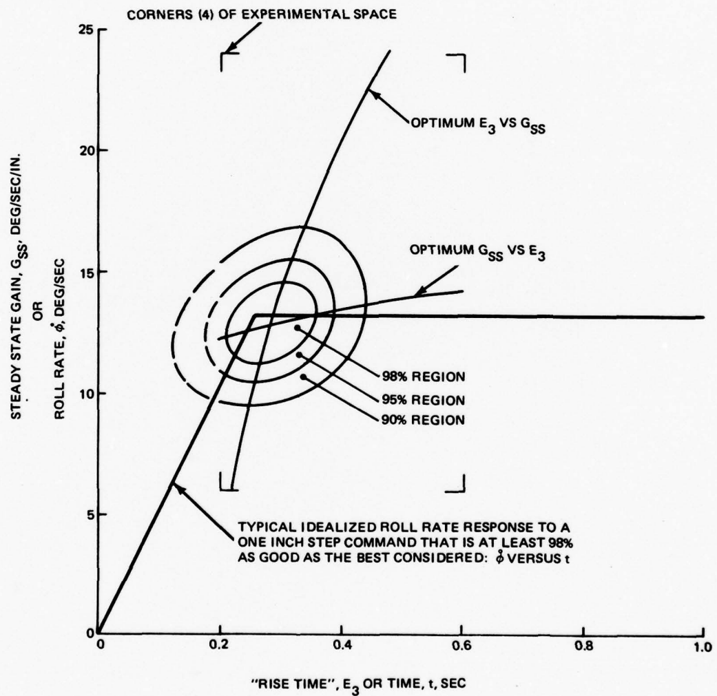
Fig. 12 Most Preferred Regions for the "Knee" of the Idealized Roll Rate Step Response
