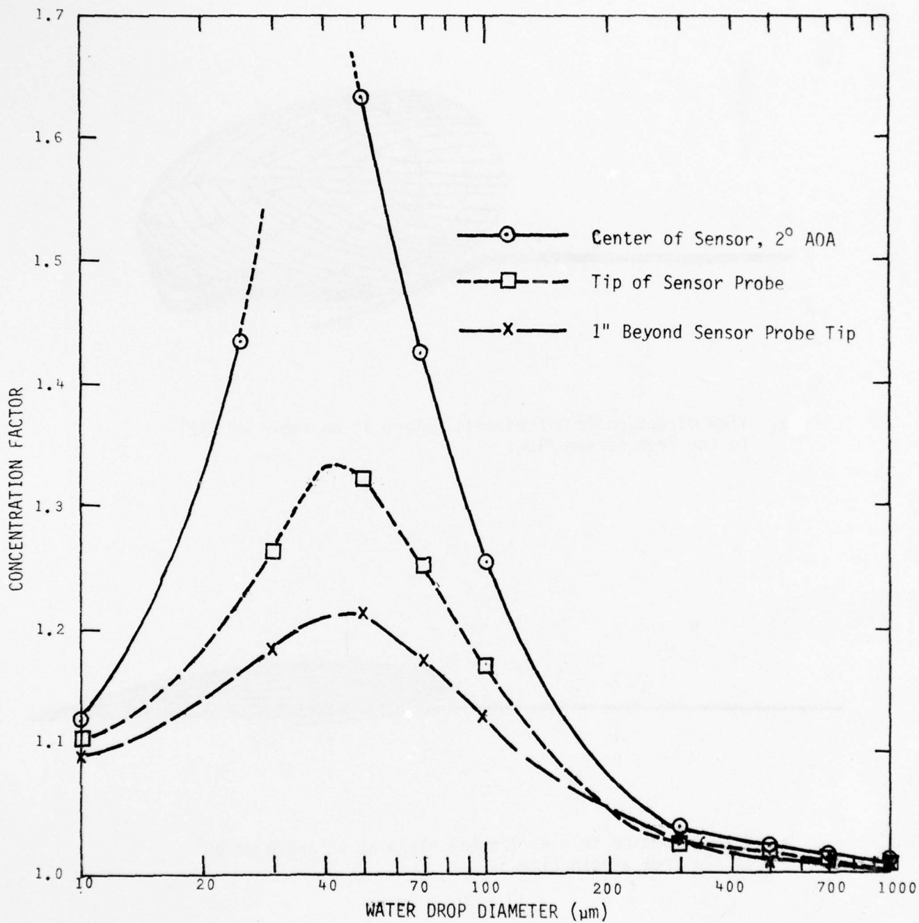
Figure 8. Concentration factor vs. water drop diameter for 2° angle-of-attack at the sensor probe center, and at two increased distances from the wing tip surface along the probe axis, both for 4° angle-of-attack. All for mounting site no. 1.
