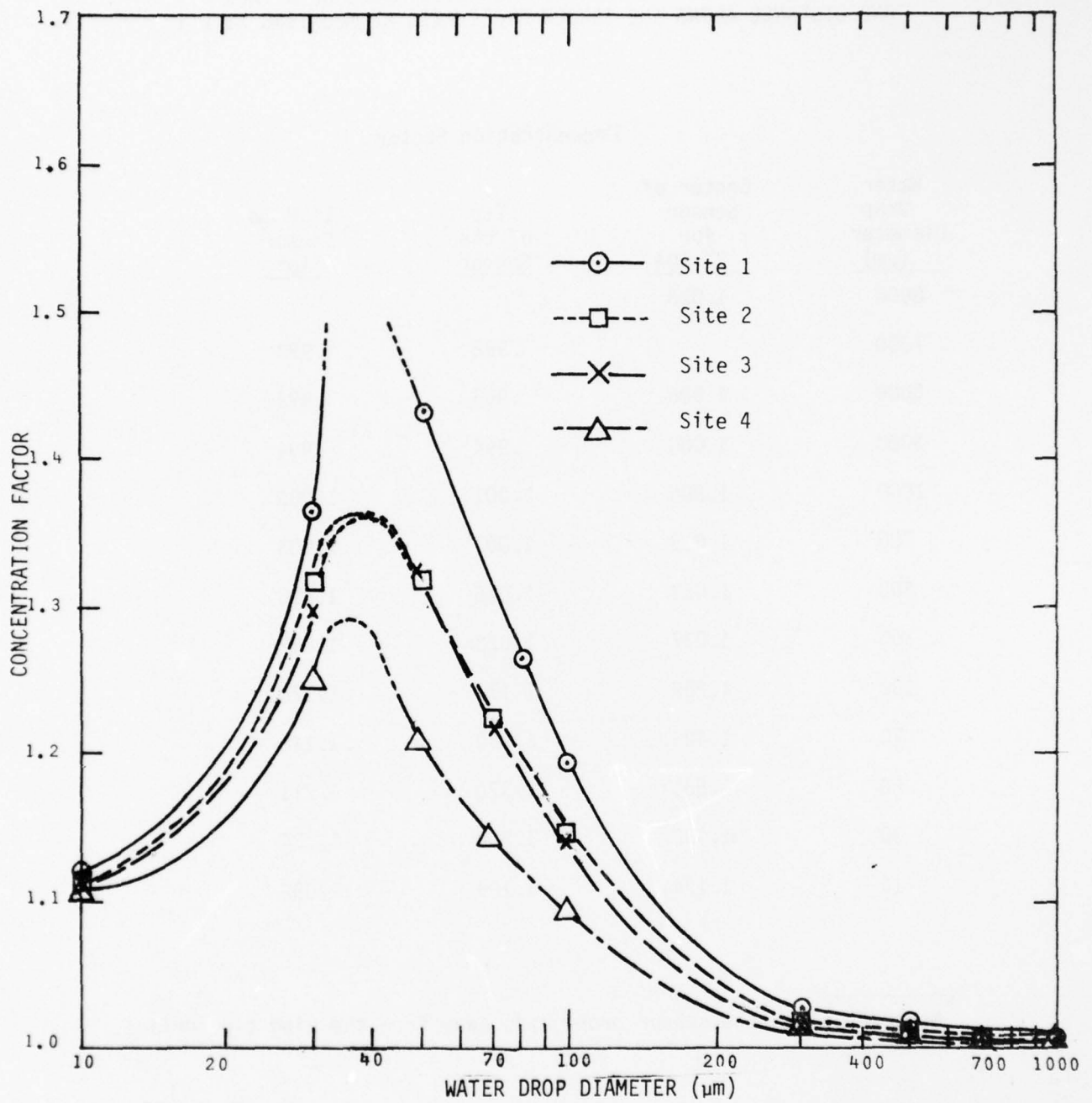
Figure 7. Concentration factor vs. water drop diameter at the sensor probe centers at the four proposed mounting sites. All for 4° angle-of-attack.
