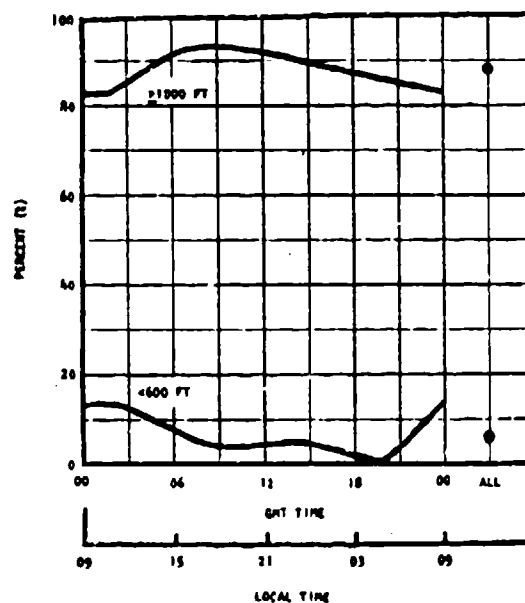
Figure D-9b - Ceiling Height - Diurnal Variation
