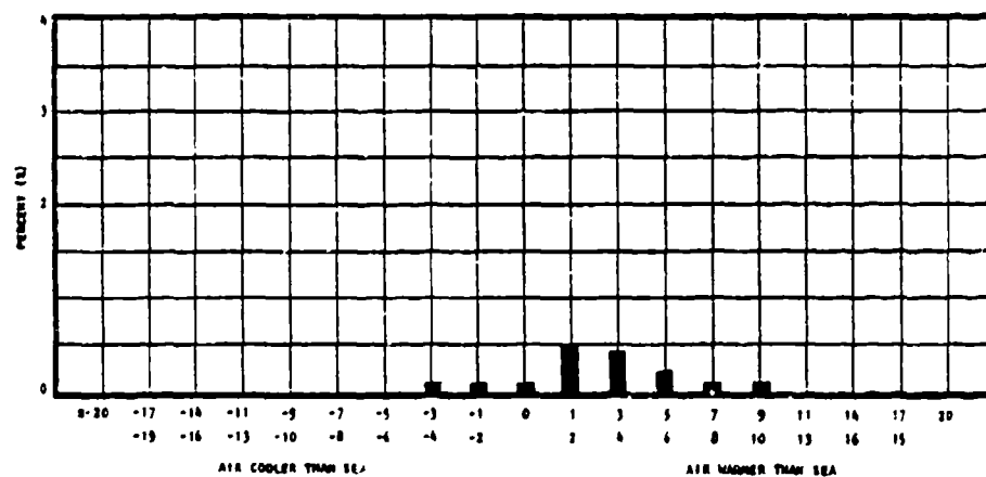
Figure E-10b - Fog versus Air - Sea Temperature Difference
