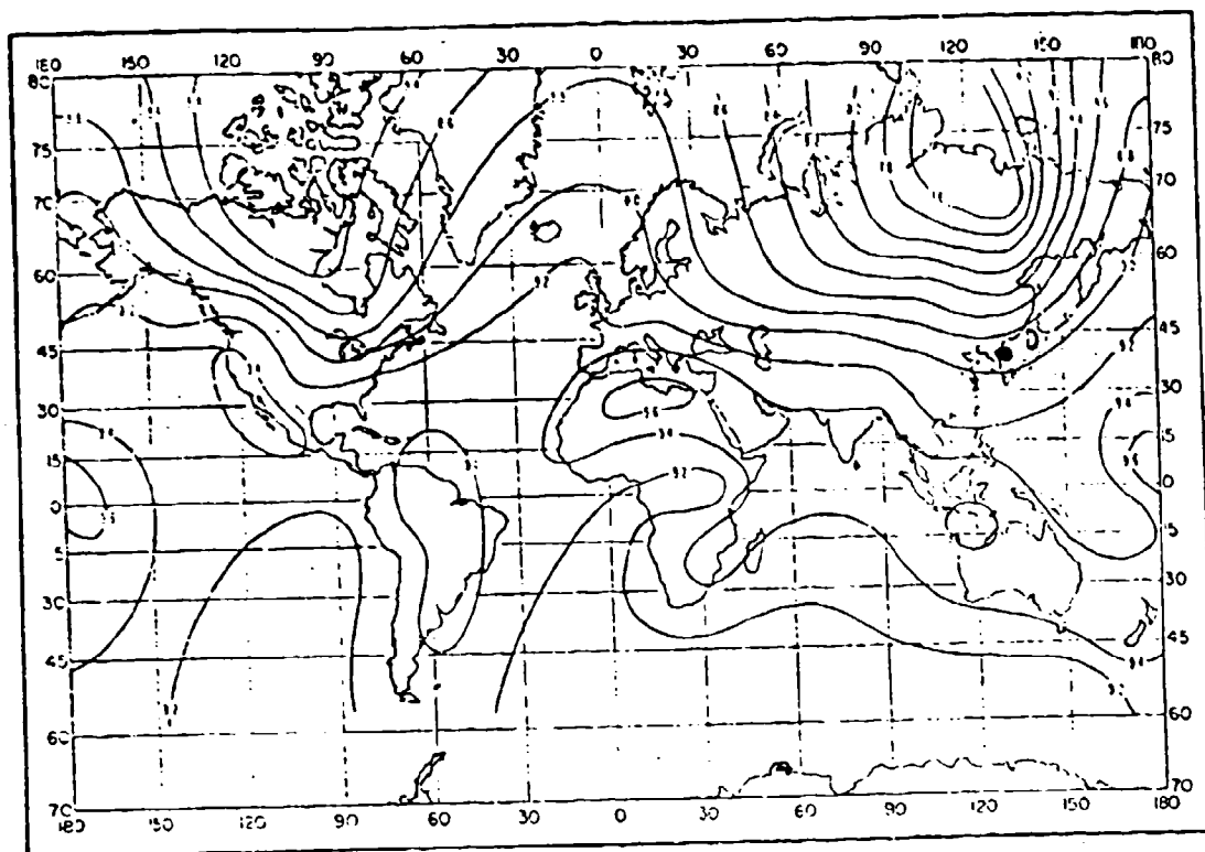
Dry-term tropospheric scale height in km, H_1 : November.
