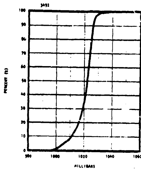
Figure D-8a - Sea Level Pressure - Cumulative Distribution
