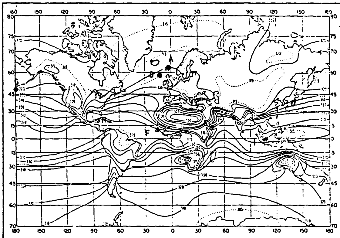
Annual mean of sea-level refractivity, \bar{N}_0 .
