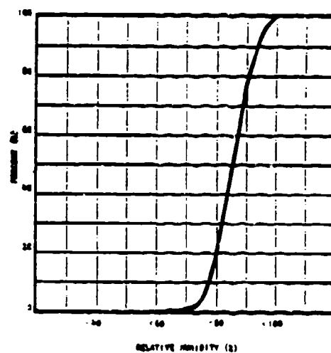
Figure F-6g - Relative Humidity - Cumulative Distribution
