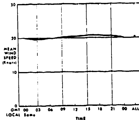
Figure A-2d - Wind Speed - Diurnal Variation
