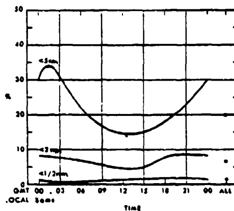
Figure A-3b - Visibility - Diurnal Variation
