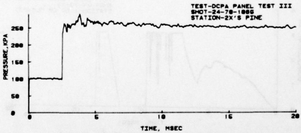
Figure 8. Pressure-time loading records for 2x's placed flat
