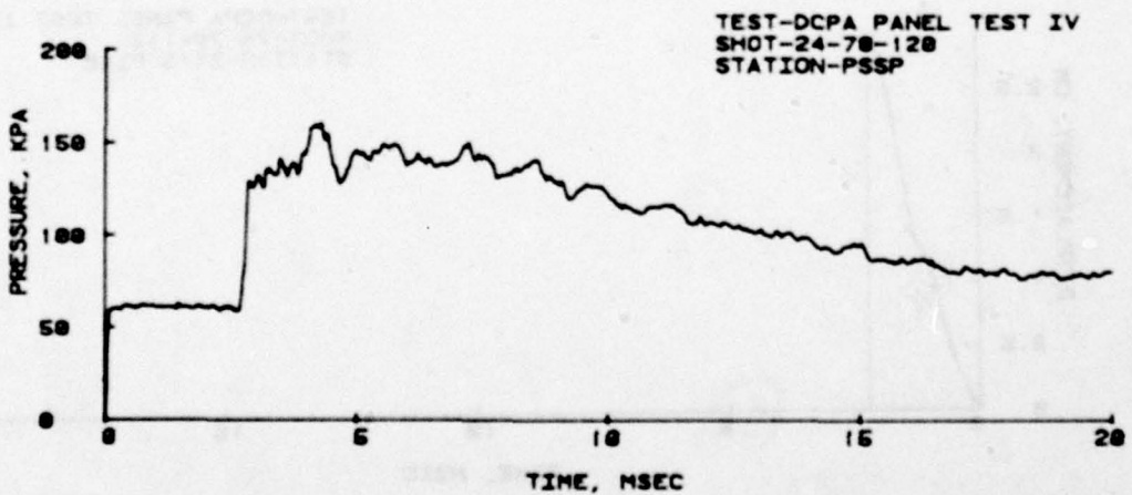
Figure 10. Pressure-time loading records for PSSP closures with plywood skins not glued
