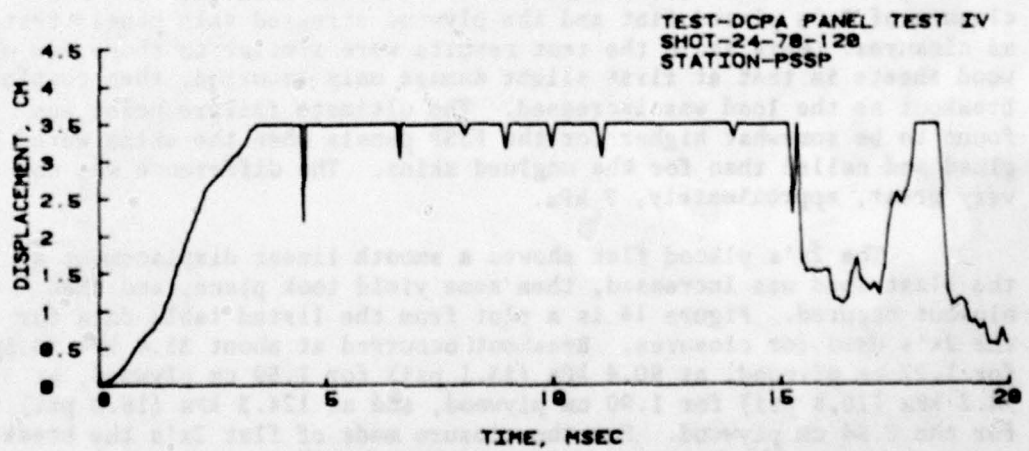
Figure 11. Displacement-time records for PSSP closures with plywood skins not glued
