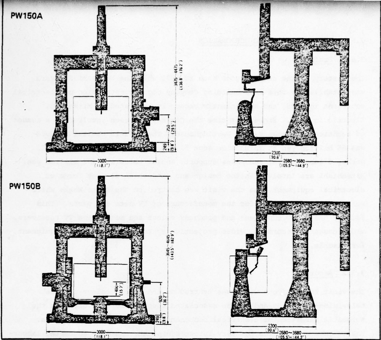
FIG. 3.5.1 SHIN MEIWA ROBOT WELDER PW 150 SERIES
