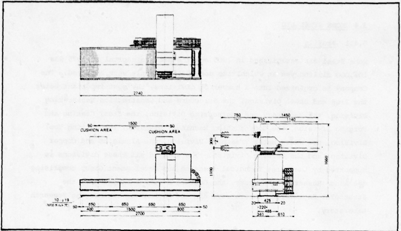
FIG. 3.3.6 KAWASAKI-UNIMATE MODEL 3330
