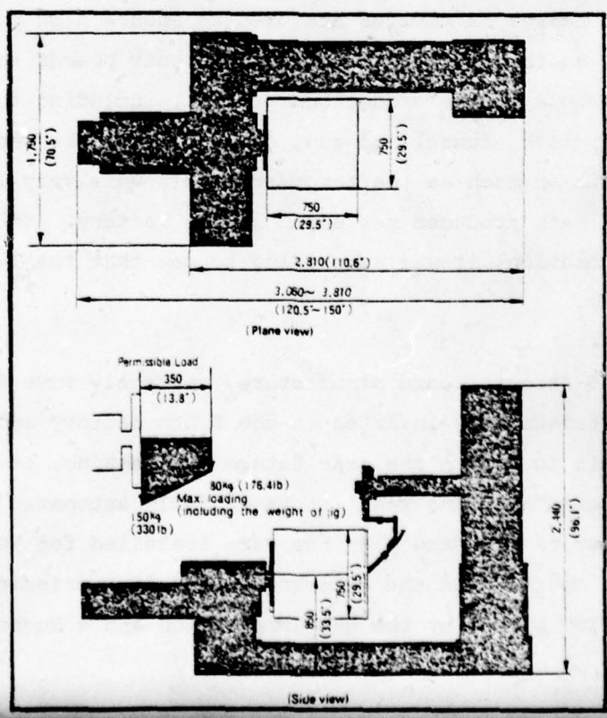
FIG. 3.5.1 SHIN MEIWA ROBOT WELDER PW 150 SERIES
