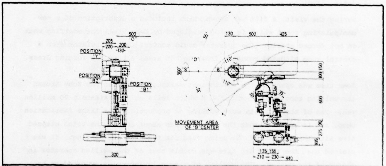
FIG. 3.3.7 KAWASAKI-UNIMATE MODEL 6060
