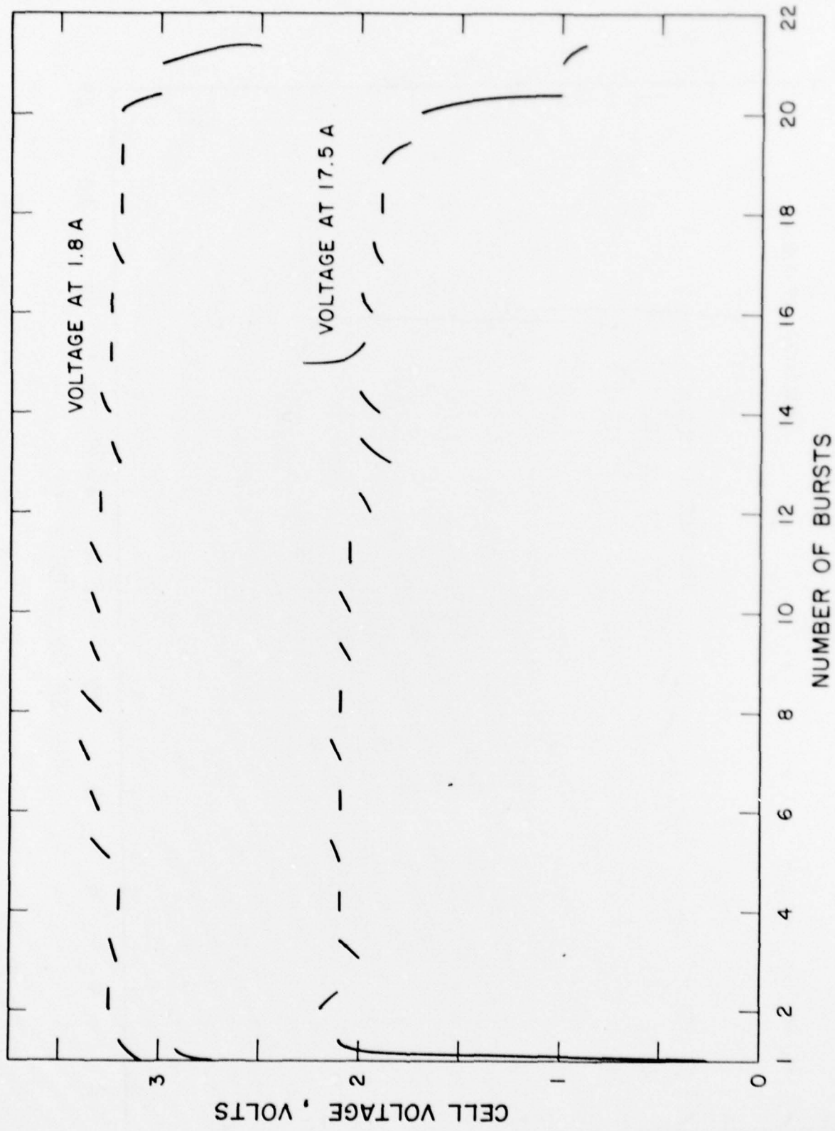
Fig. 28 Performance of two D cells with cathode additive 4 on GLLD test
