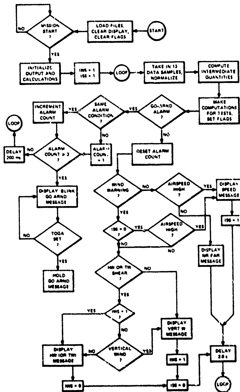
FIGURE C-2 DISPLAY LOGIC
