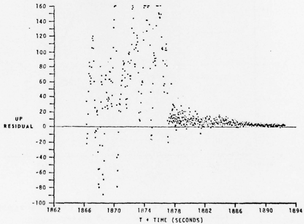
FIGURE 16 KMR POINT BY POINT TRAJECTORY MINUS WTR REENTRY TRAJECTORY 196
