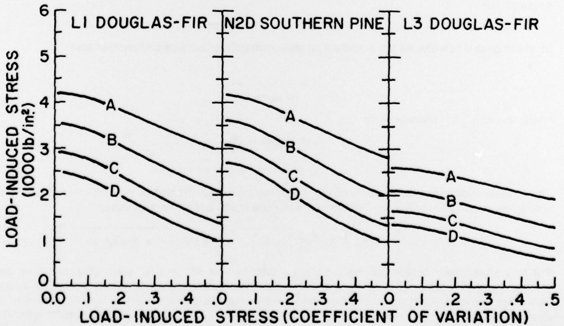
Figure 1-2.—Comparative reliability plots for two lamination beams at four safety levels (A-D), for three grades of material quality (Safety index values as for fig. 1-1).
