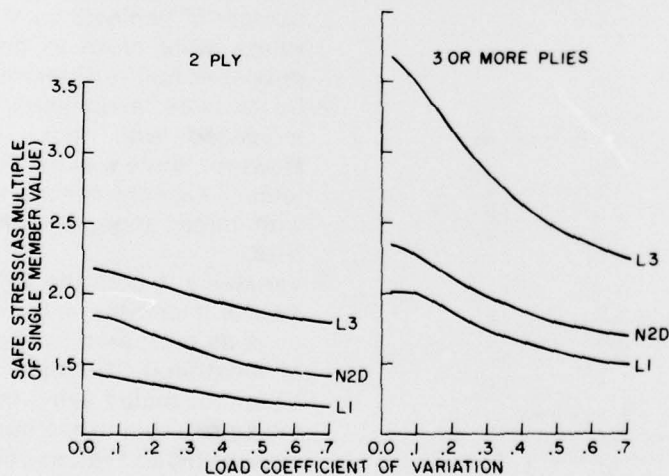
Figure 10.—Laminating effect at a safety index \beta = 3.0
