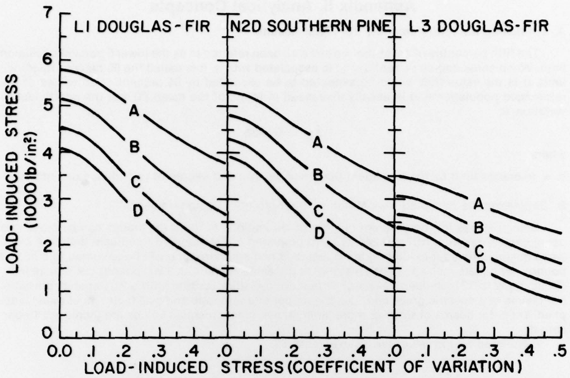
Figure 1-5.—Comparative reliability plots for five-lamination beams at four safety levels (A-D), for three grades of material quality. (Safety index values as for fig. 1-1). (M 146 713)
