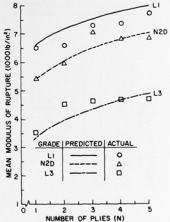
Figure 4.—Comparison of mean modulus of rupture values with those predicted by equations (3) and (4). (M 146 717)
