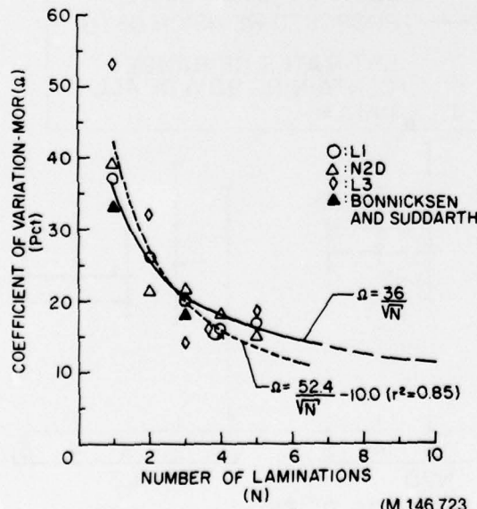
Figure 3.—Decrease in variability in modulus of rupture with more laminations. (M 146 723)
