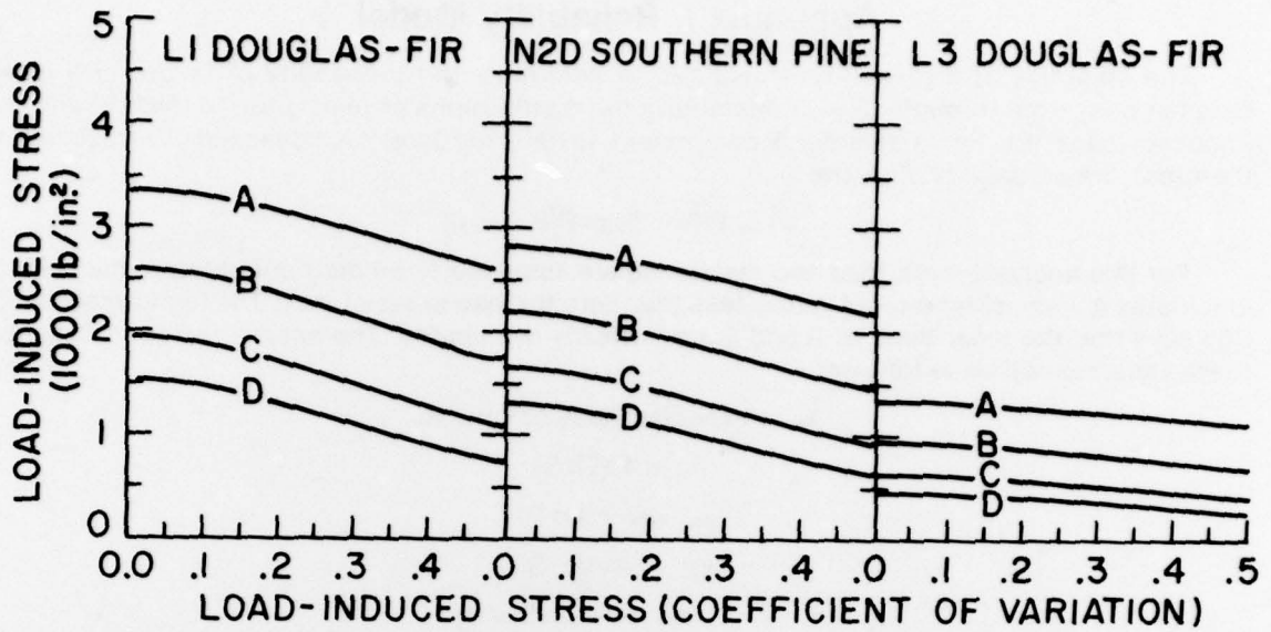
Figure 1-1.—Comparative reliability plots for single member beams at four safety levels (A-D) for three grades of material quality. Loads were applied parallel to the wide face. A Safety index \beta = 1.645 - reliability level = 0.9500 B Safety index \beta = 2.330 - reliability level = 0.9900 C Safety index \beta = 3.100 - reliability level = 0.9990 D Safety index \beta = 3.750 - reliability level = 0.9999
