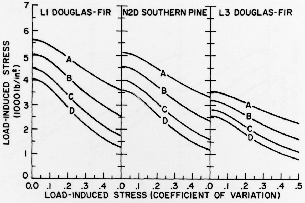
Figure I-4.—Comparative reliability plots for four-lamination beams at four safety levels (A-D), for three grades of material quality. (Safety index values as for fig. I-1). (M 146 711)
