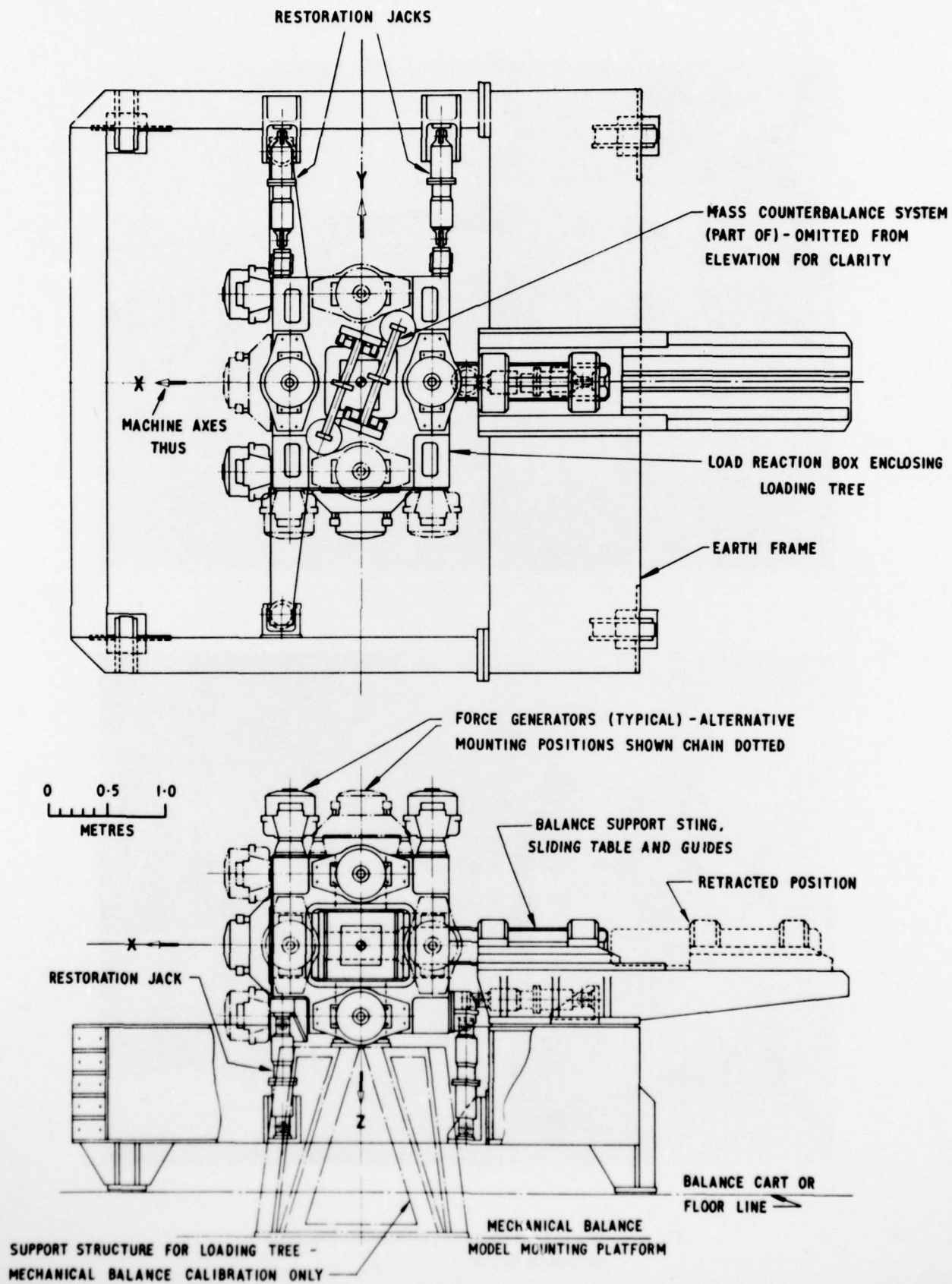
Fig 7 5m tunnel balance calibration machine - GA
