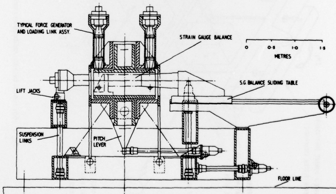
Fig 5 1972 design study proposed arrangement of balance calibration machine
