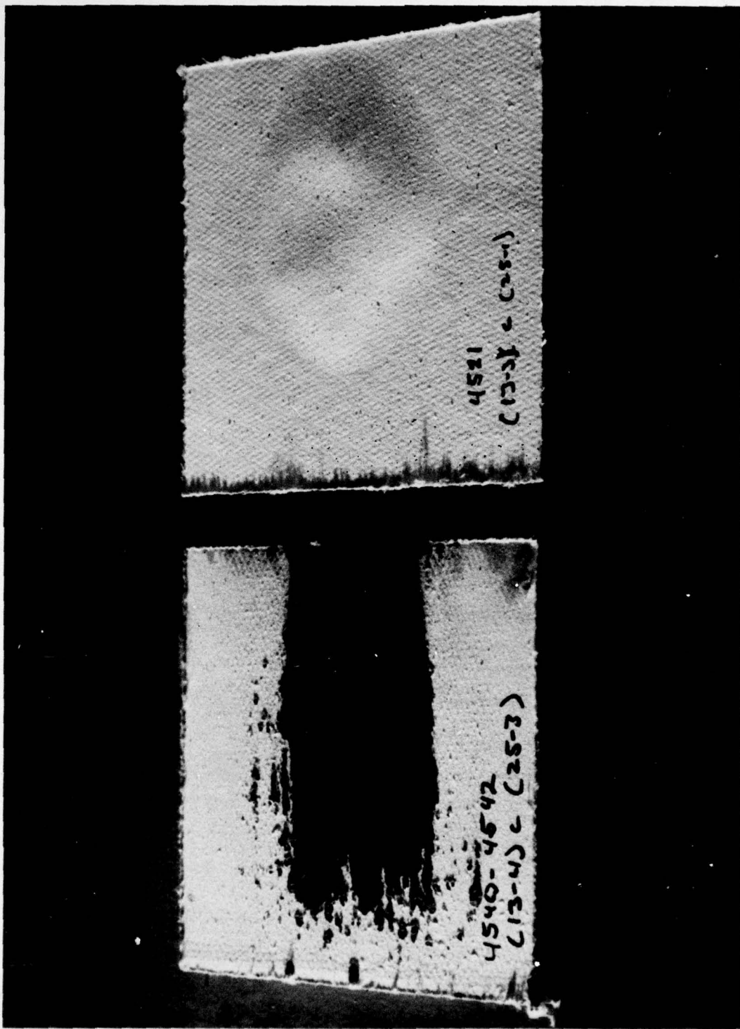
Figure 58. System 13 - one vs three flashes at 25 cal/cm 2 .
