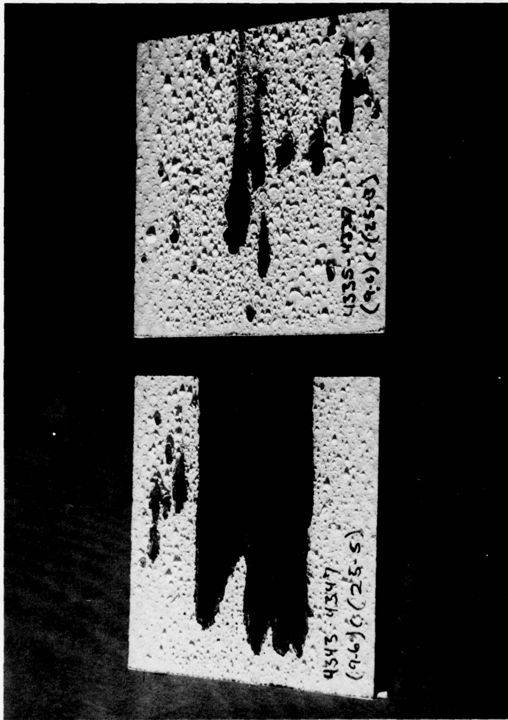
Figure 24. System 9 - progressive degradation from three to five flashes at 25 cal/cm 2 .
