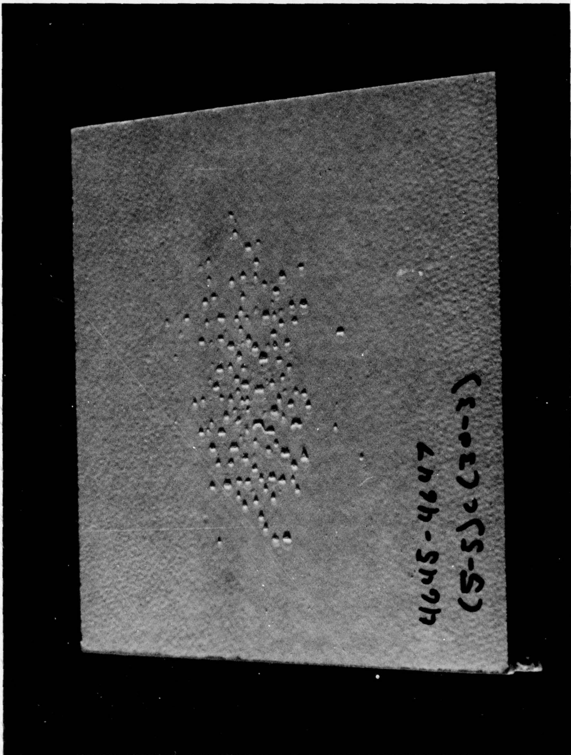
Figure 12. System 4 - paint blistering at 50 \text{ cal/cm}^2 .
