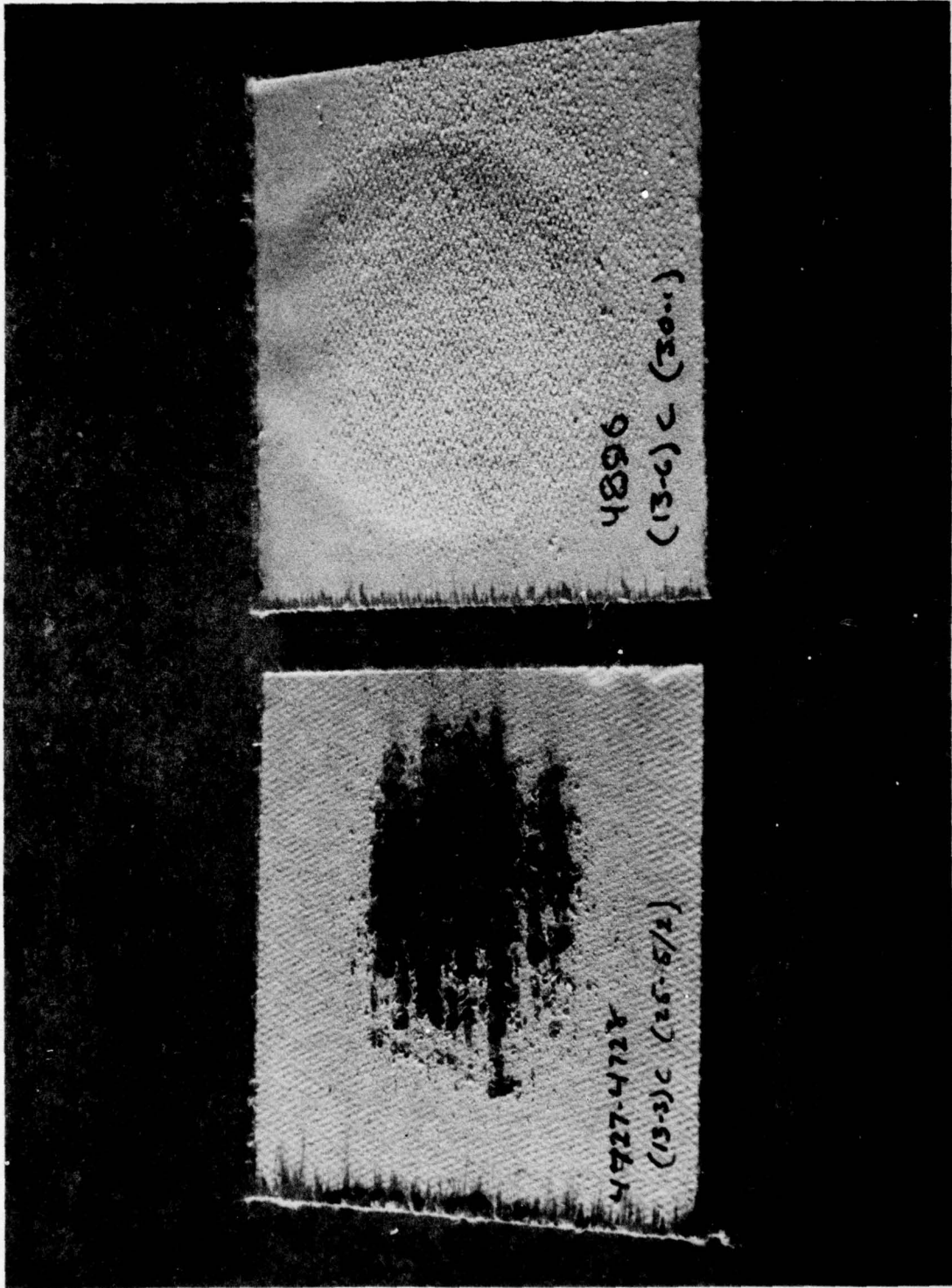
Figure 57. System 13 - 3- vs 6-ply damage.
