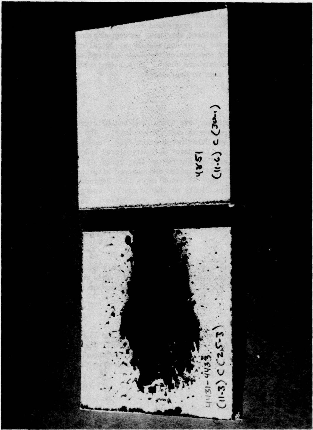
Figure 31. System 11 - 6- vs 3-ply specimen damage.
