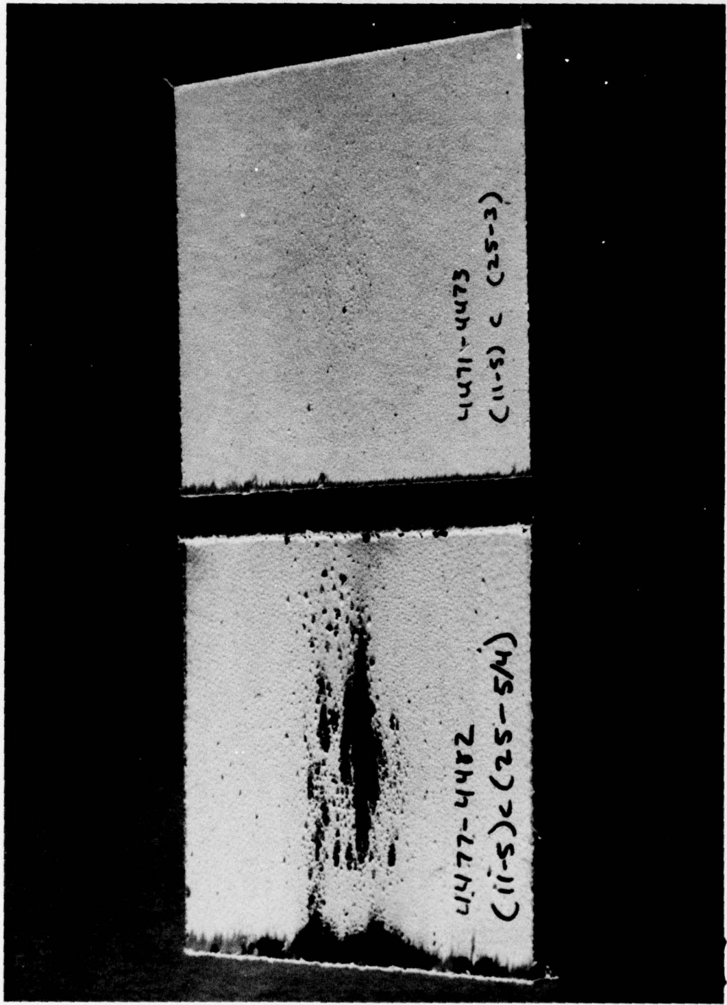
Figure 29. System 11 - three vs four flashes at 25 cal/cm 2 .
