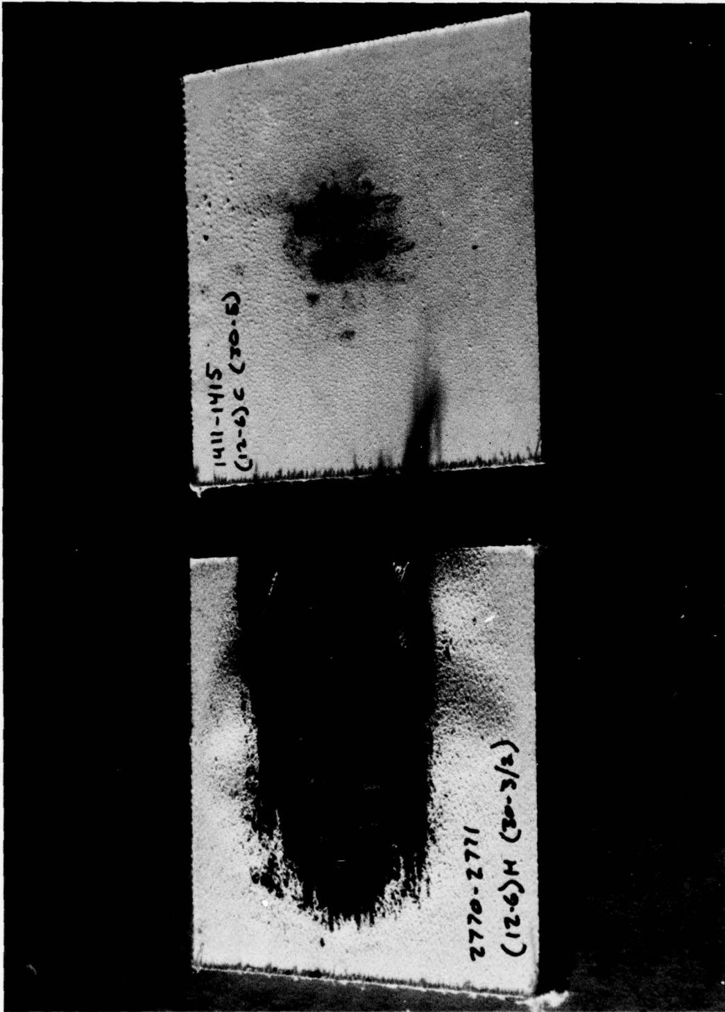
Figure 35. System 12 - humidity saturated vs dry specimen at 50 cal/cm 2 .
