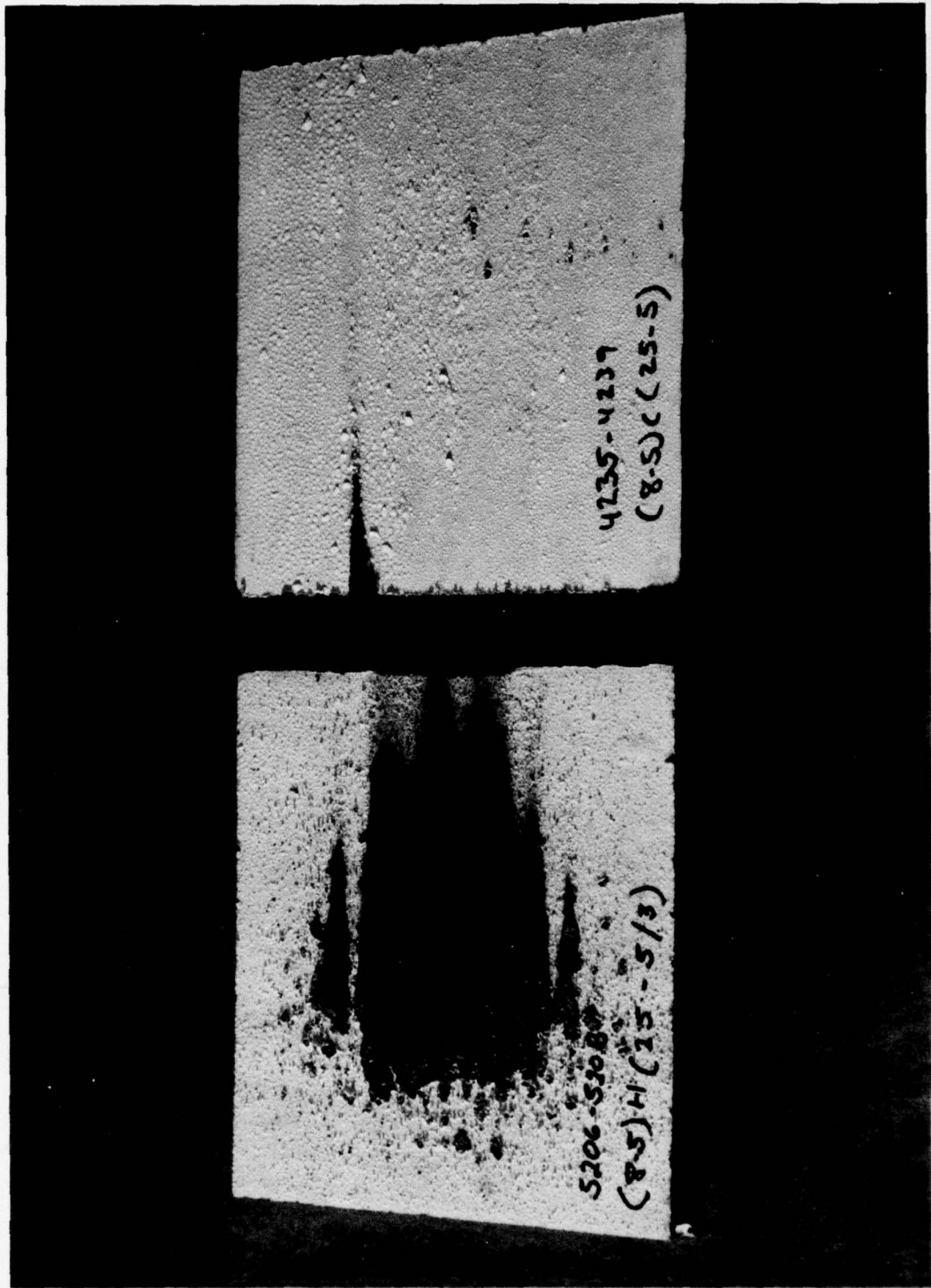
Figure 21. System 8 - humidity saturated vs dry specimen at 25 cal/cm 2 .
