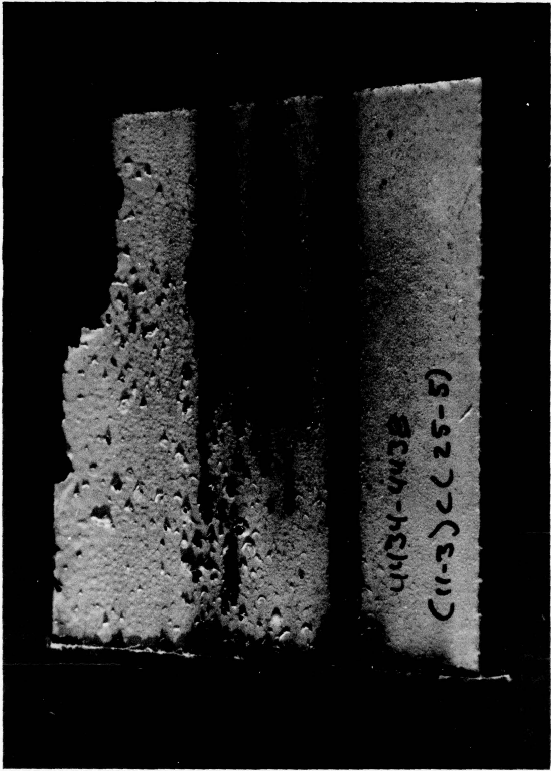
Figure 28. System II - specimen degradation at 25 \text{ cal/cm}^2 (five flashes).
