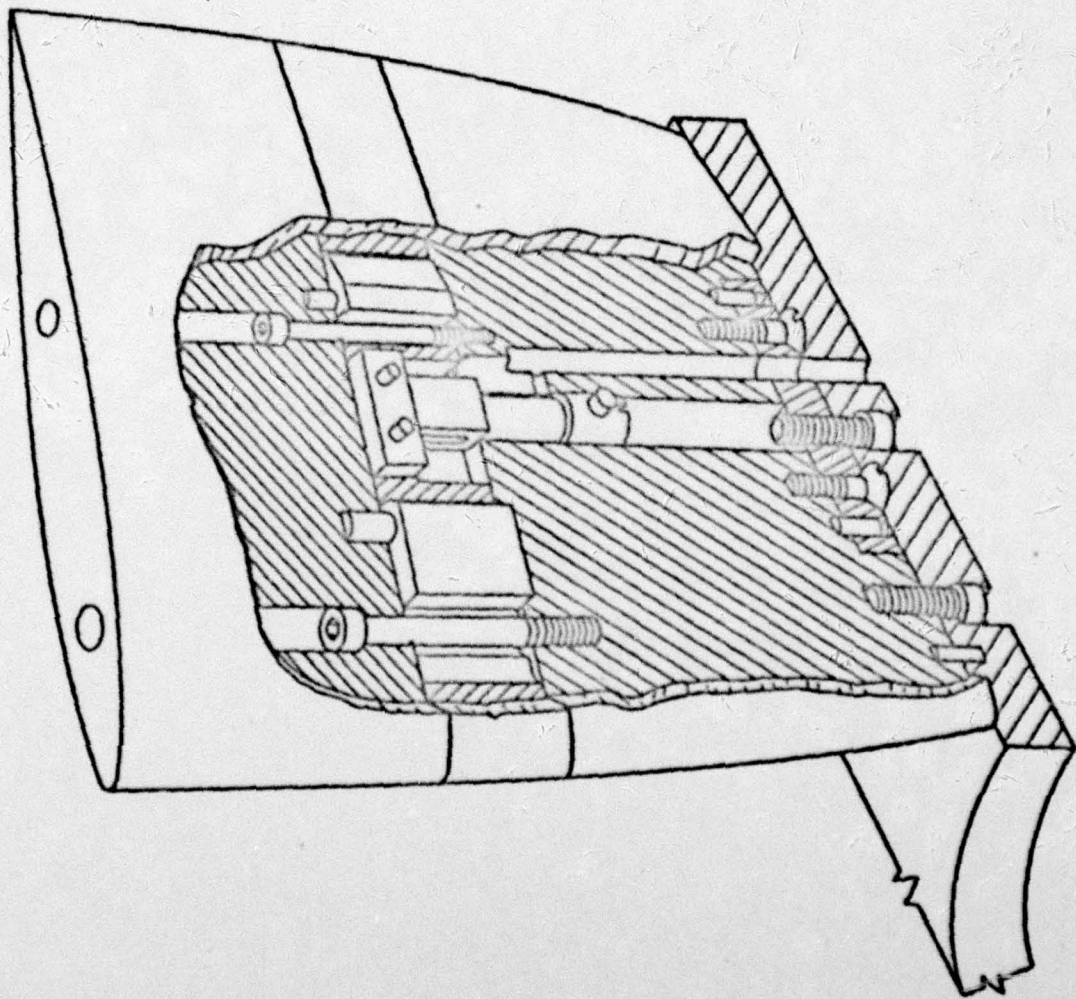
Figure 15. Schematic of Strain Gage Sensor Installation for ORL Axial Flow Research Fan Rotor Blade Section
