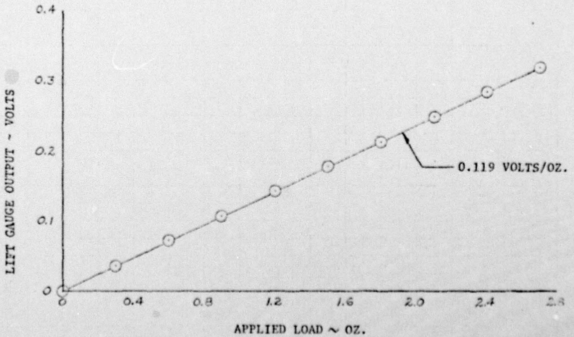
Figure 17. Results of Static Calibration of AFRF Instrumented Blade Sensor
