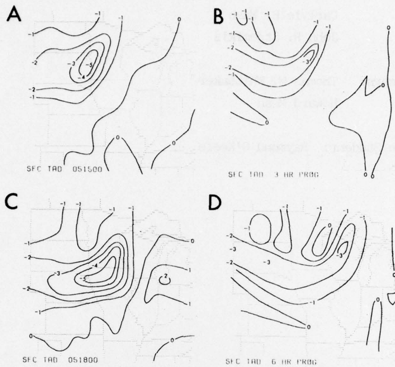
Figure 7. a. Observed temperature advection 1500 GMT 5 April 1979. b. 3 hour temperature advection forecast verifying at 1500 GMT. c. Observed temperature advection 1800 GMT 5 April 1979. d. 6 hour temperature advection forecast verifying at 1800 GMT.
