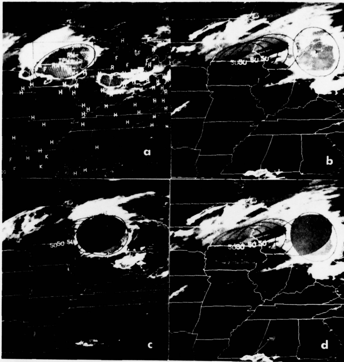
Figure 4. a. Surface weather data and an ellipse fit of the brightness area for 1400 GMT 17 June 1978. b. Sequence of ellipses generated from brightness patterns for 1300, 1400, 1500, 1600 and 2000 GMT. c. & d. Verification of linear regression extrapolation for 2 (c) and 4 (d) hours.
