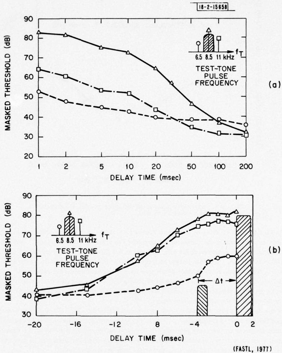
Fig. III-7. Nonsimultaneous masking of tone pulses by critical bandwidth noise masker bursts: (a) forward masking, (b) backward masking.
