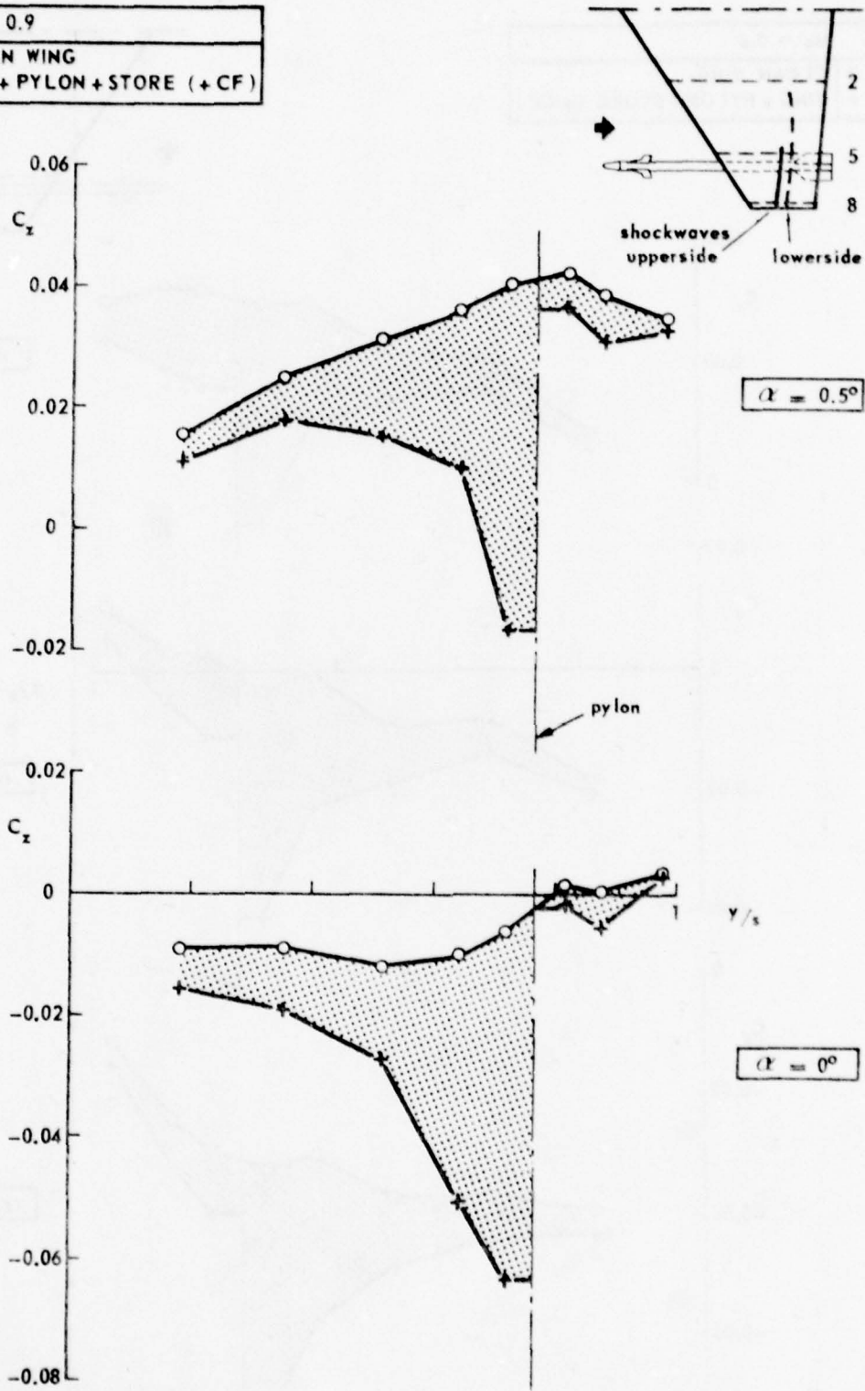
Fig. 2b Steady spanwise normal load distributions on the clean wing and on the wing with pylon and store at Ma = 0.9
