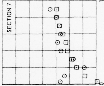
CONF. 31 (WING + PYLON + LAUNCHER + MISSILEBODY WITH AFT WINGS)
