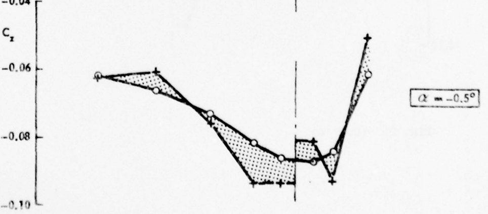
Fig. 2c Steady spanwise normal load distributions on the clean wing and on the wing with pylon and store at Ma = 1.35
