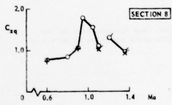
Fig. 4 Sectional quasi-steady normal load distribution on the clean wing and the wing with pylon and store versus Mach number
