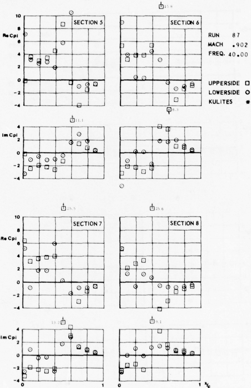
CONF. 31 (WING + PYLON + LAUNCHER + MISSILEBODY WITH AFT WINGS)
