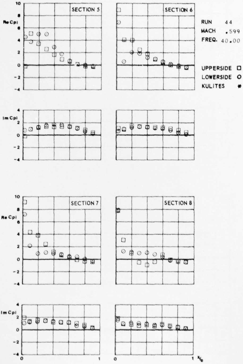
CONF. 301 (WING + PYLON + LAUNCHER + COMPLETE MISSILE)
