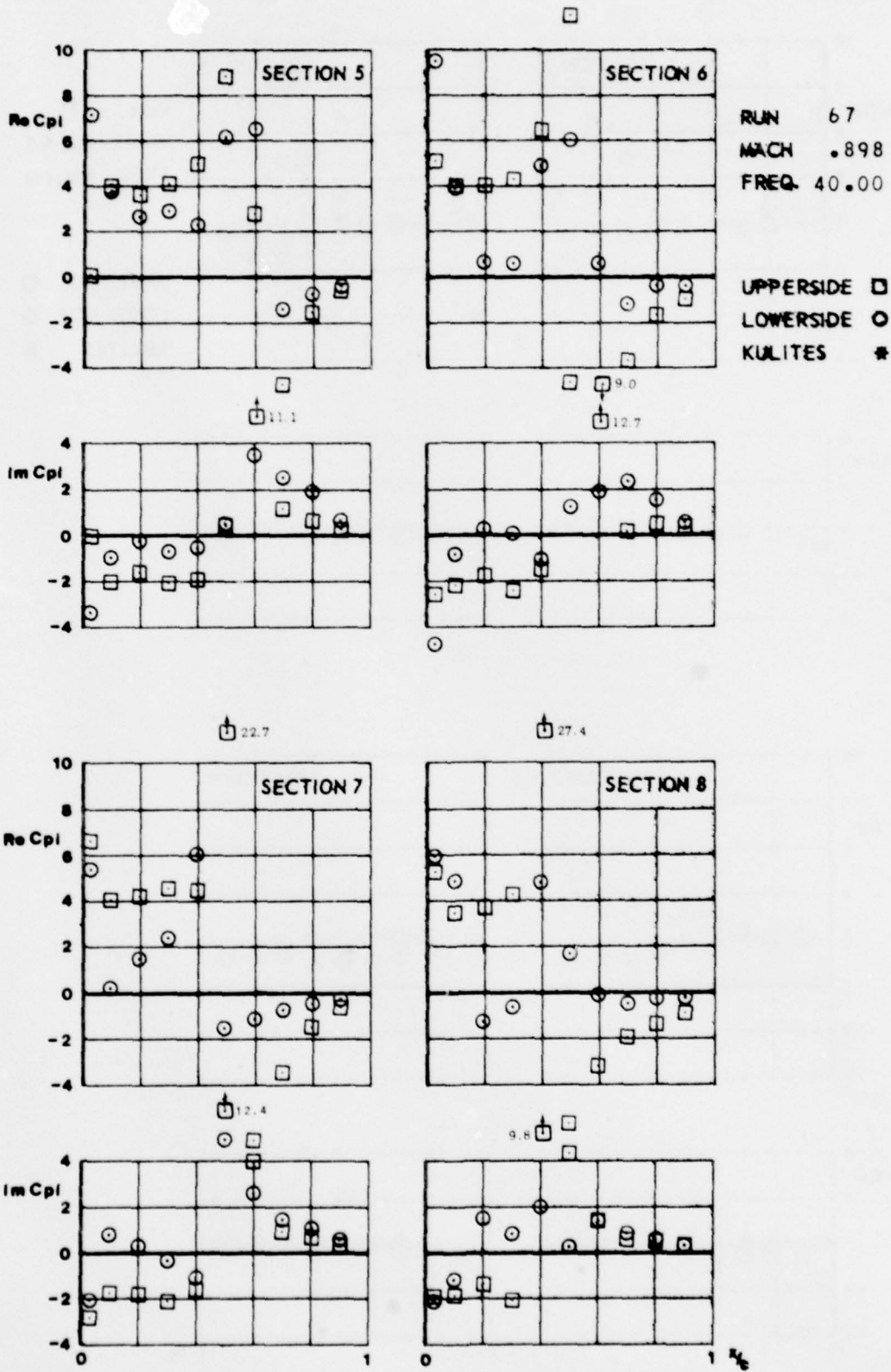
CONF. 20 (WING + PYLON + LAUNCHER)
