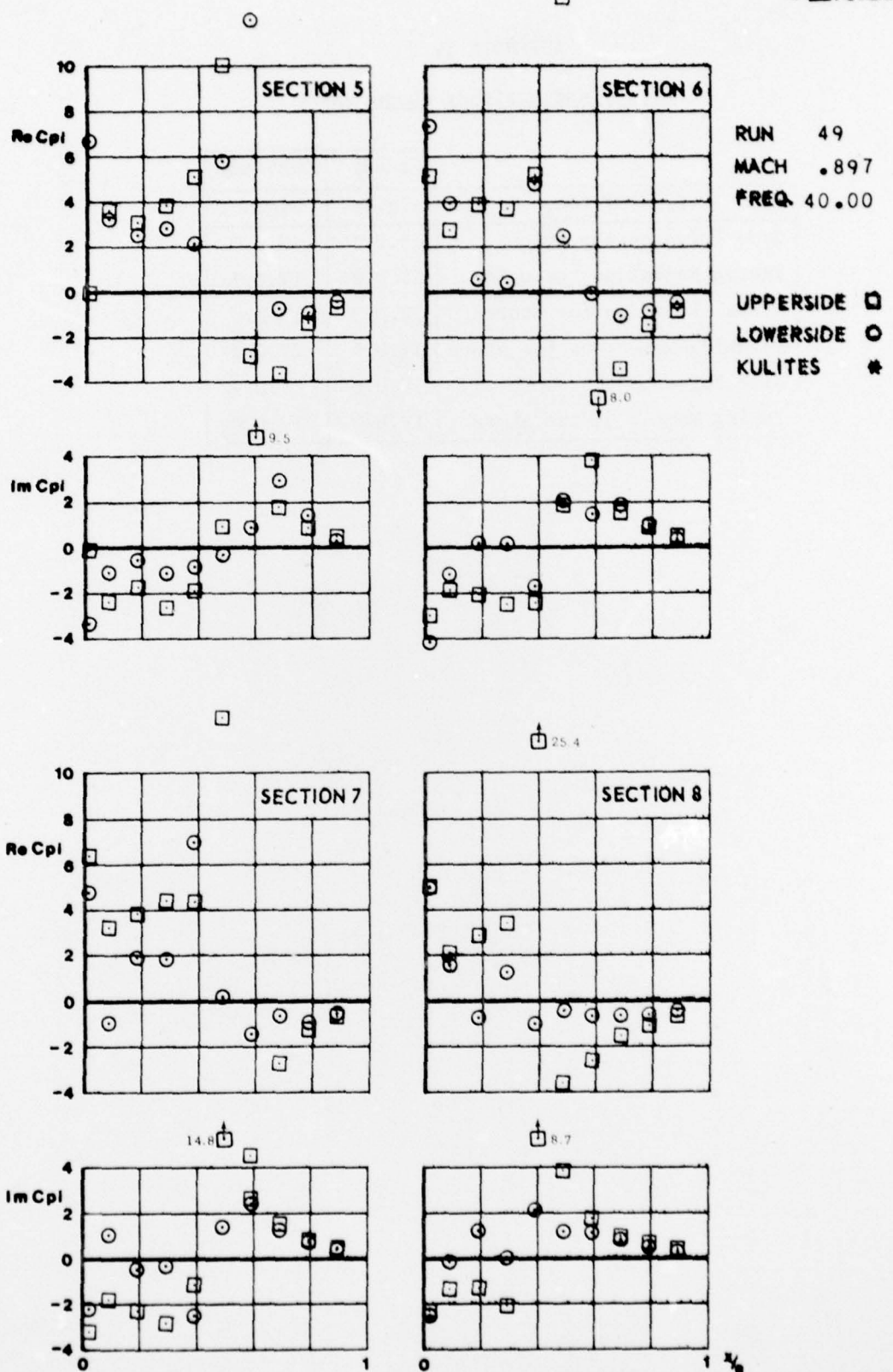
CONF. 301 (WING + PYLON + LAUNCHER + COMPLETE MISSILE)
