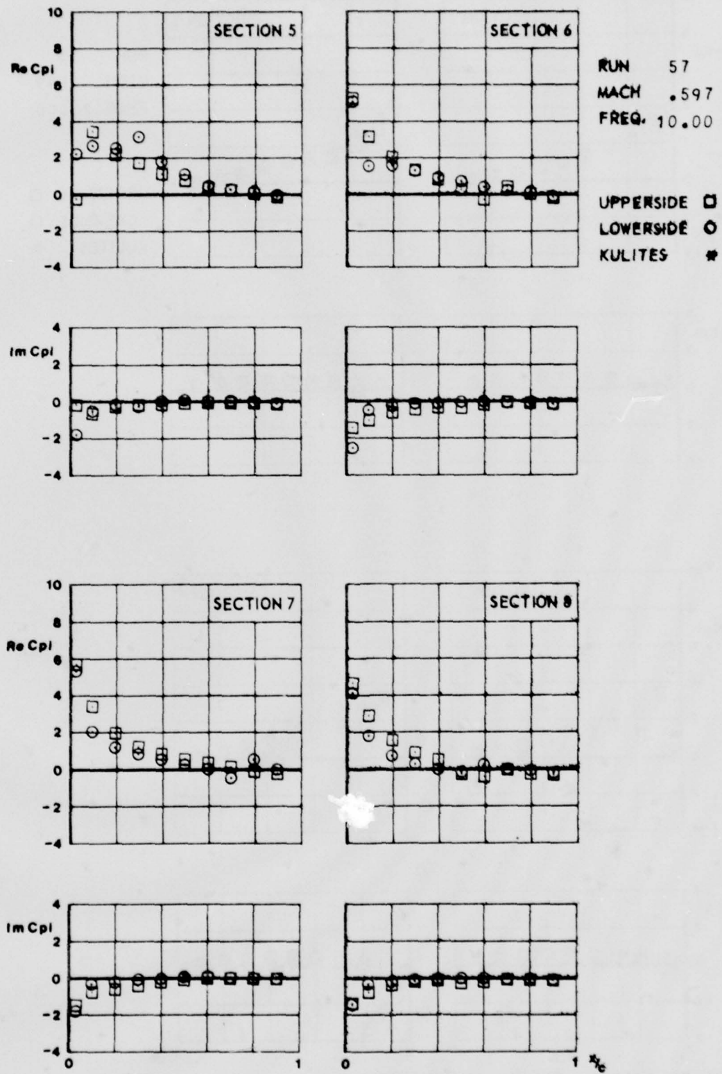
CONF. 20 (WING + PYLON + LAUNCHER)
