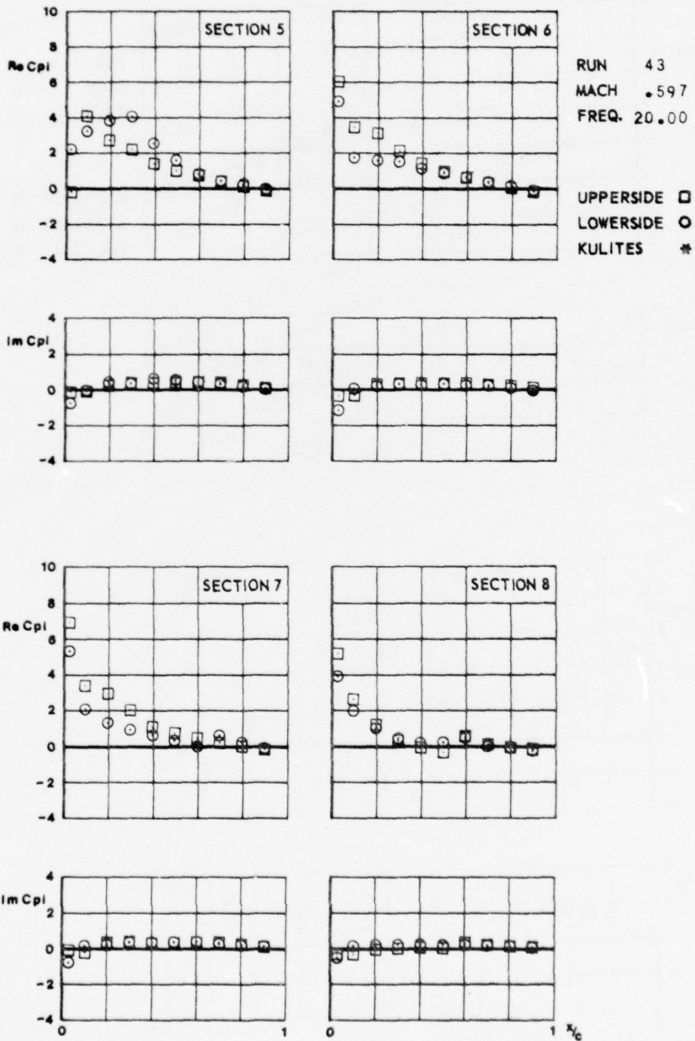
CONF. 301 (WING + PYLON + LAUNCHER + COMPLETE MISSILE)
