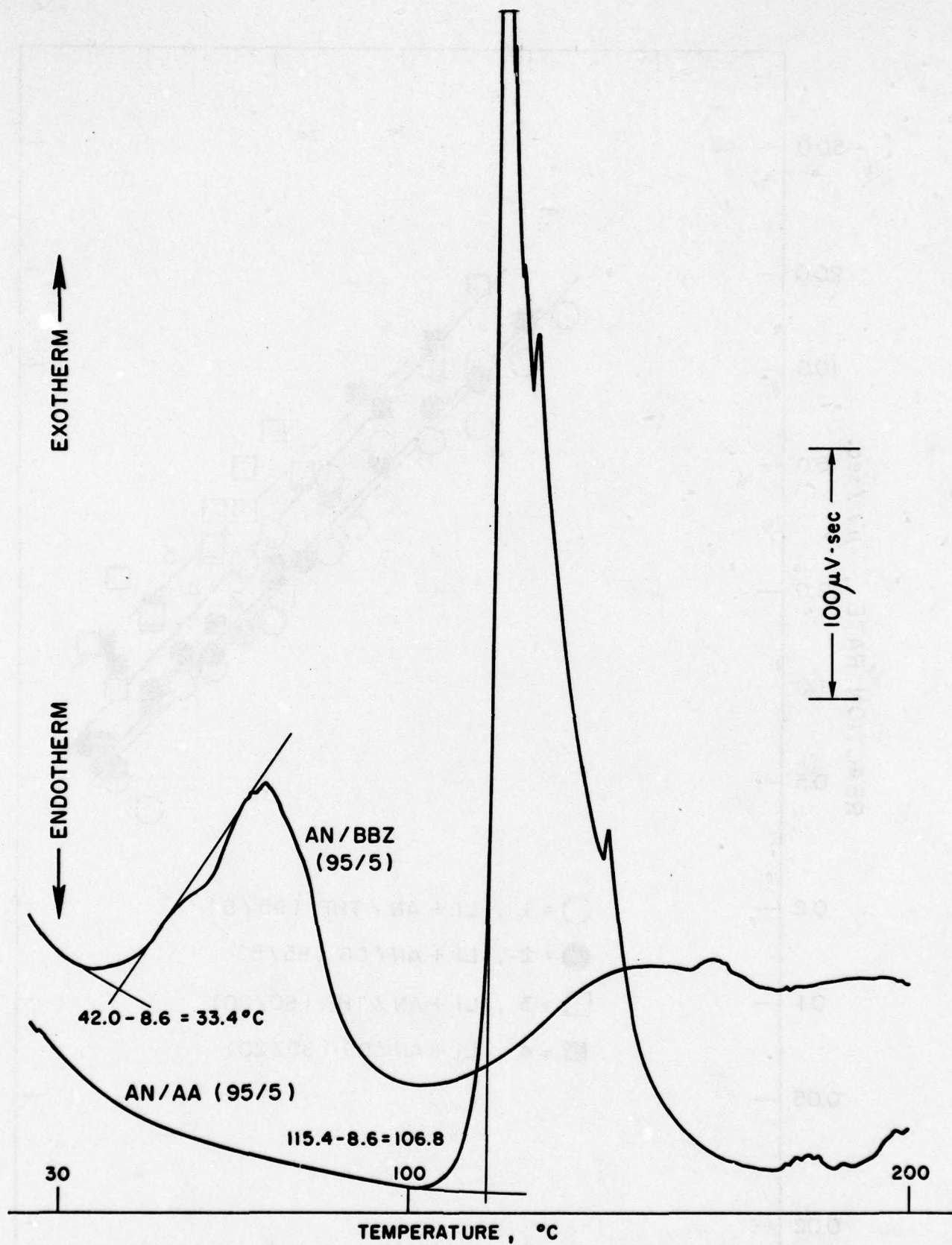
Figure 54. Thermograms at 5°C/Minute Showing the Determination of the Exotherm Initiation Temperature (1) Li + AN/bromobenzene (95/5), (2) Li + AN/acetic anhydride (95/5).
