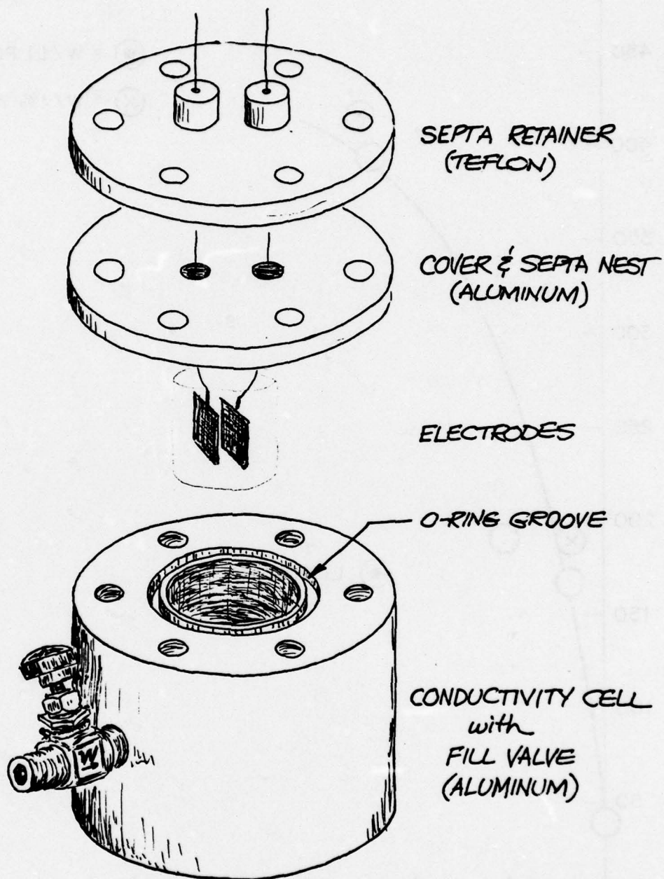
FIGURE 60: CONDUCTIVITY CELL for SO_2 ELECTROLYTES
