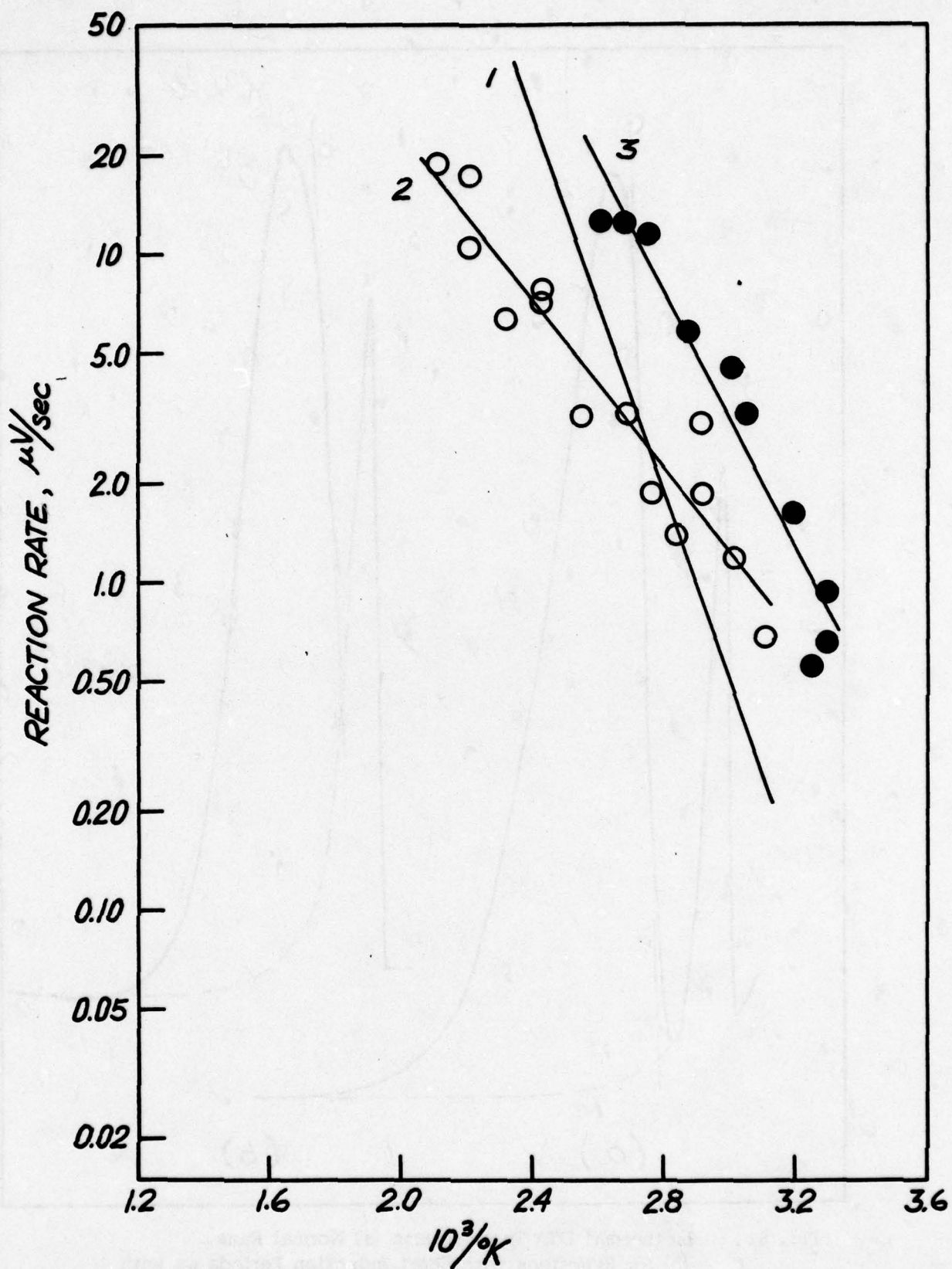
Fig. 52. Arrhenius Plots of Li + AN + DME System; (1) 0% DME, (2) 5% DME, and (3) 20% DME.
