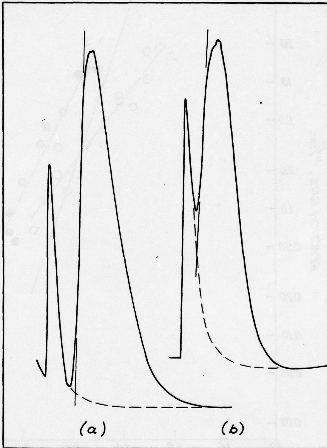
Fig. 51. Isothermal DTA Thermograms (a) Normal Runs, (b) for Reactions with Short Induction Periods as with Li + AN/MF (80/20).
