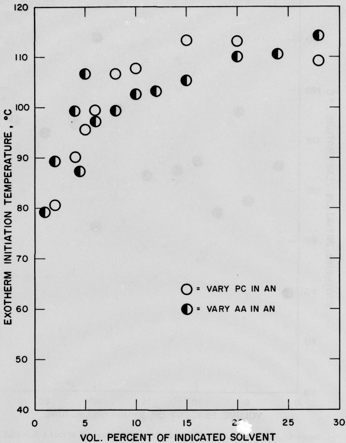
Figure 57. Exotherm Initiation from DTA @ 5°C/Minute. 0.000291 g Li + 20 \mu l of Solvent Mixture.
