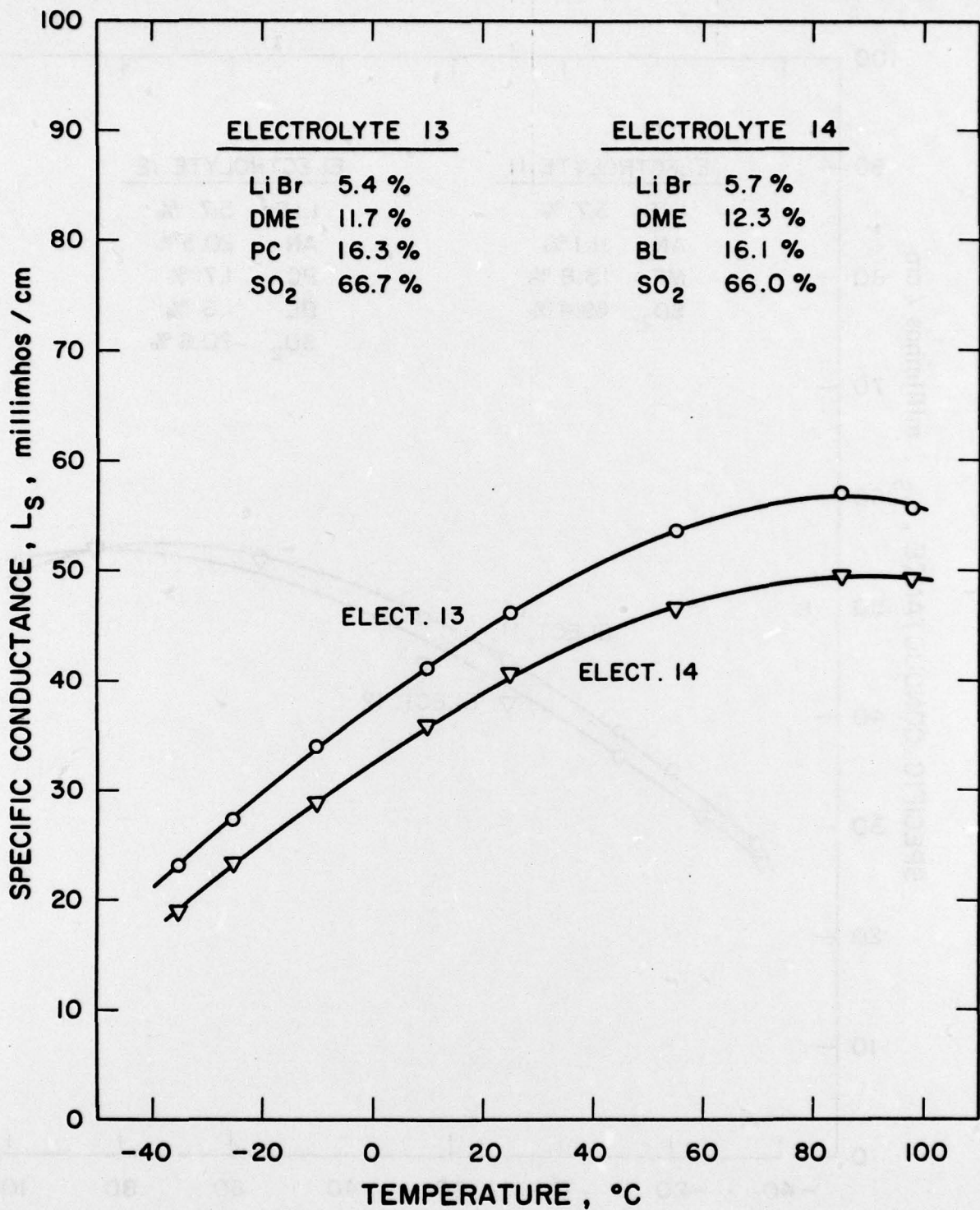
Figure 70. Specific Conductance vs. Temperature Electrolytes 13 and 14. Electrolyte 13: LiBr, DME/PC (50/50), SO 2 Electrolyte 14: LiBr, DME/BL (50/50), SO 2
