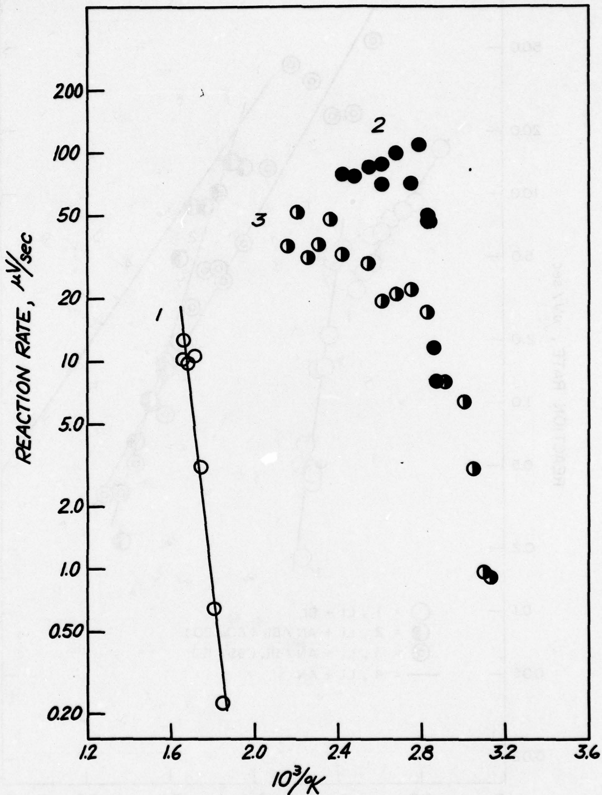
Fig. 50. Arrhenius Plots of Li + AN + MF System; (1) 0% AN, (2) 80% AN, and (3) 95% AN.
