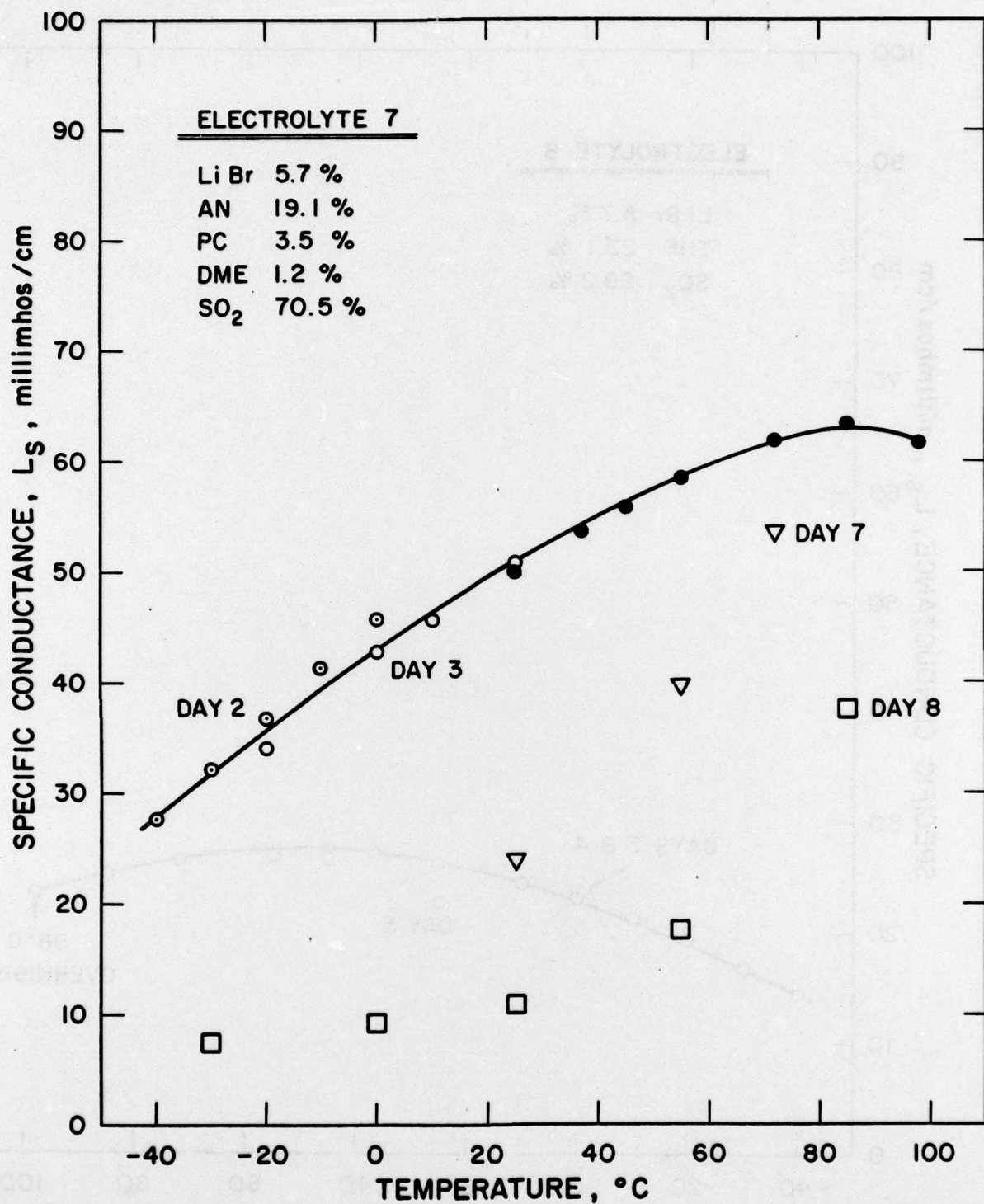
Figure 66. Specific Conductance vs. Temperature Electrolyte 7: LiBr, AN/PC/DME(85/10/5), SO 2
