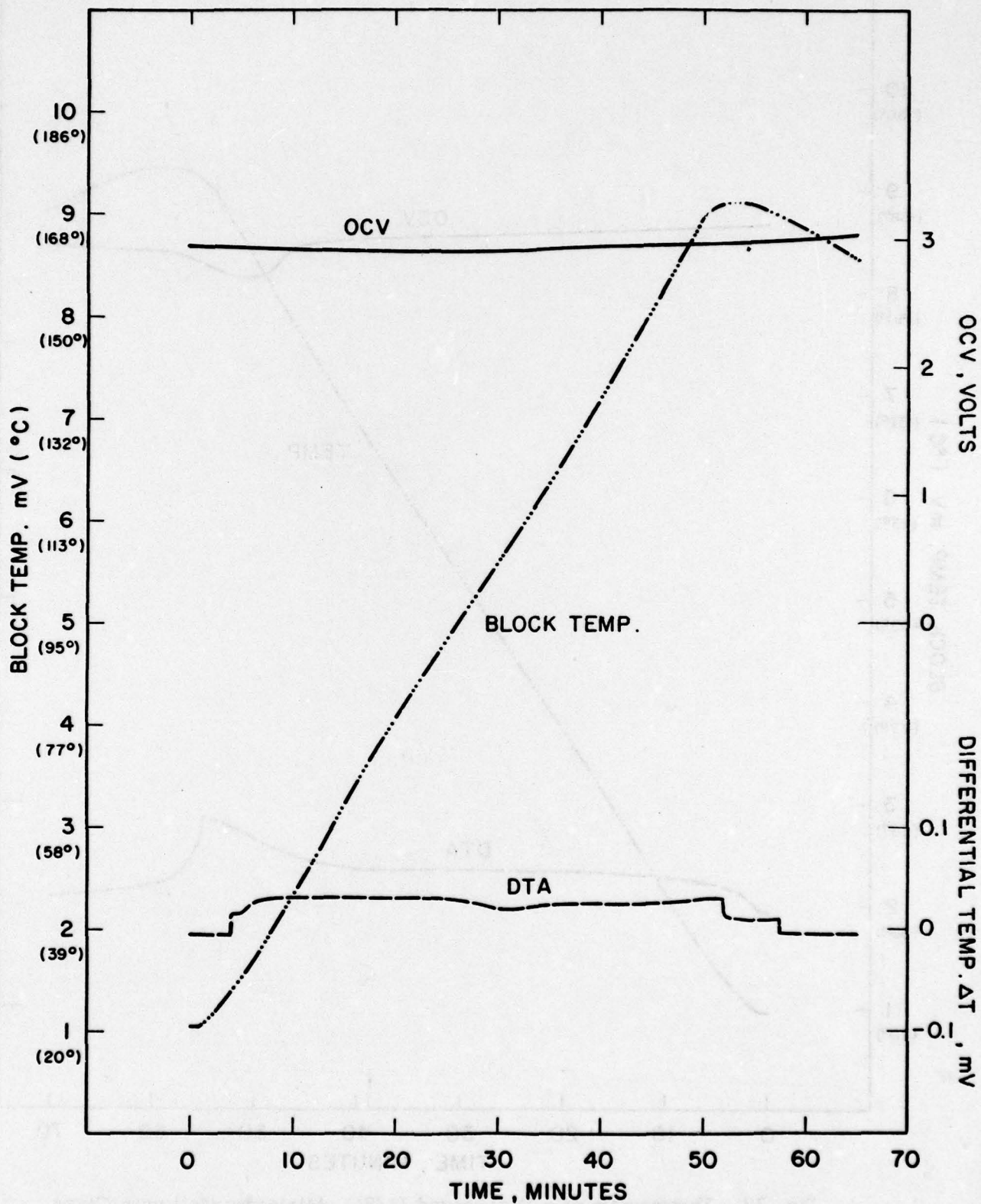
Fig. 37. Thermogram of an Undischarged Li/SO 2 Miniature Cell with Glass Filter Paper Separator.
