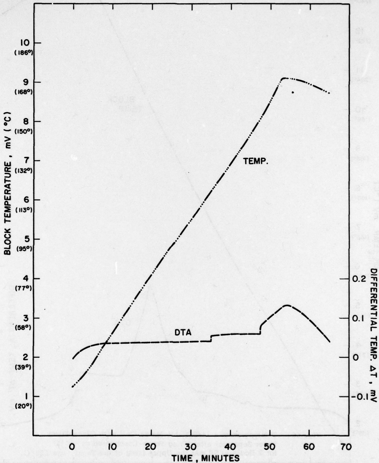
Fig. 39. Thermogram of a \text{Li}/\text{SO}_2 Miniature Cell with Glass Filter Paper Separator after being Force-Discharged at -30^\circ\text{C} for 3 Hours at 90 mA; Upper Limit of Temperature was 170^\circ\text{C} .
