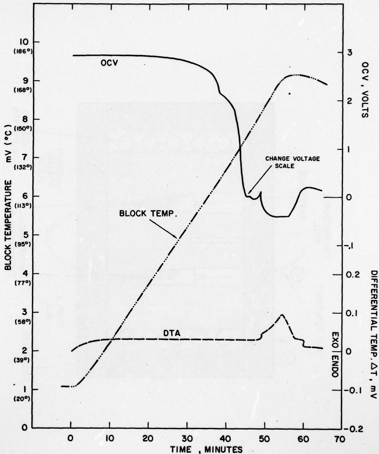
Fig. 26. Thermogram of a Discharged Miniature Li/SO 2 Cell of Standard Construction, Discharge Current 1 mA; Discharge Capacity 193 mAhr.
