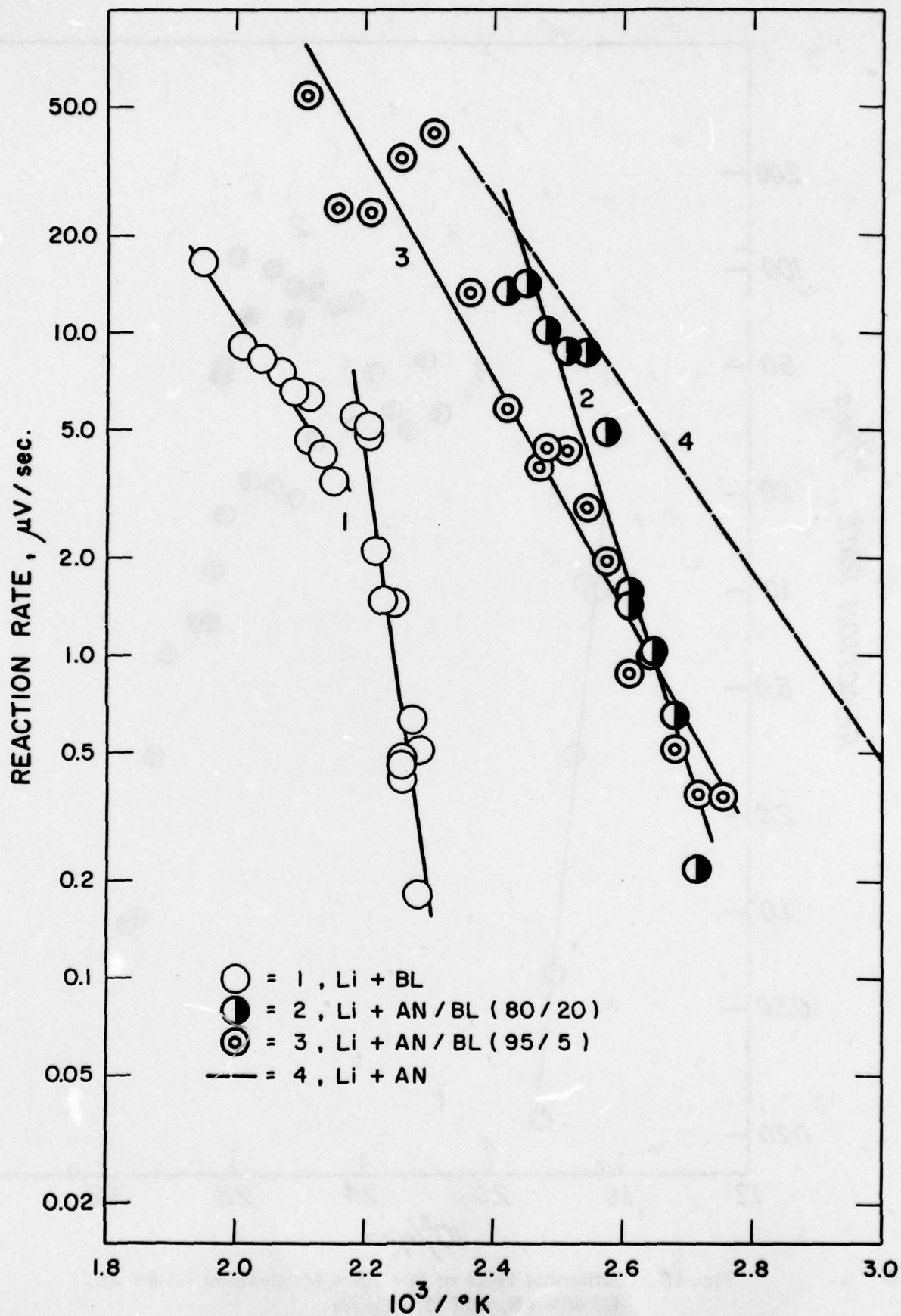
Figure 49. Arrhenius Plots of the Li + AN/BL system; (1) 0% AN, (2) 80% AN, (3) 95% AN and (4) 100% AN. 101
