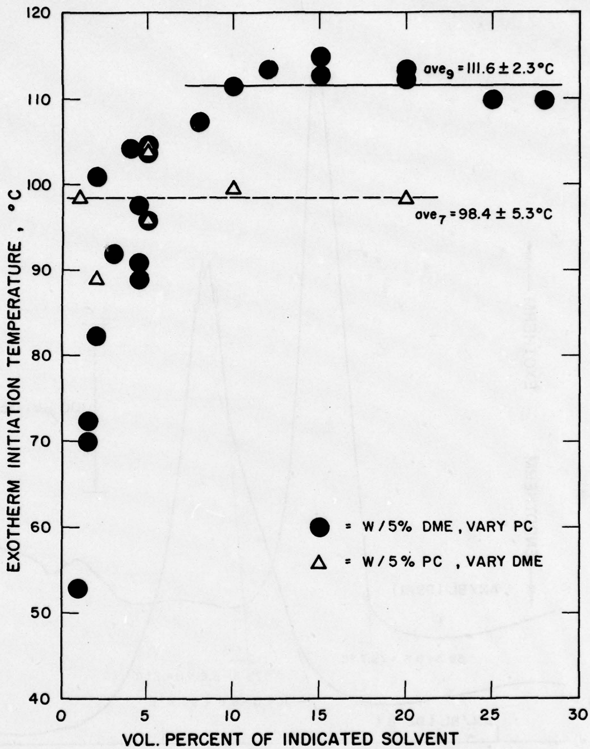
Figure 56. Exotherm initiation from DTA @ 5°C/Minute. 0.00029 g Li + 20μl of indicated AN/DME/PC
