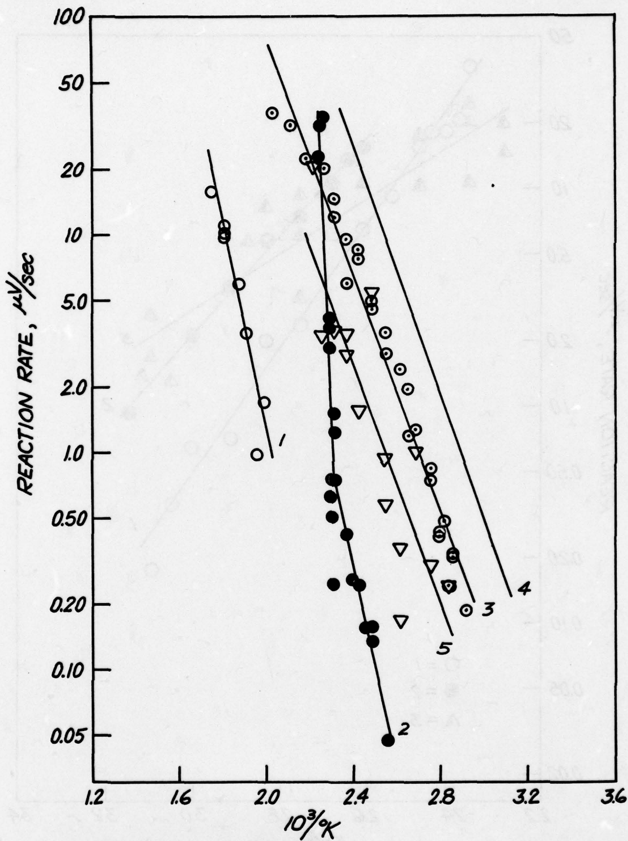
Fig. 48. Arrhenius Plots of the Li + AN + PC System; (1) 0% AN, (2) 50% AN, (3) 80% & 95% AN, (4) 100% AN, and (5) 0% PC and 3% \text{SO}_2 . 100
