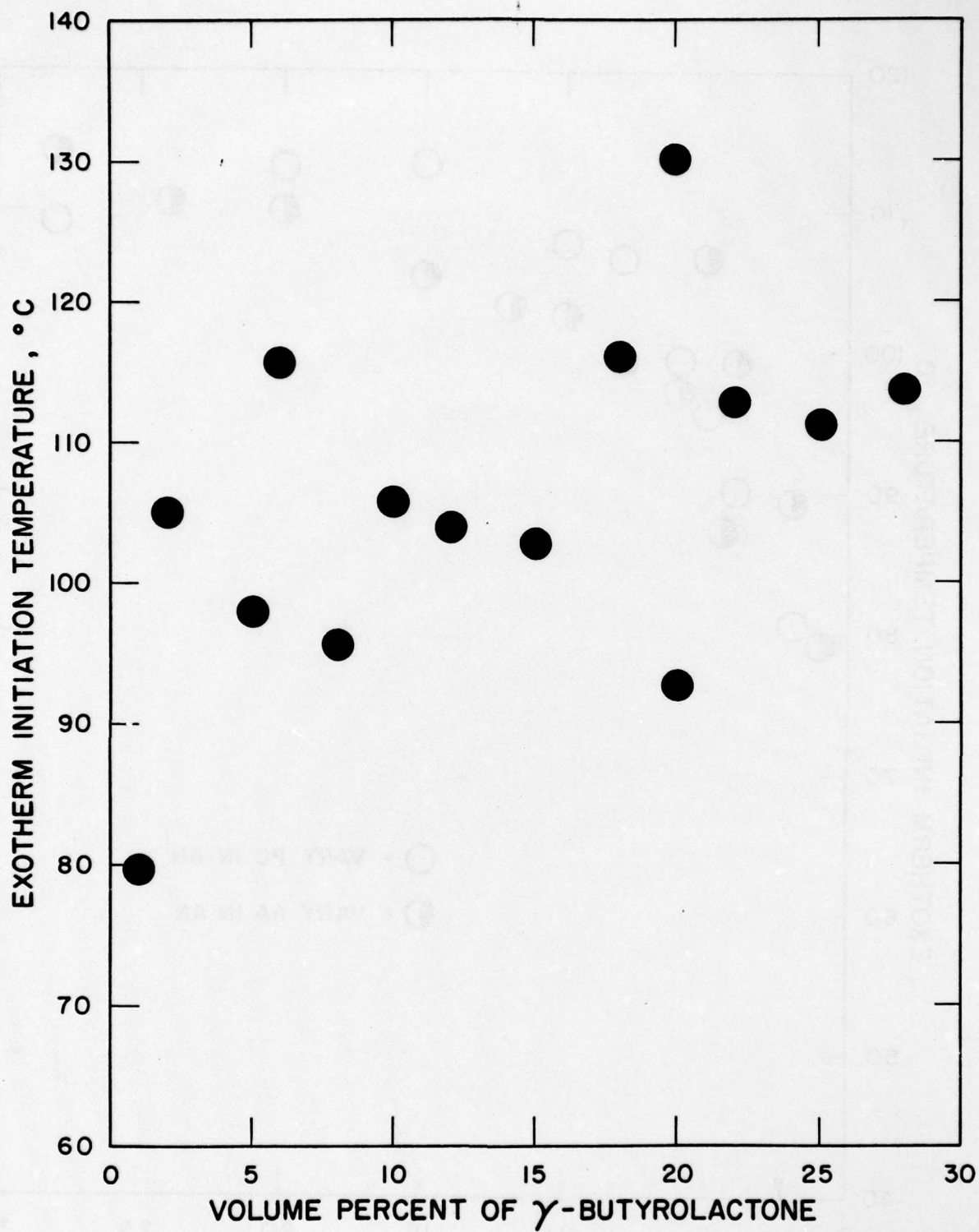
Figure 58. Exotherm Initiation from DTA @ 5°C/Minute. 0.000291 g Li + 20 \mu l of AN/BL Mixture.
