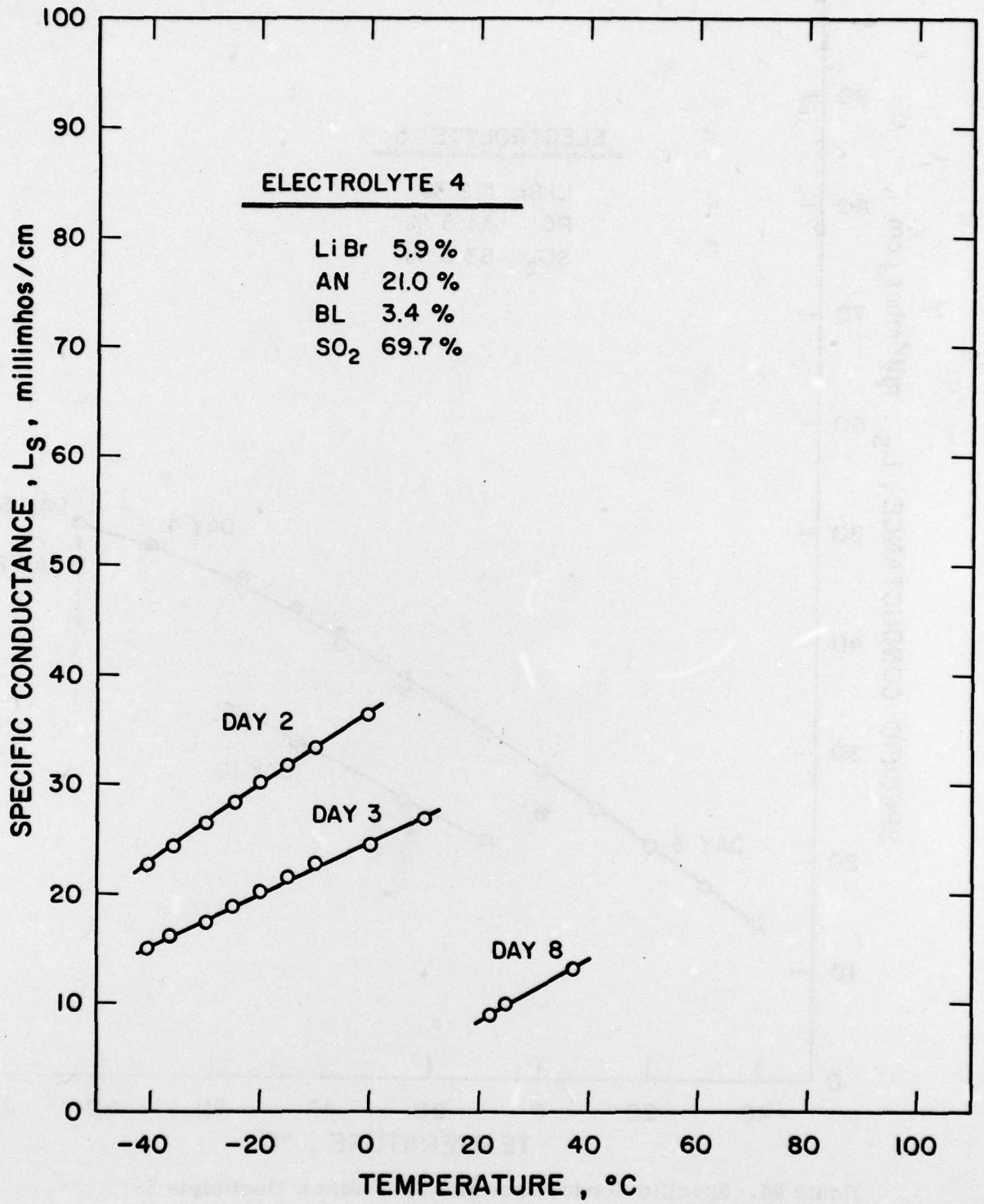
Figure 63. Specific Conductance vs. Temperature for Electrolyte 4: LiBr, AN/BL (90/10), SO 2 .
