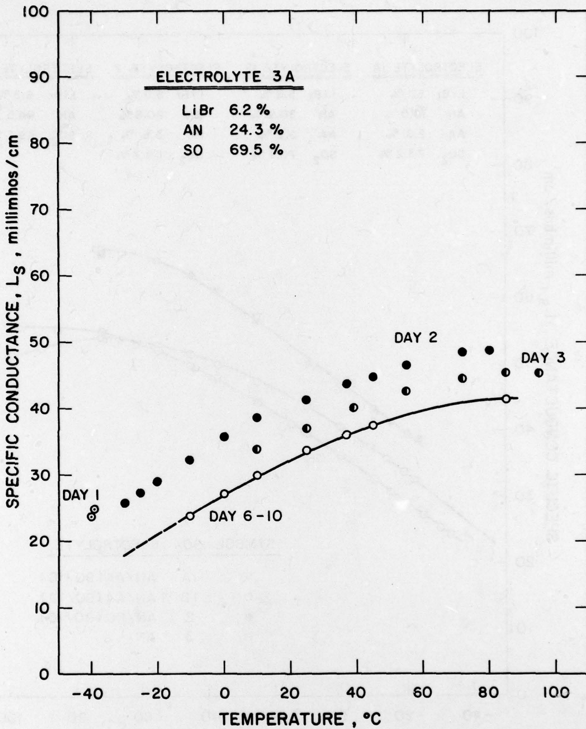
Figure 62. Specific Conductance vs. Temperature Electrolyte 3A: LiBr, AN, SO_2
