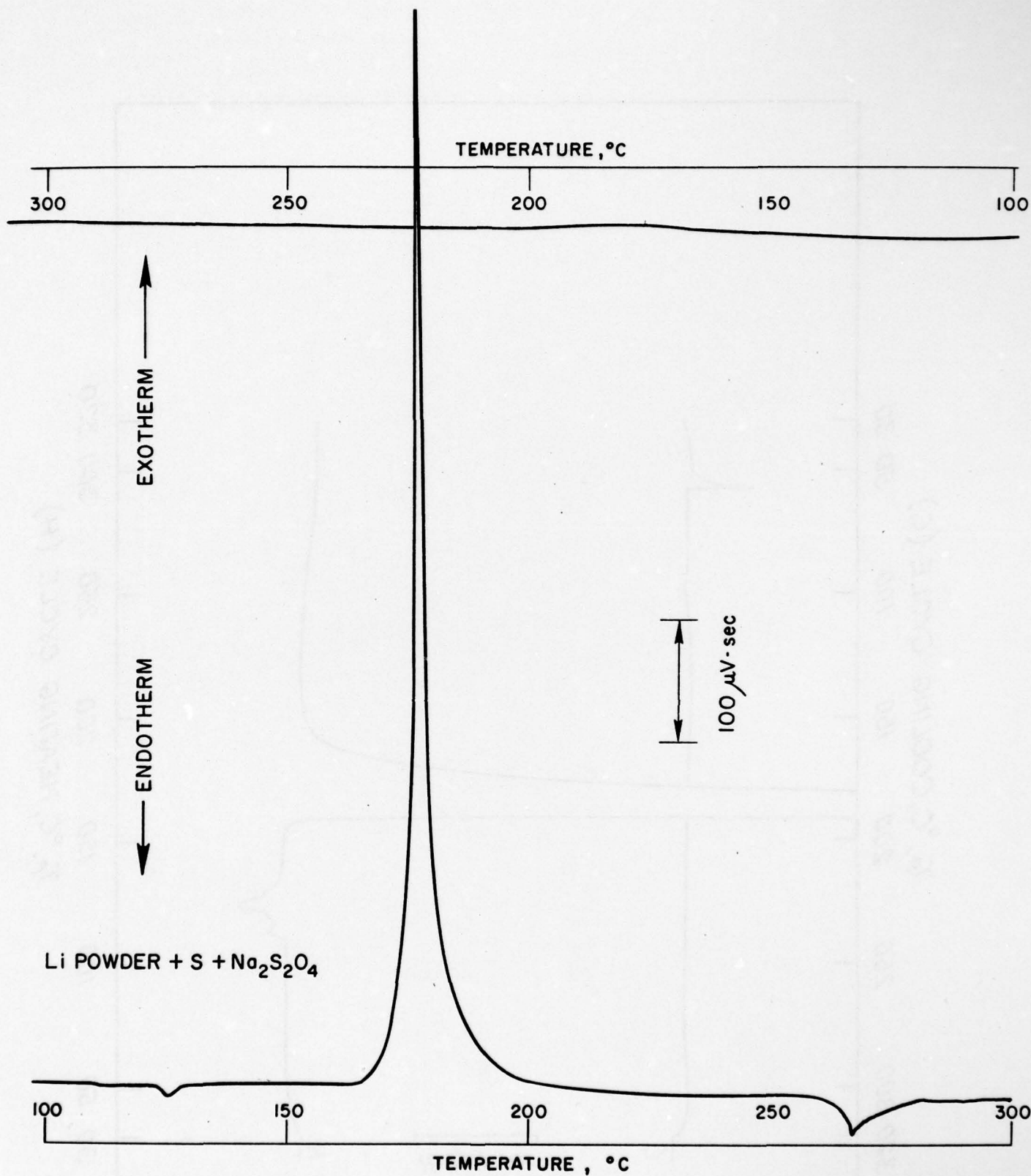
Figure 18. Thermogram of Powdered Li (0.00039 g) + S (0.00147 g) + Na 2 S 2 O 4 (0.00644 g)
