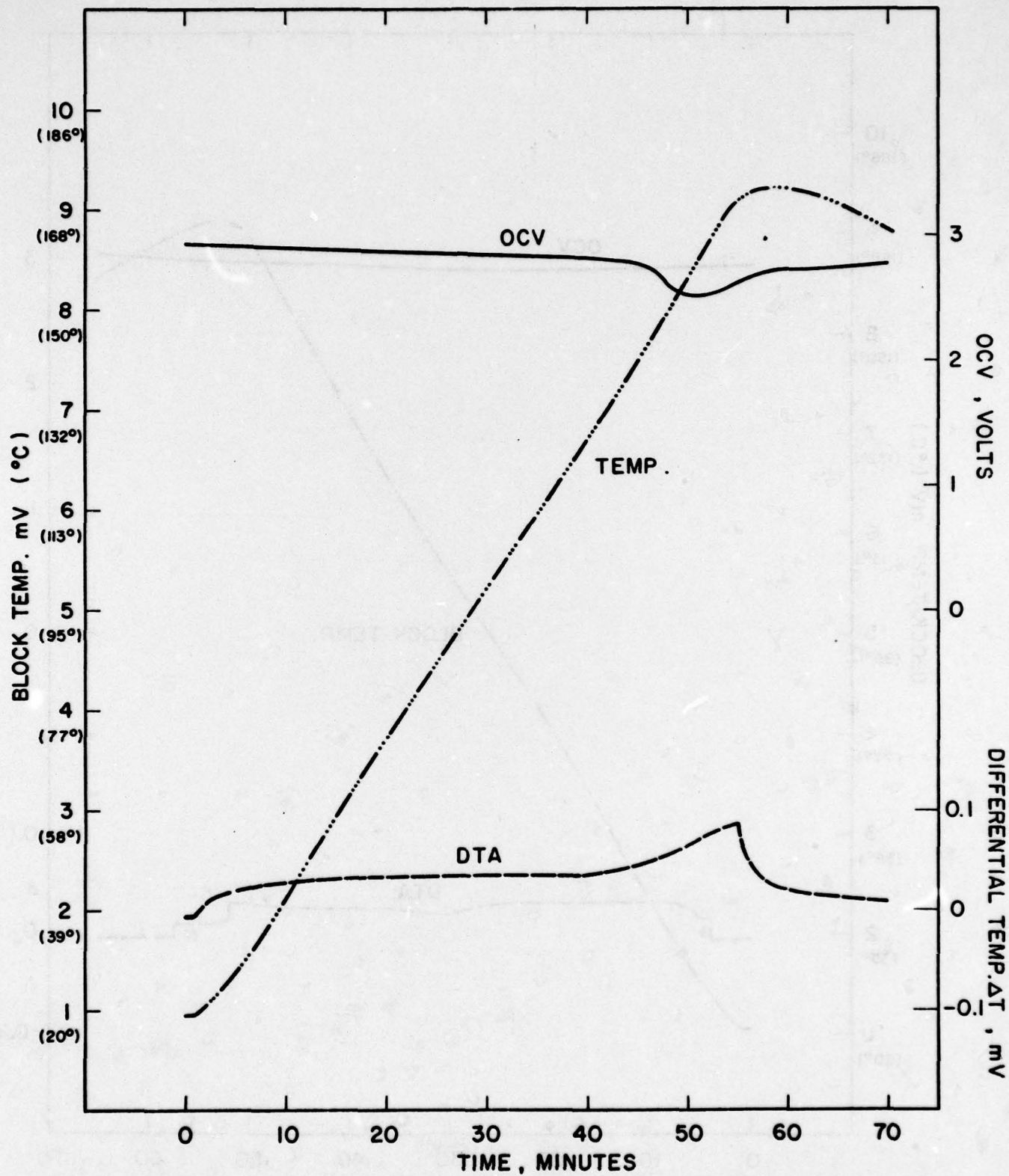
Fig. 38. Thermogram of a Discharged Li/SO 2 Miniature Cell with Glass Filter Paper Separator; Discharge Current, 10 mA; Discharge Temperature, 25°C. 90
