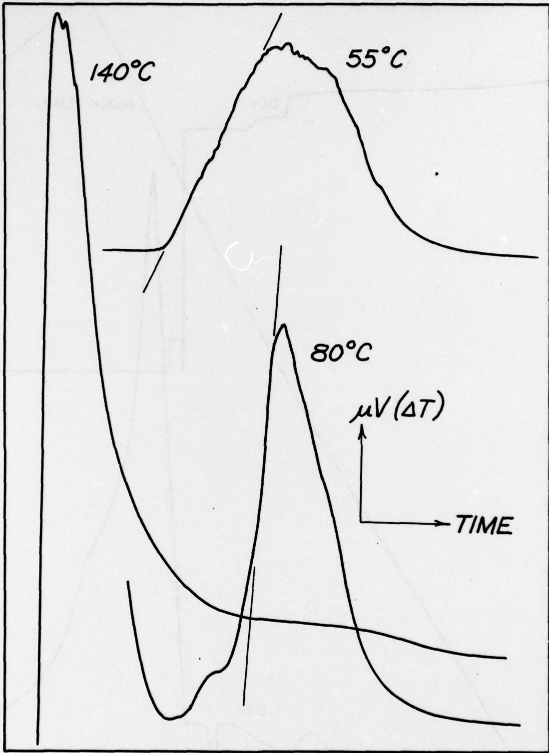
Fig. 46. Typical Isothermal DTA Thermograms of Li + AN System at Various Temperatures.
