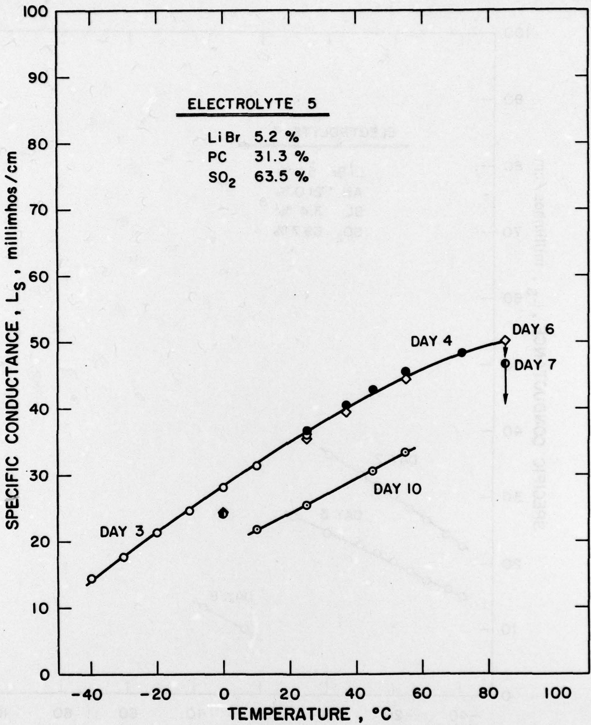
Figure 64. Specific Conductance vs. Temperature Electrolyte 5: LiBr, PC, SO 2 .
