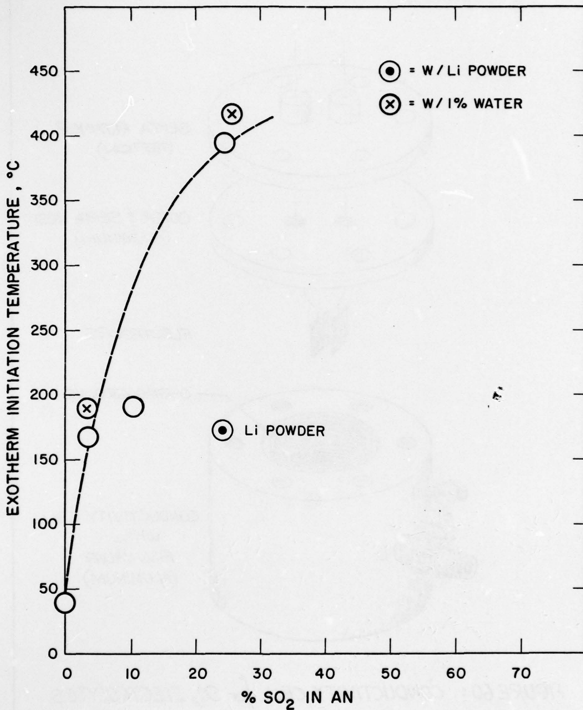
Figure 59. Exotherm Initiation Temperature of the Li + AN. Reaction as a Function of SO 2 concentration
