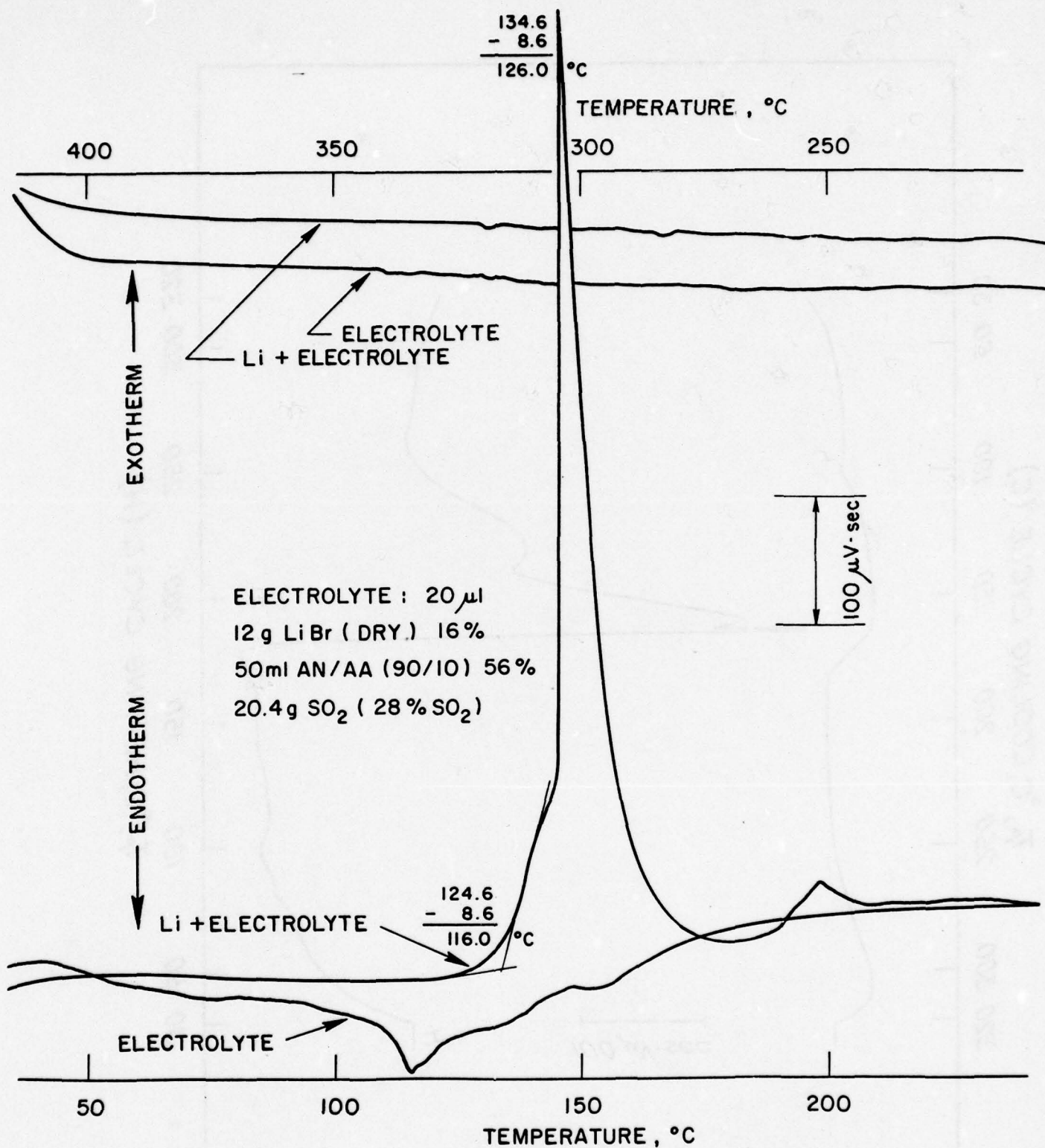
Figure 12. Thermogram of Li (0.00029g) + 20 \mu\text{l} Electrolyte (28% SO 2 , 56% AN/AA (90/10), 16% LiBr). 5 ^\circ\text{C}/\text{Minute} .
