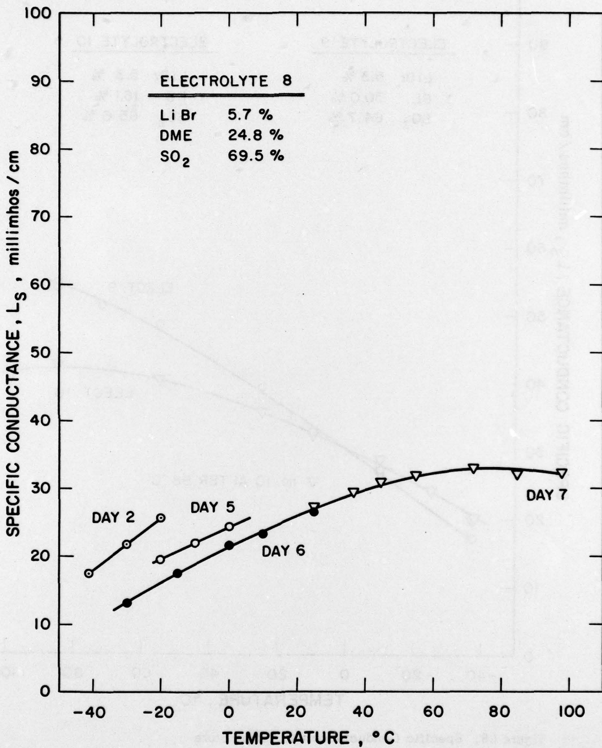
Figure 67. Specific Conductance vs. Temperature Electrolyte 8: LiBr, DME, SO 2
