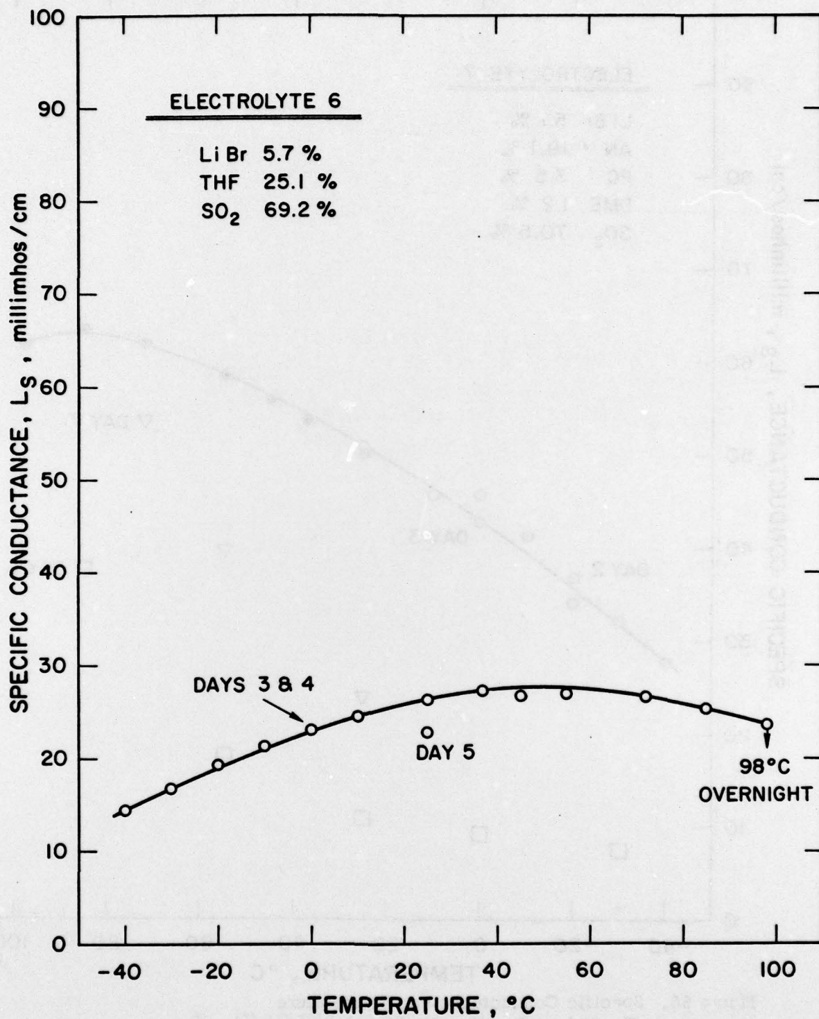
Figure 65. Specific Conductance vs. Temperature Electrolyte 6: LiBr, THF, SO 2 .
