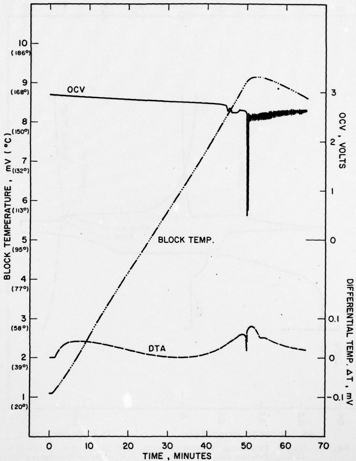
Fig. 31. Thermogram of a Discharged Miniature Li/SO 2 Cell with PC in the Electrolyte; Discharge Current, 10 mA; Discharge Temperature, 25°C. 83
