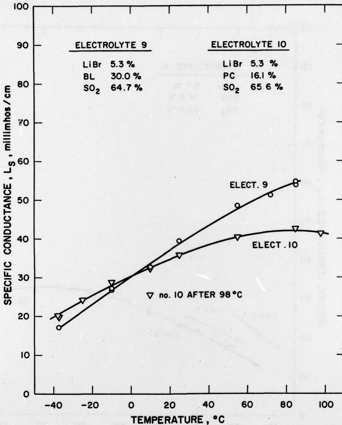
Figure 68. Specific Conductance vs. Temperature Electrolytes 9 and 10. Electrolyte 9: LiBr, BL, SO 2 and Electrolyte 10: LiBr, PC, SO 2
