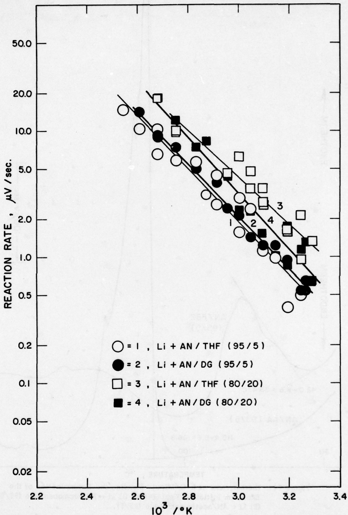
Figure 53. Arrhenius Plots of (1) Li + AN/THF (95/5), (2) Li + AN/DG (95/5), (3) Li + AN/THF (80/20), and (4) Li + AN/DG (80/20) Systems.
