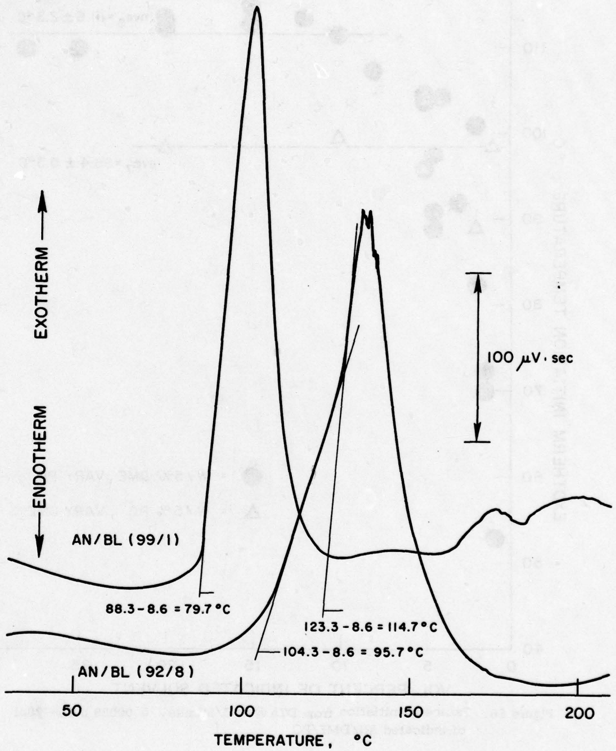
Figure 55. Thermograms for the Li + AN/BL Reaction
