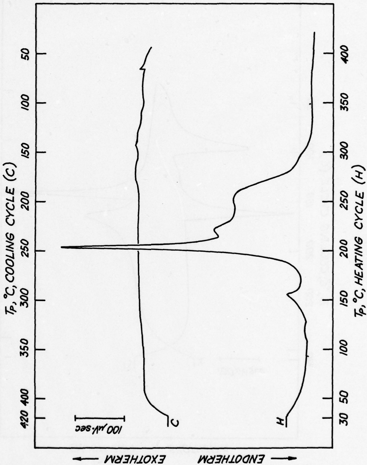
Fig. 3. Thermogram of \text{Na}_2\text{S}_2\text{O}_4 (0.0333 gm); 5^\circ\text{C}/\text{Minute} .
