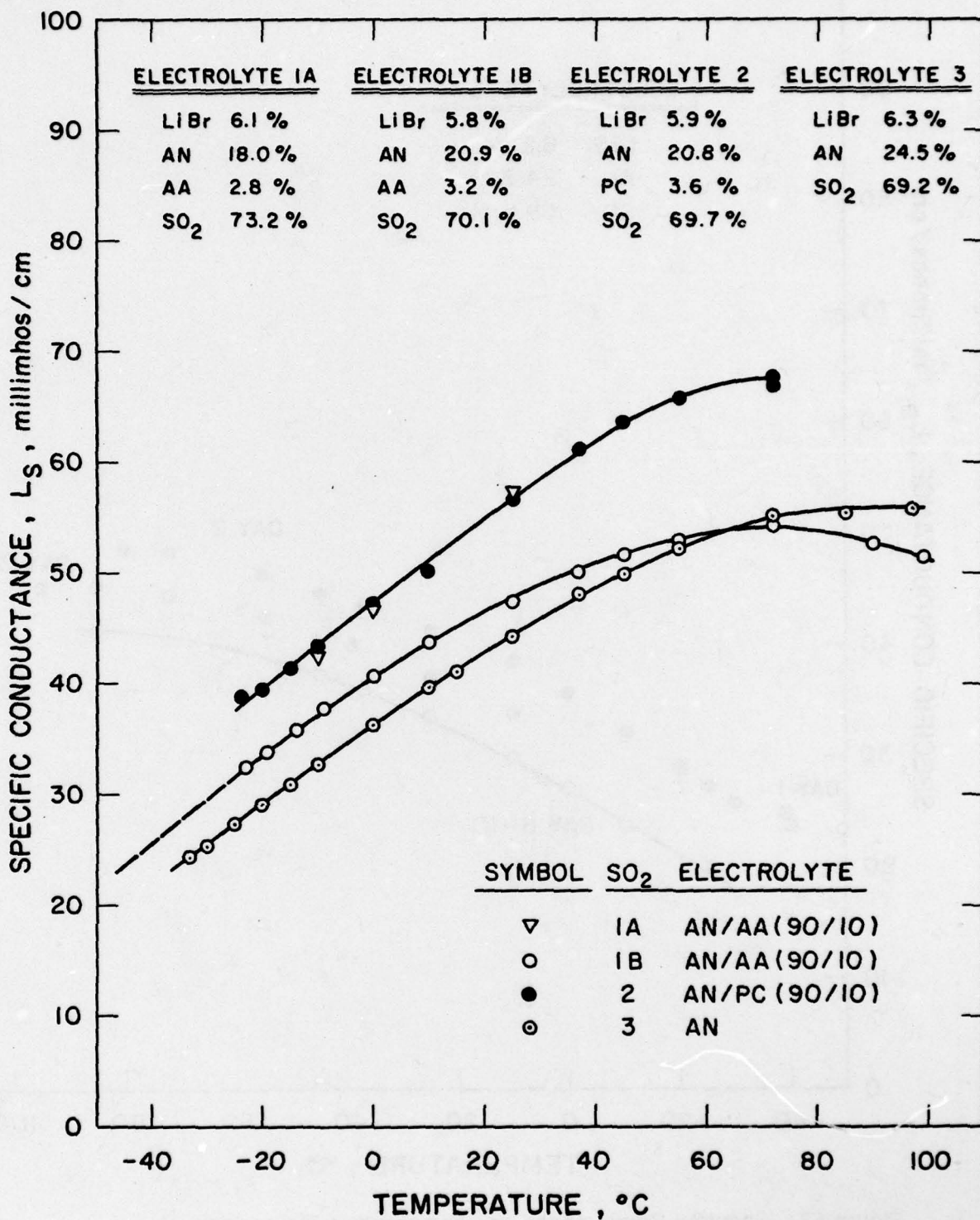
Figure 61. Specific Conductance vs. Temperature for SO 2 Electrolytes, in Aluminum Cell.
