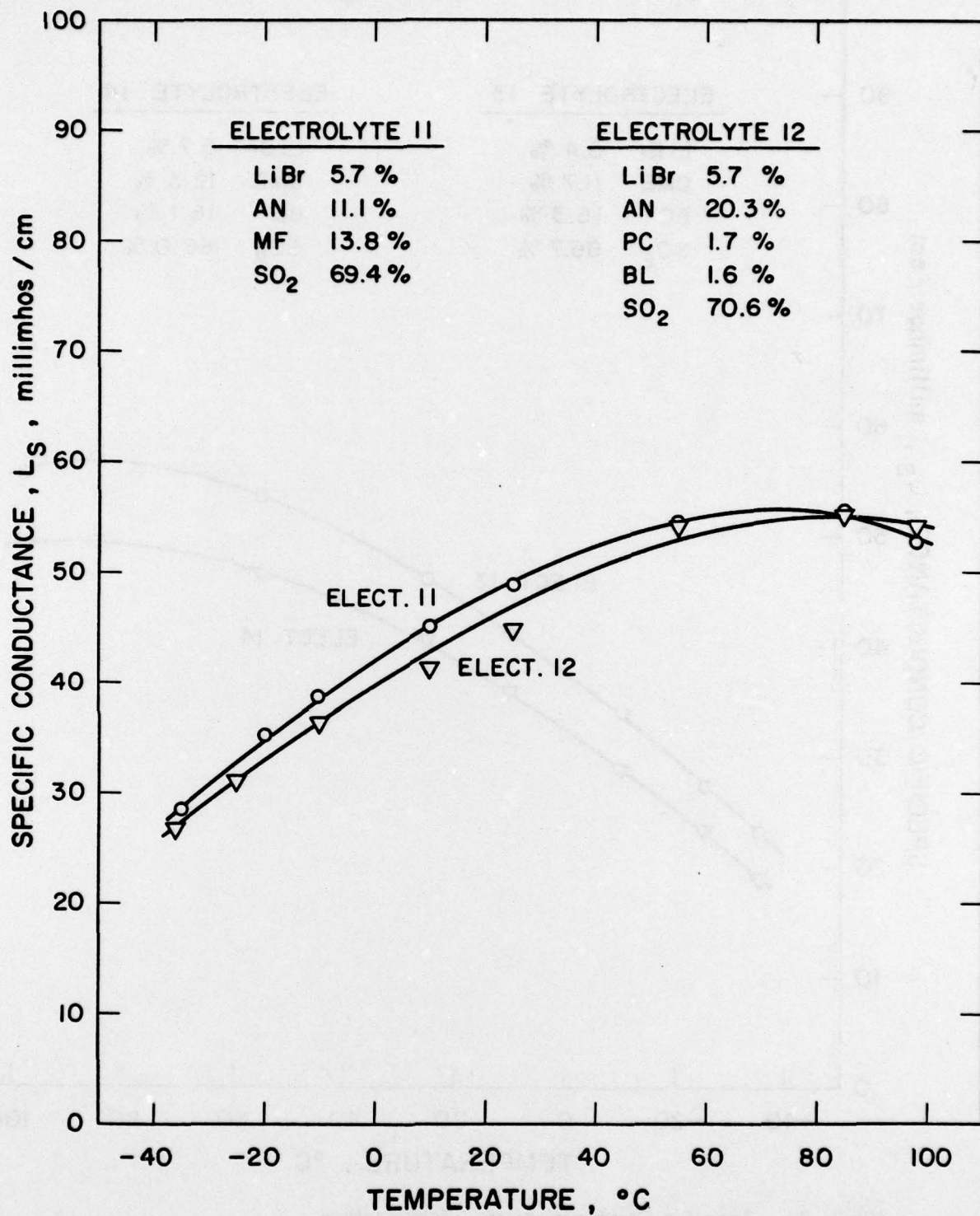
Figure 69. Specific Conductance vs. Temperature Electrolytes 11 and 12.
