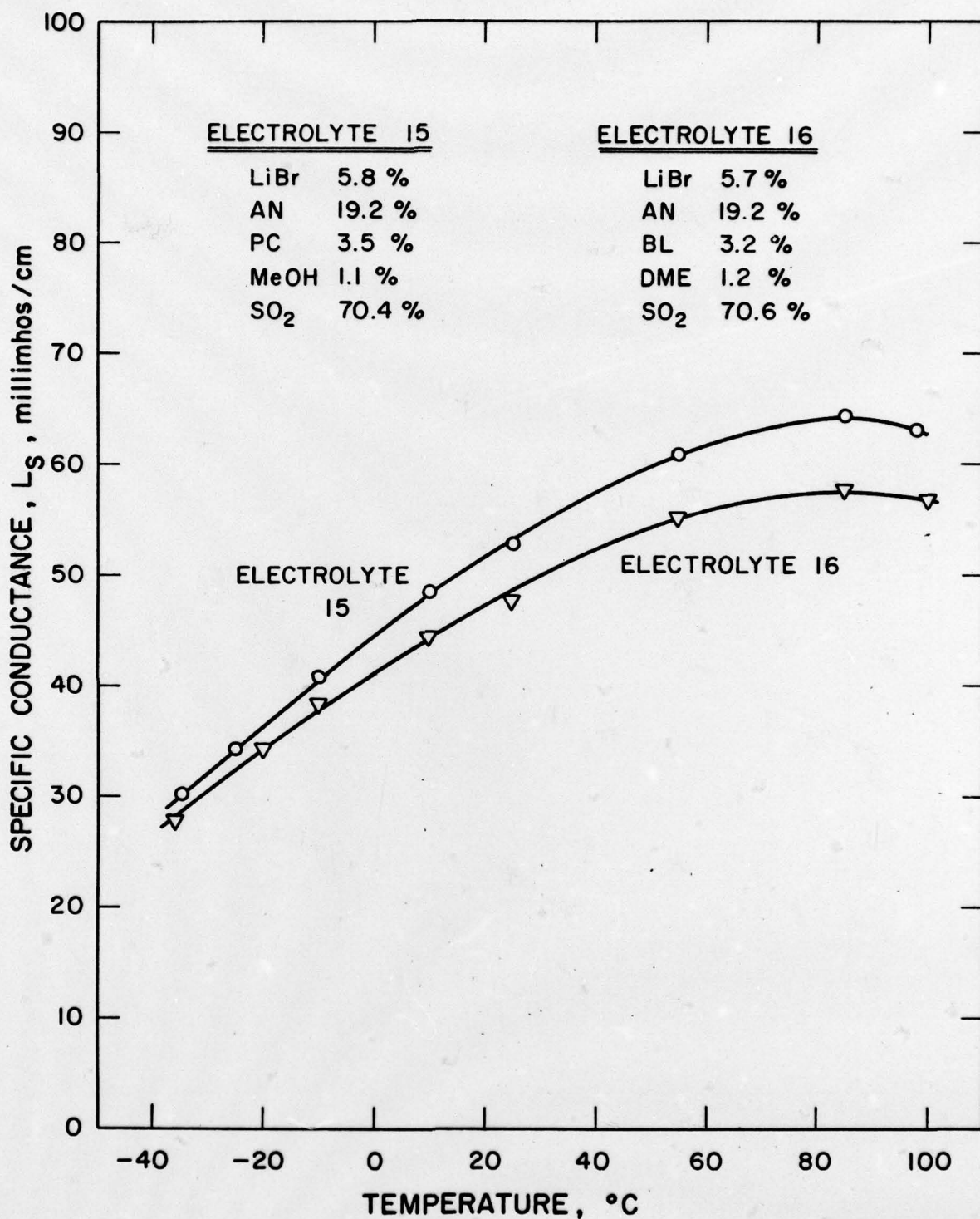
Figure 71. Specific Conductance vs. Temperature Electrolyte 15: LiBr, AN/PC/MeOH(85/10/5), SO 2 Electrolyte 16: LiBr, AN/BL/DME(85/10/5), SO 2
