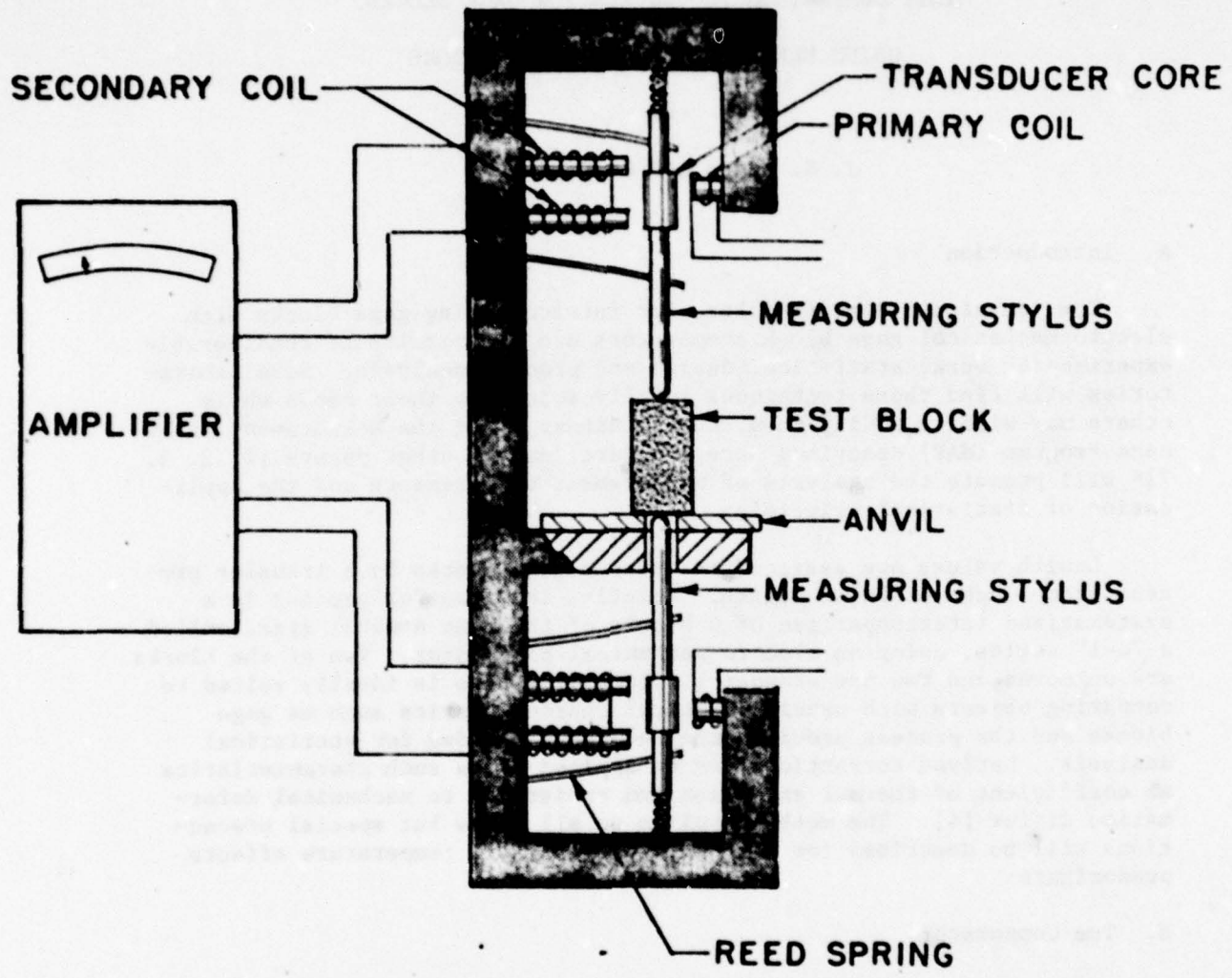
ELEMENTS OF A MECHANICAL COMPARATOR OF LENGTHS.
