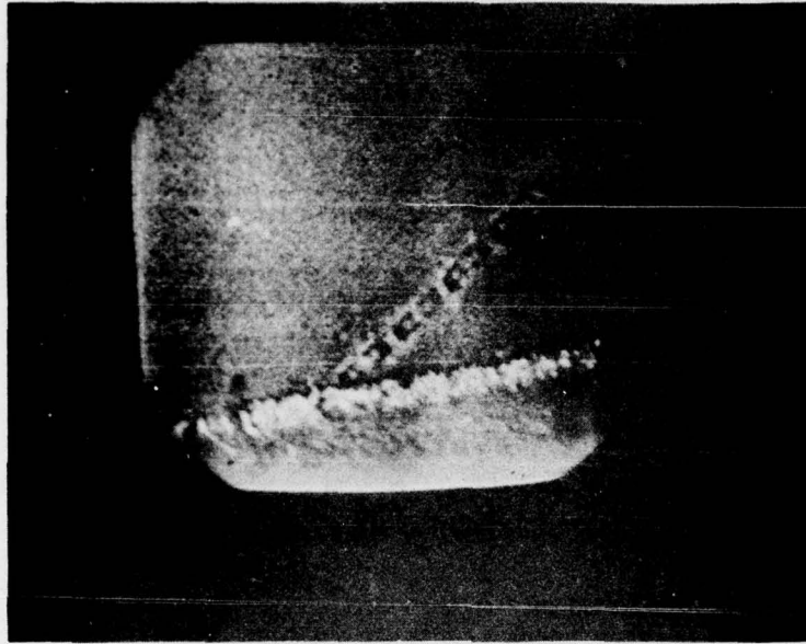
Figure 26. TELEVISION. Securing track on flight deck of SARATOGA showing radio antenna bent across deck to port. ABCR Photo No. 5106-12.
