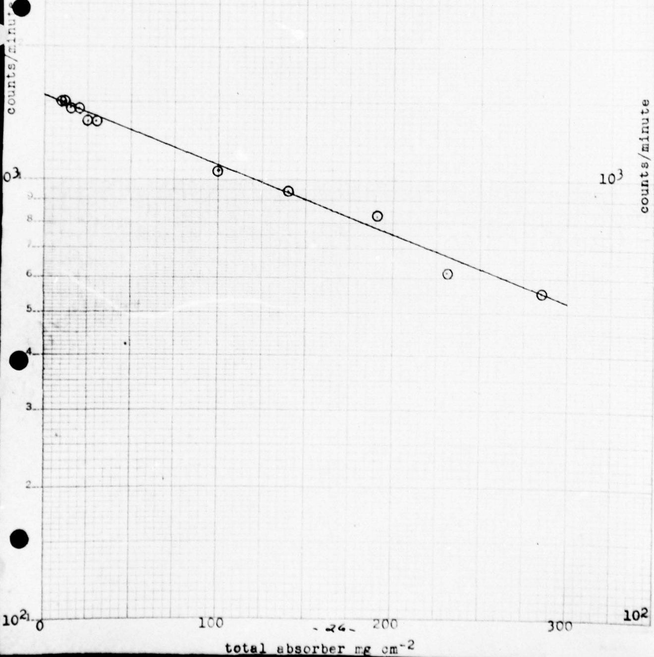
Figure 2. Gross absorption curve for sand, midway between Bikini Island and Amen Island.
