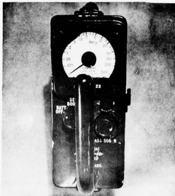
Fig. 1.2 Radiacmeter SU-13
