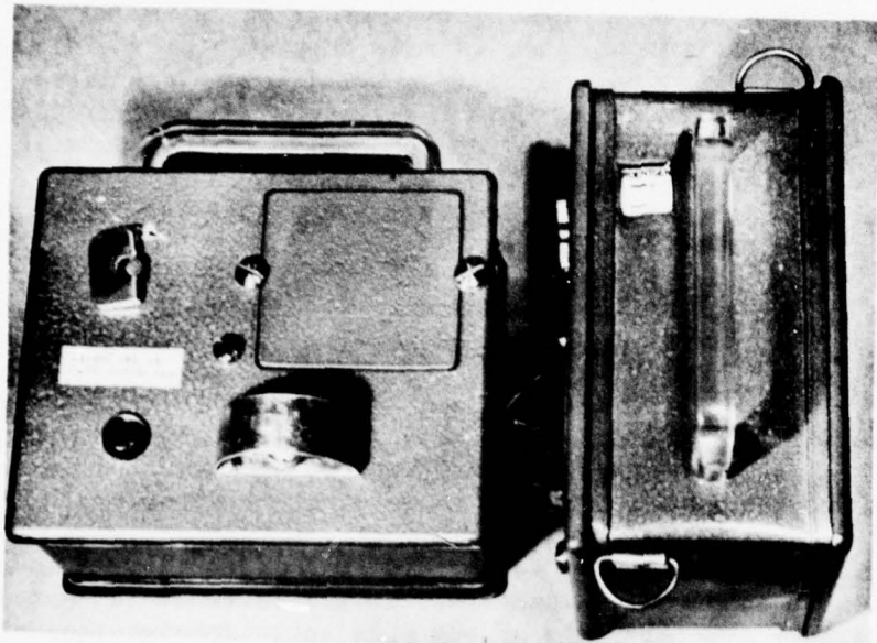
Fig. 1.9 ERDL #472 Recycling Ionization Chamber Dosimeter
