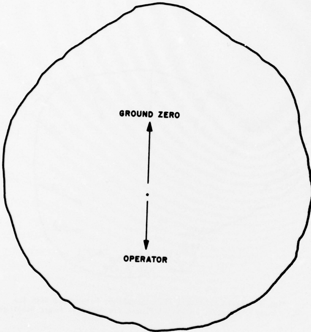
Fig. A.2 Response of The AN/PDR-18 To Radiation Field of Fig. A.1
