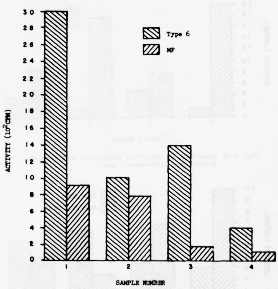
Fig. 4.12 Comparison of Activities Measured on Type 6 and MF Filters from Instruments A and B
