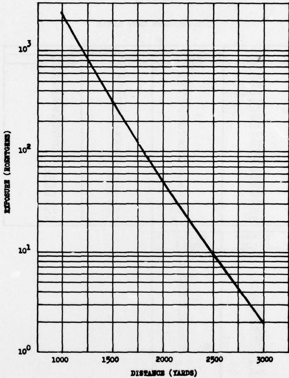
Fig. 2.16 R vs D, Shot 8
