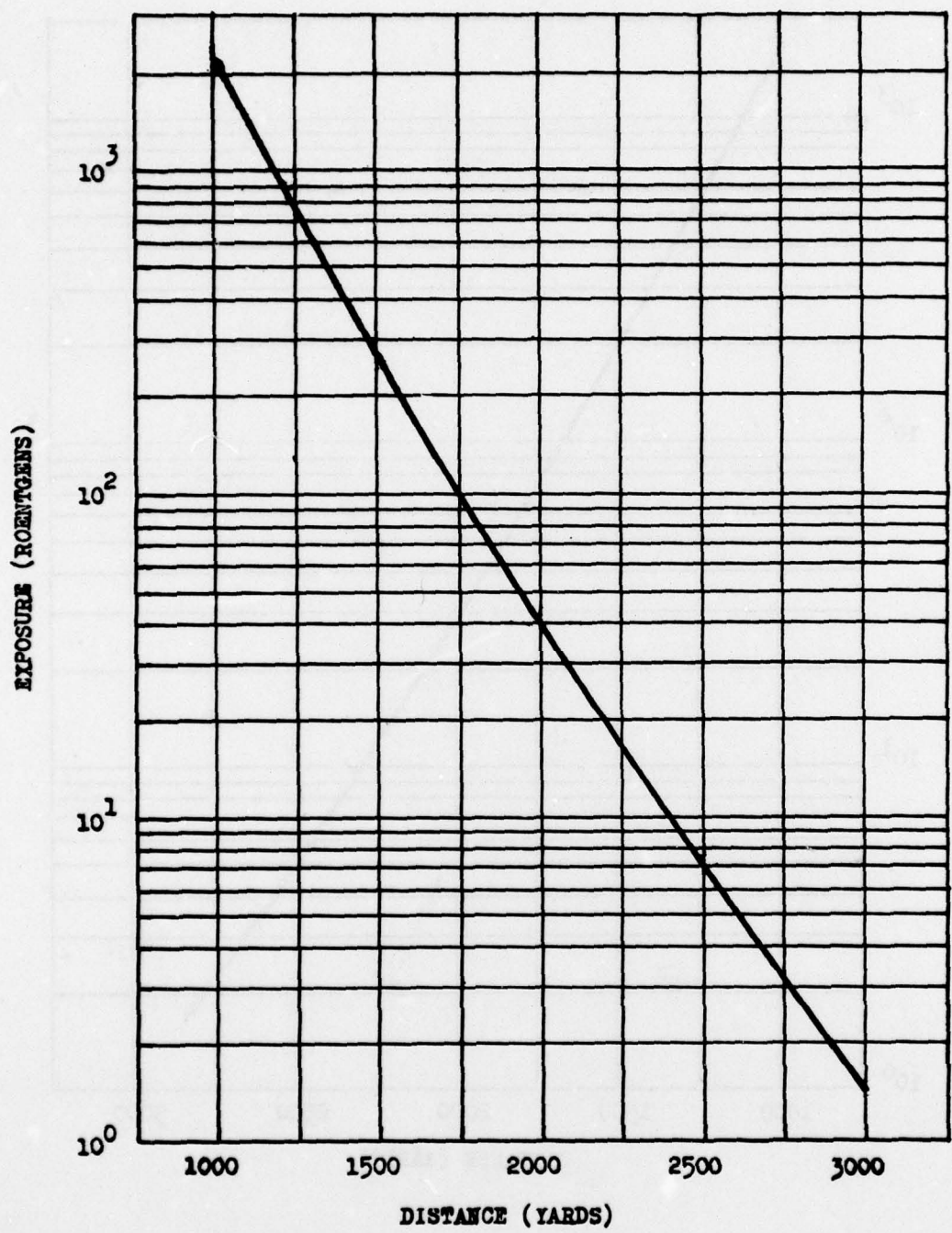
Fig. 2.15 R vs D, Shot 7
