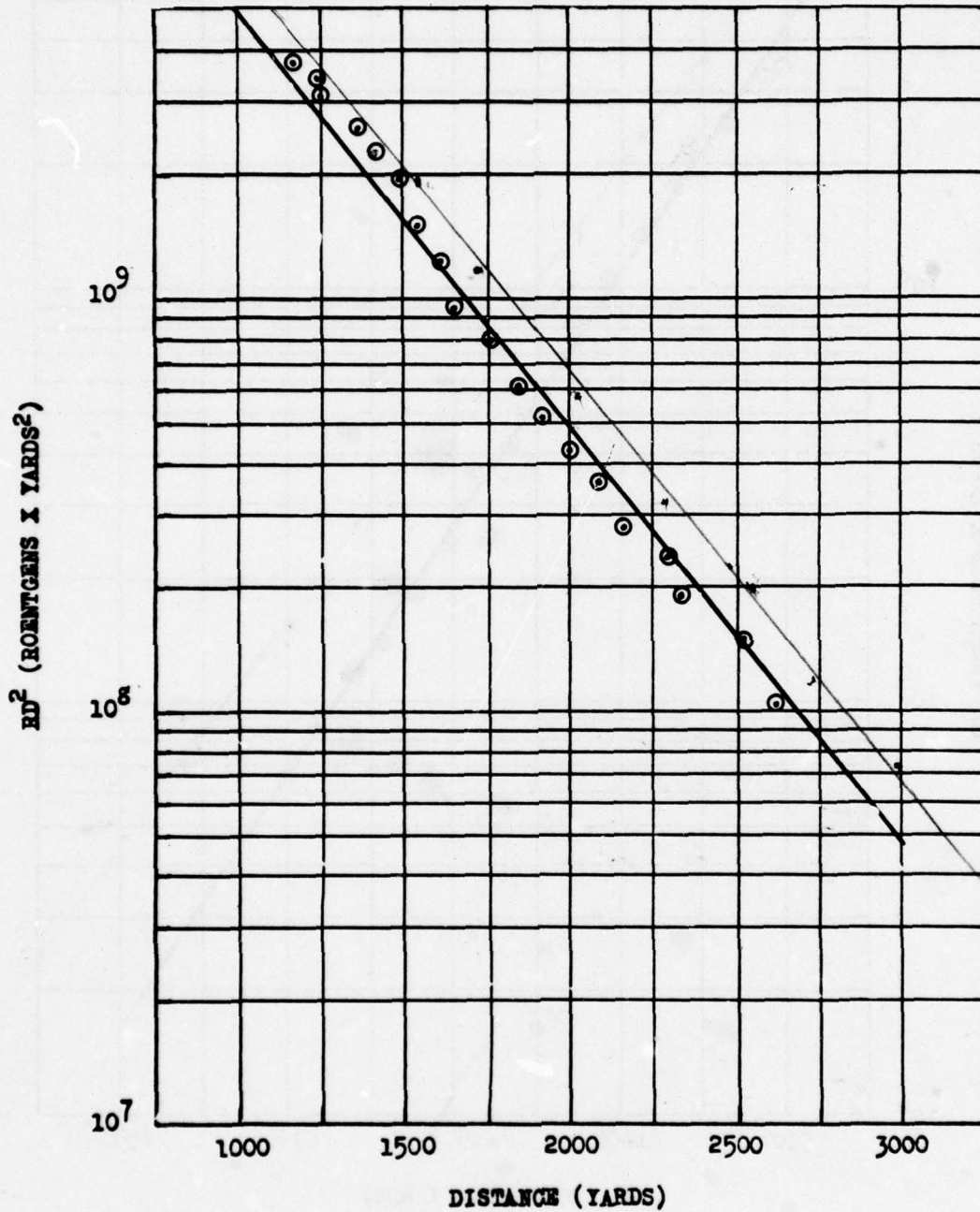
Fig. 2.2 RD 2 vs D, Shot 3
