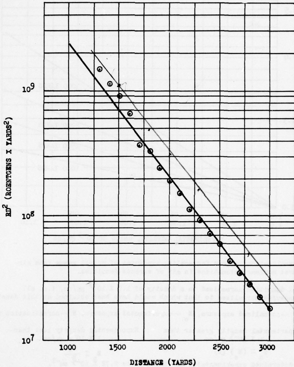
Fig. 2.7 RD^2 vs D, Shot 8
