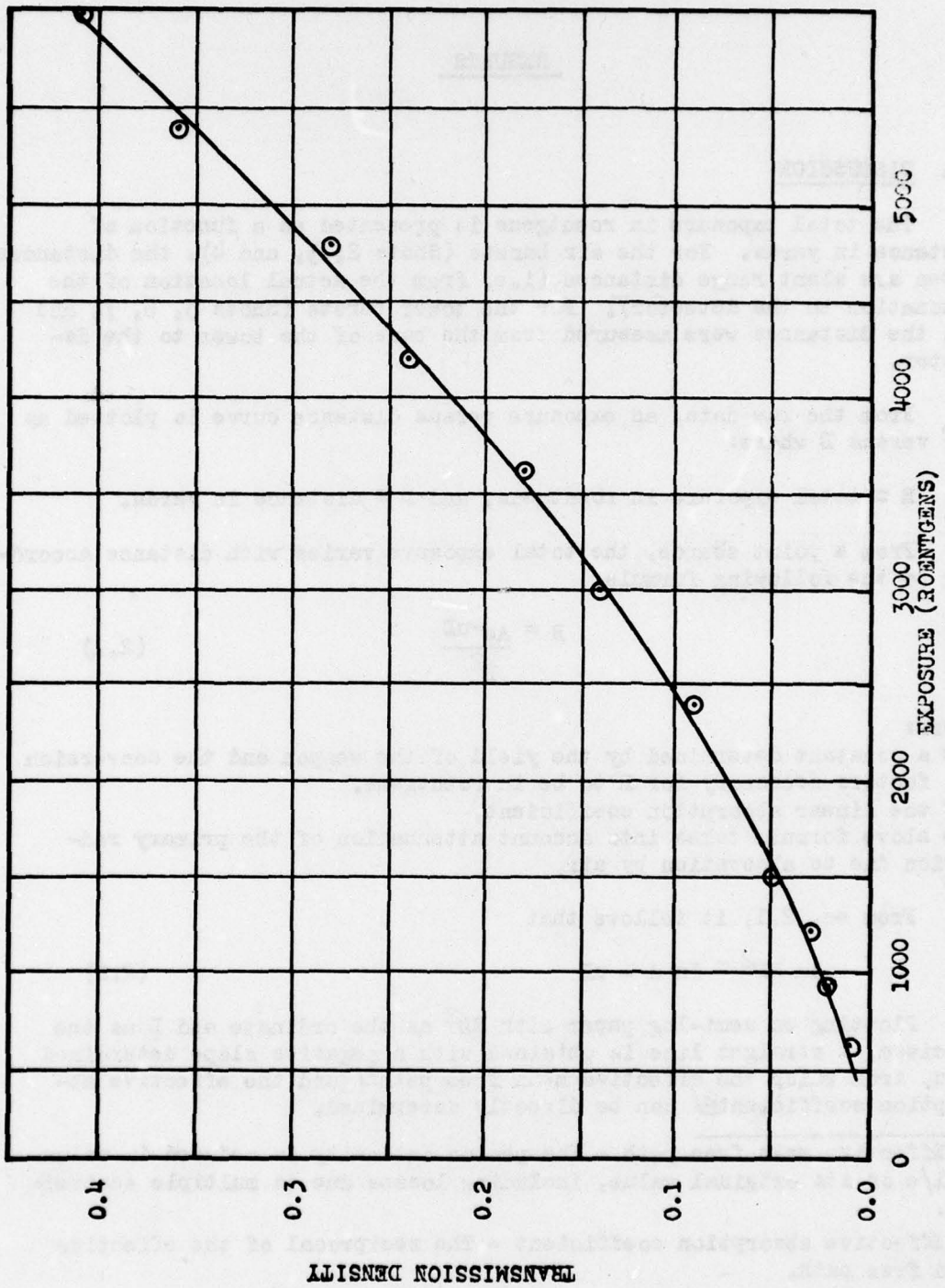
Fig. 1.5 Eastman 545-0 Calibration Curve
