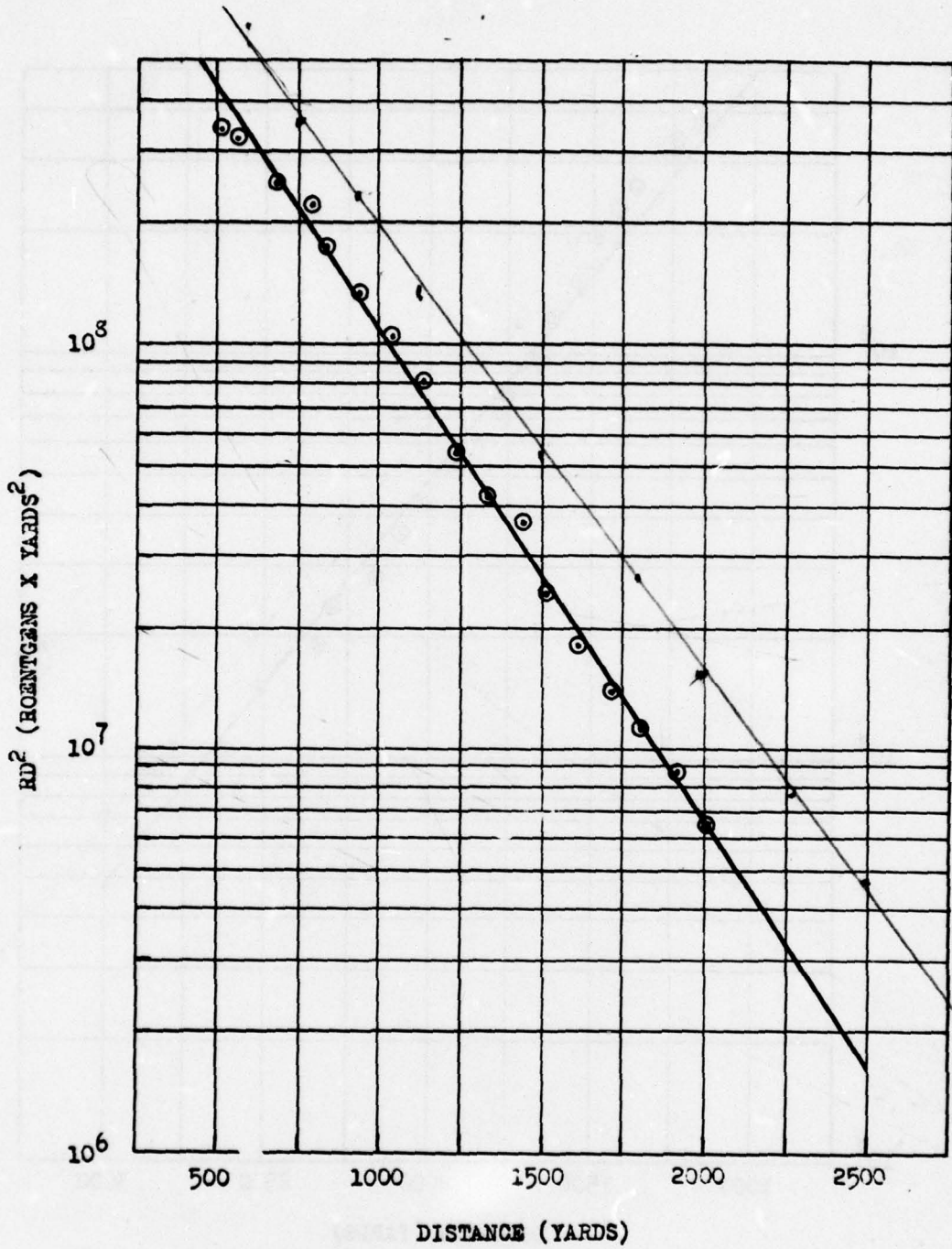
Fig. 2.1 RD^2 vs D, Shot 2
