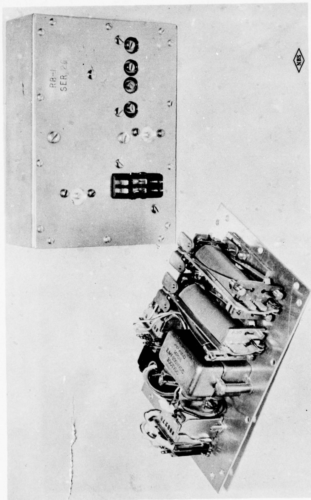
Fig. 11 —Ring box for use with telephone lines.
