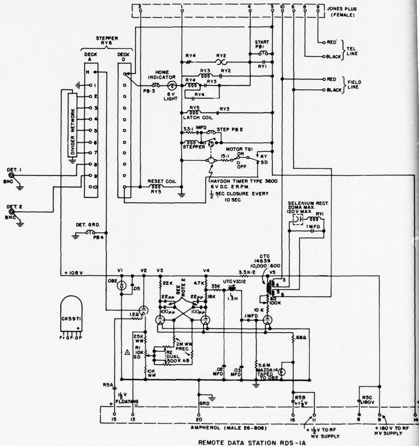
Fig. 19—Remote data station RDS-1A.
