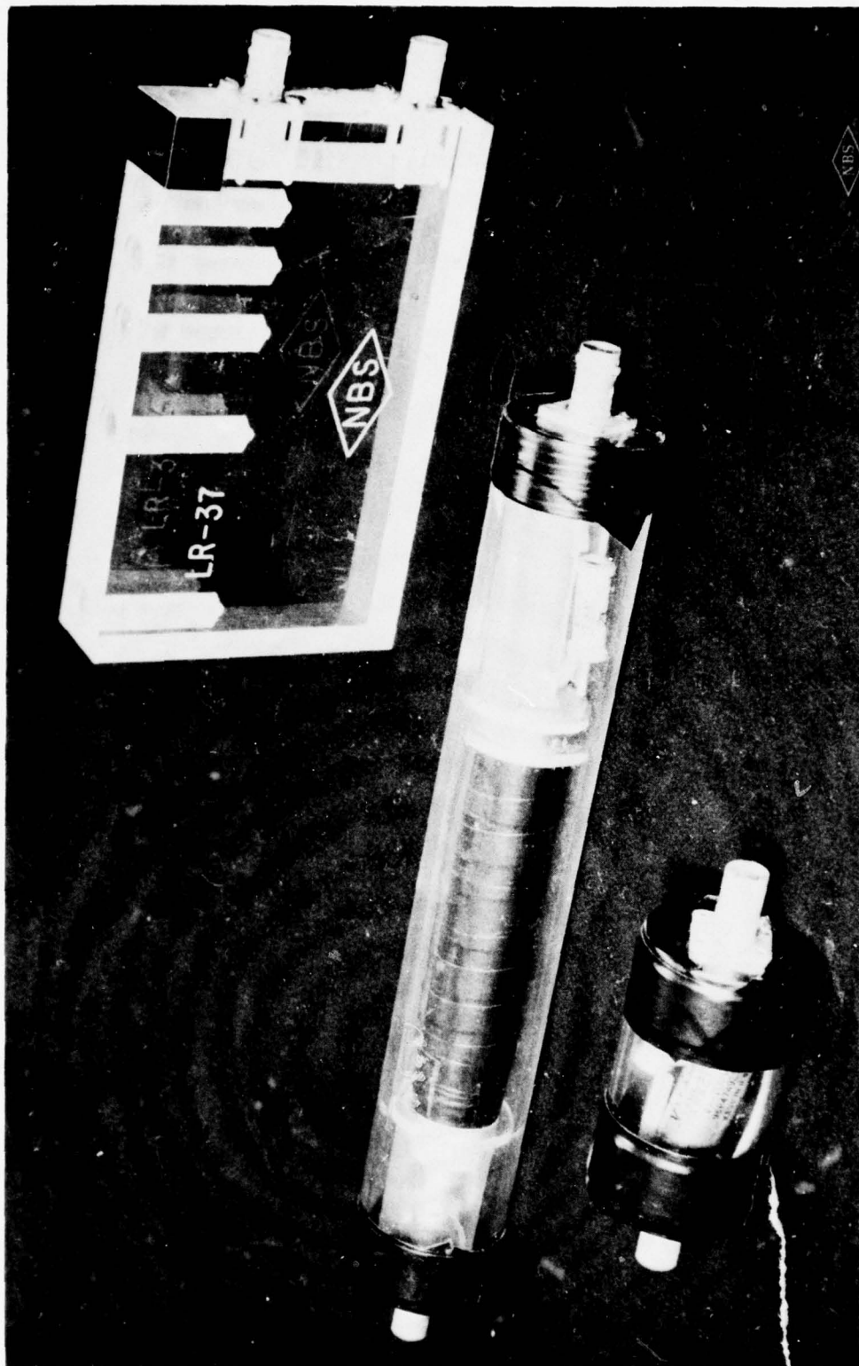
Fig. 12—Detectors and integrators. At rear is the moderate sensitivity detector (type LR), its integrator is shown in front; the sensitive detector (type VLR) is shown in the center.
