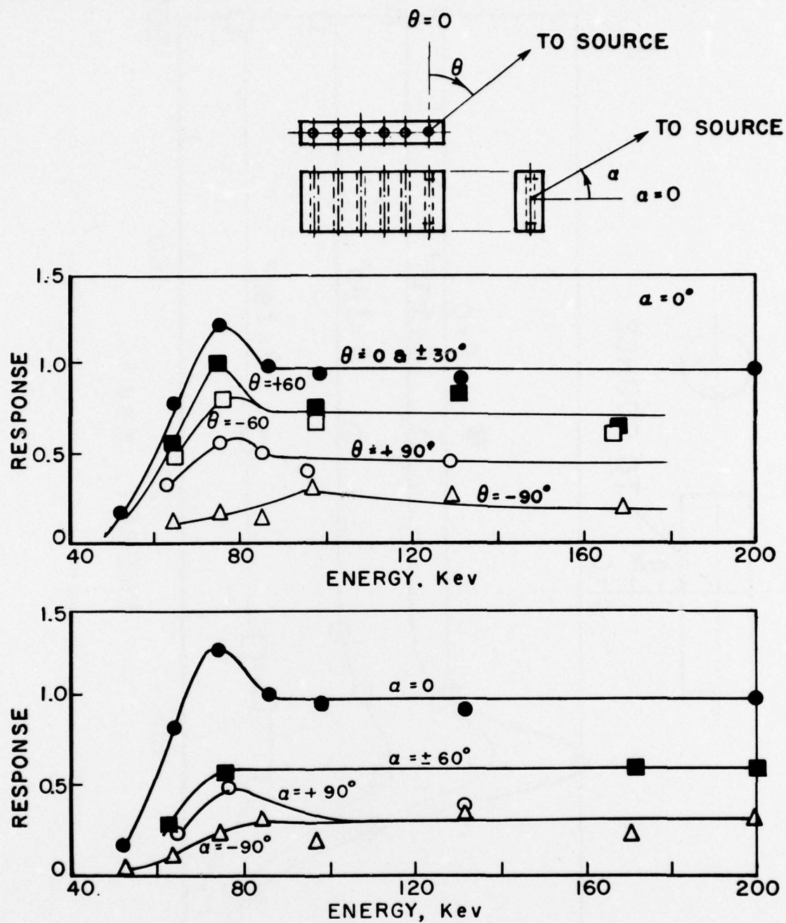
Fig. 26—Energy and directional response of LR detectors to gamma radiation.
