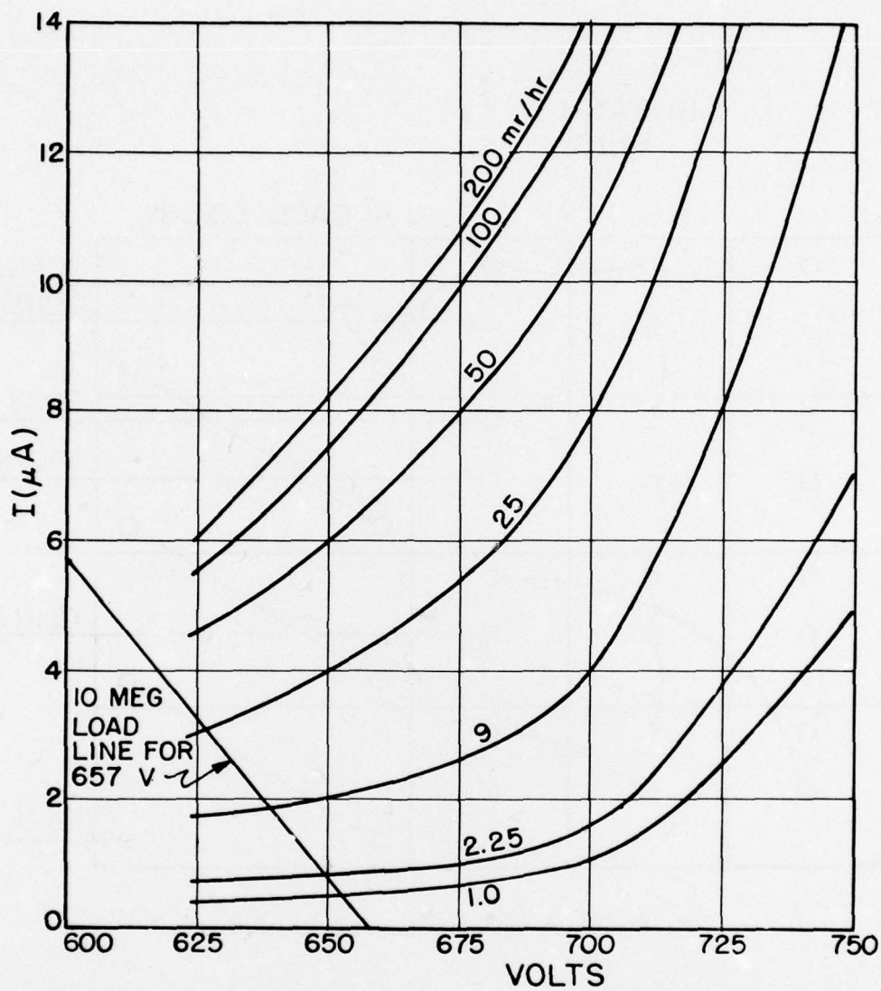
Fig. 25—Voltage—current characteristic of BS-1 counter tube (Anton).
