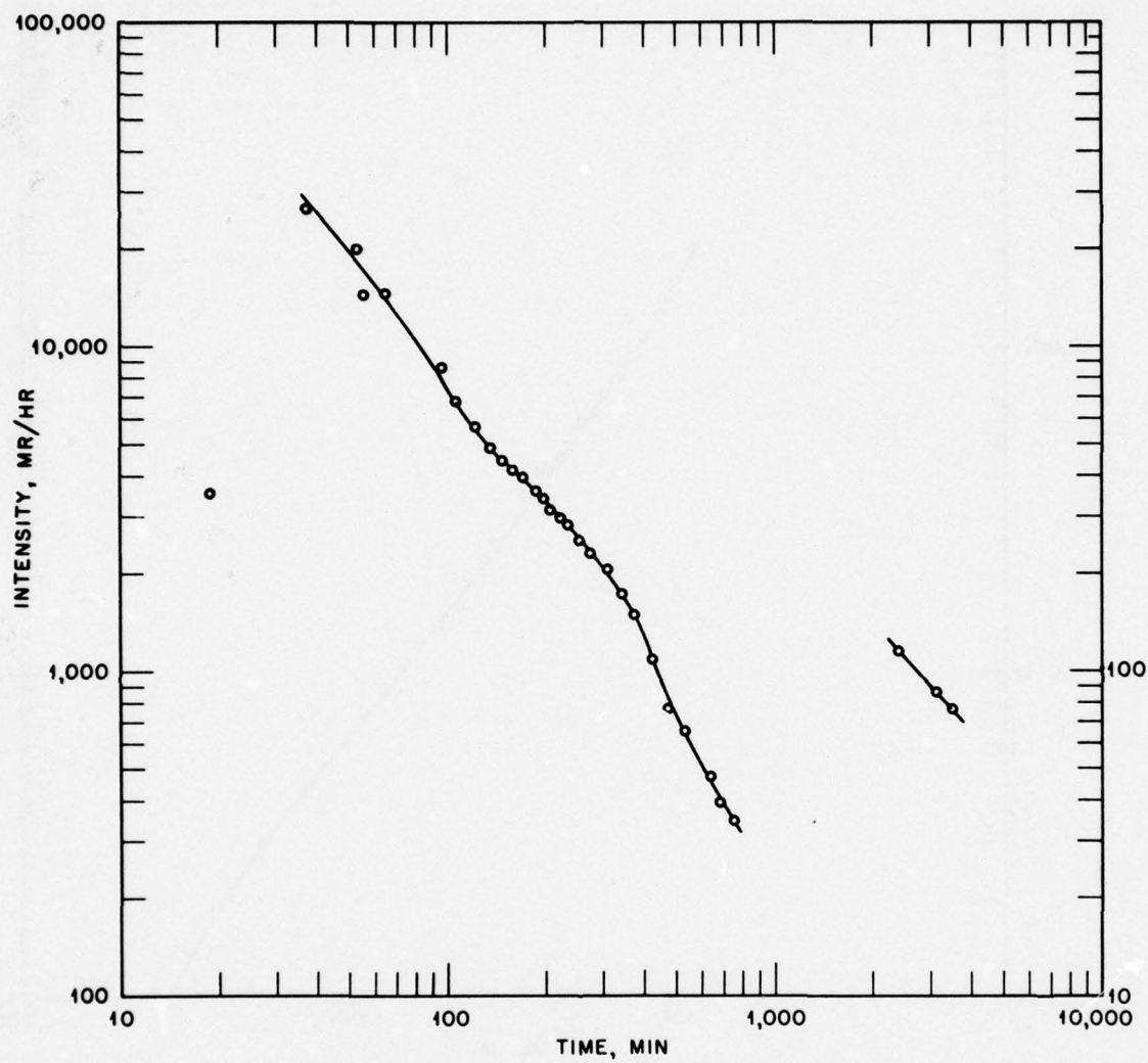
Fig. 7—Decay pattern for Butler building, left aft, shot Shasta.
