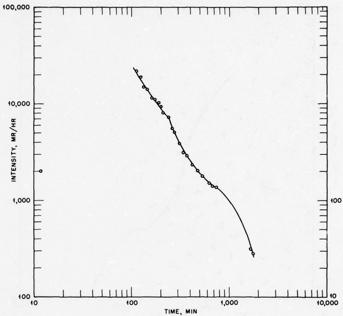
Fig. 10—Decay pattern for Project 32.3 manned shelter, left pad, shot Shasta.
