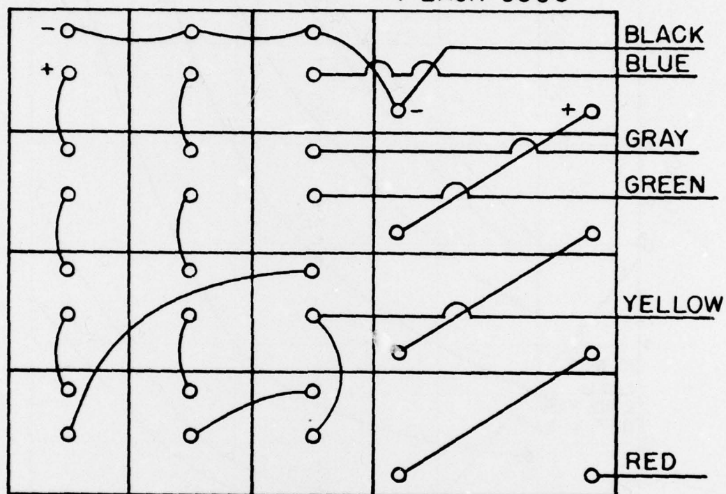
Fig. 24 — Battery wiring for remote data station RDS-1A.
