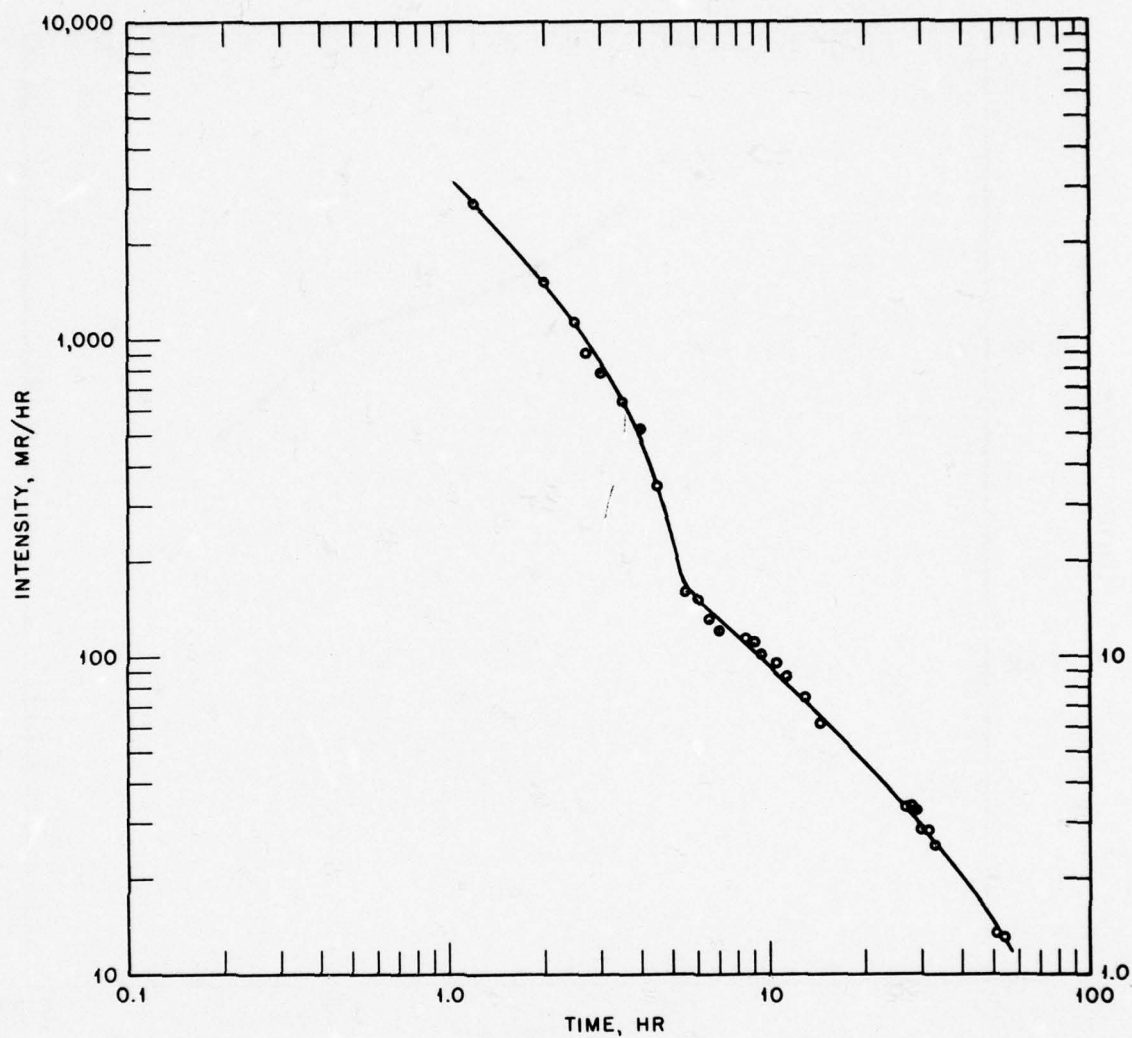
Fig. 18—Decay pattern for Project 32.3 manned shelter, center pad, shot Diablo.
