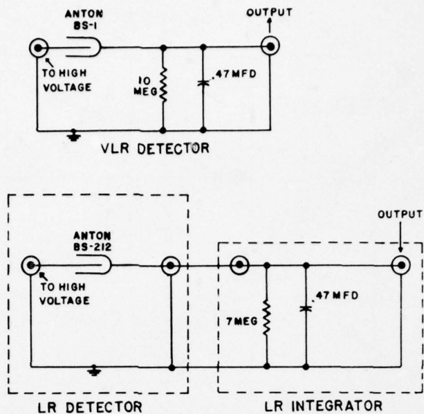
Fig. 13—Detector circuits.
