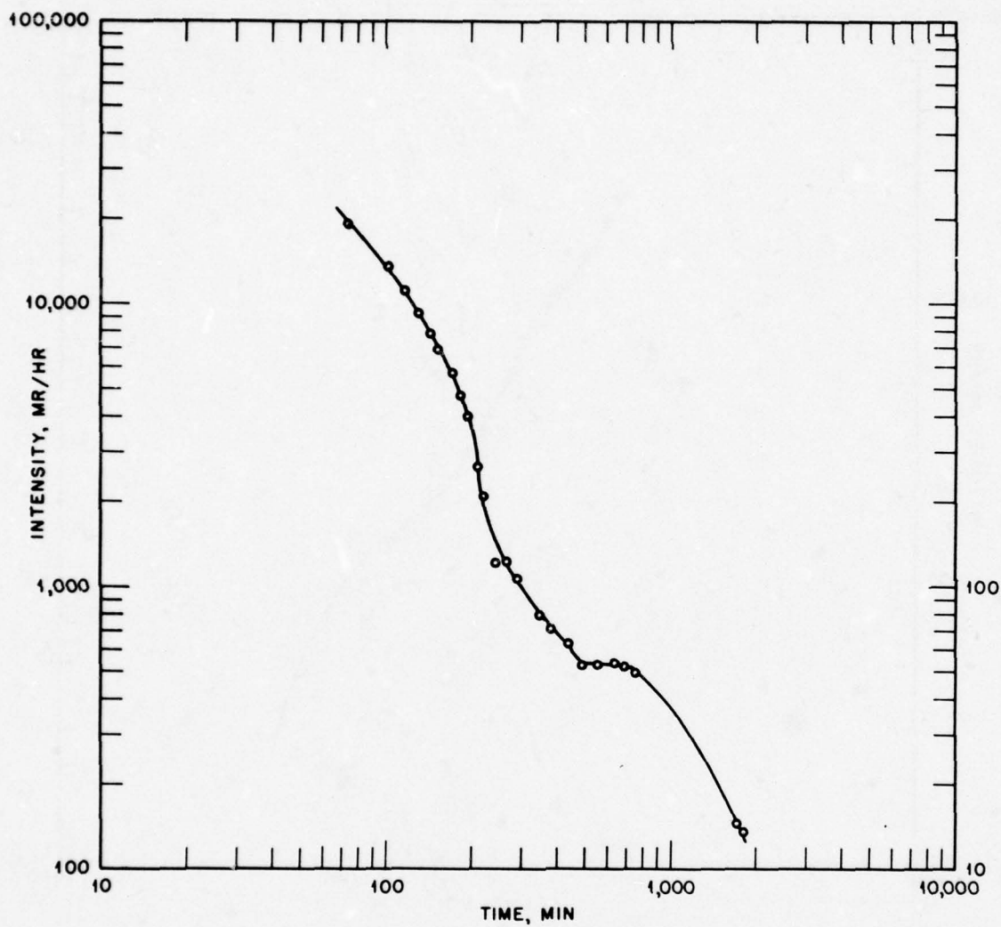
Fig. 11 — Decay pattern for Project 32.3 manned shelter, center pad, shot Shasta.
