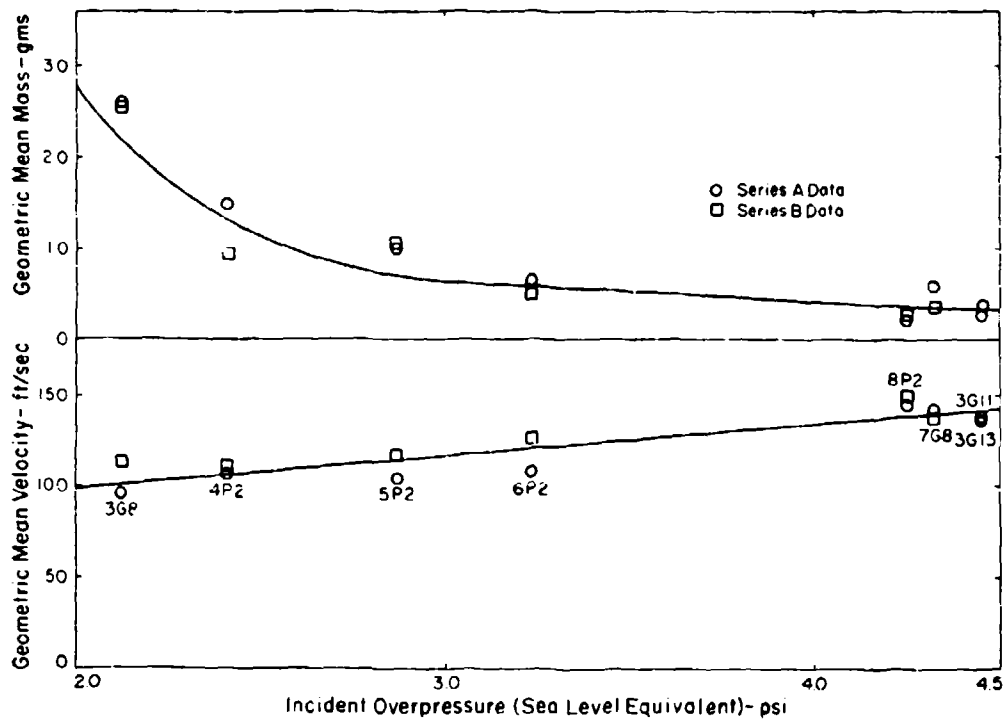
Fig. 4.14 Comparison of geometric mean velocities and masses for Series A and B missile data as a function of sea-level-equivalent incident overpressure.
