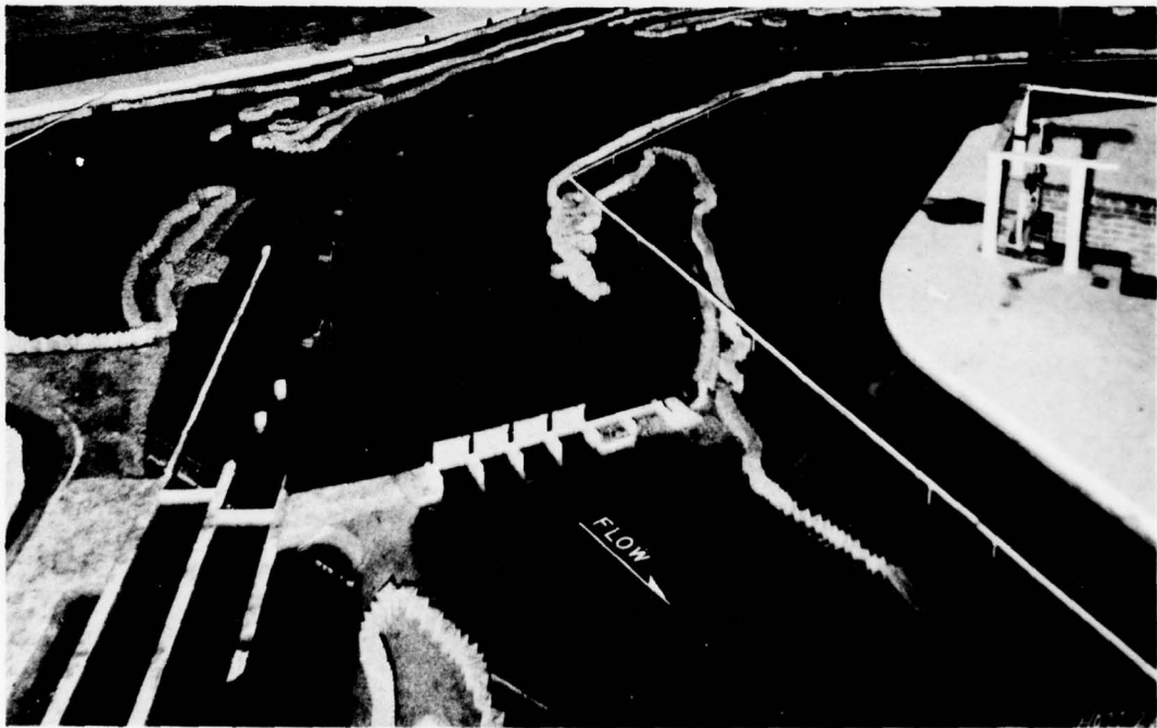
b. Path of downbound 600-ft tow approaching extended guide wall at a slight angle to wall. Note tendency for tow to be rotated clockwise
