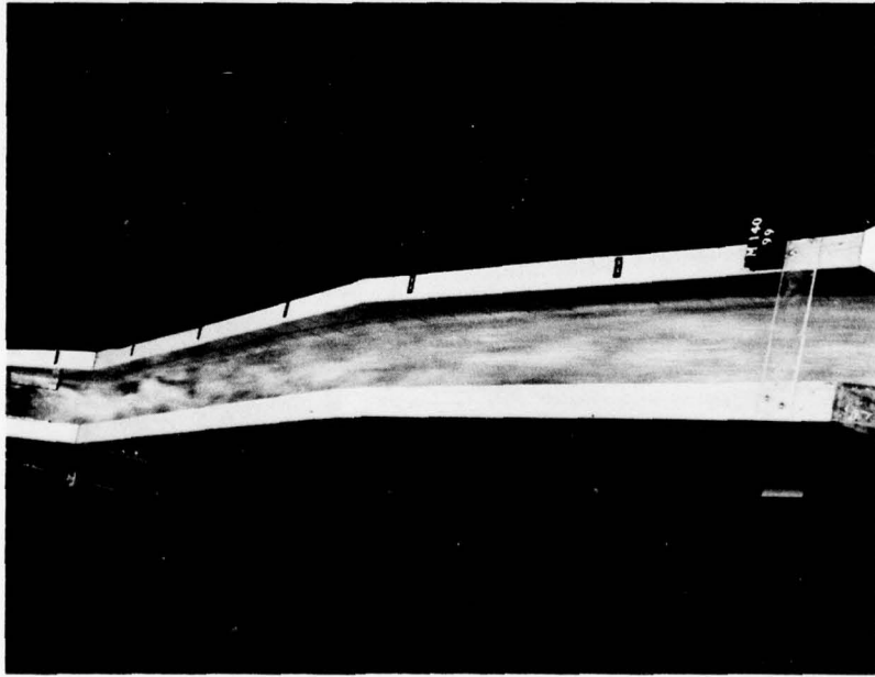
Discharge 10,000 cfs
