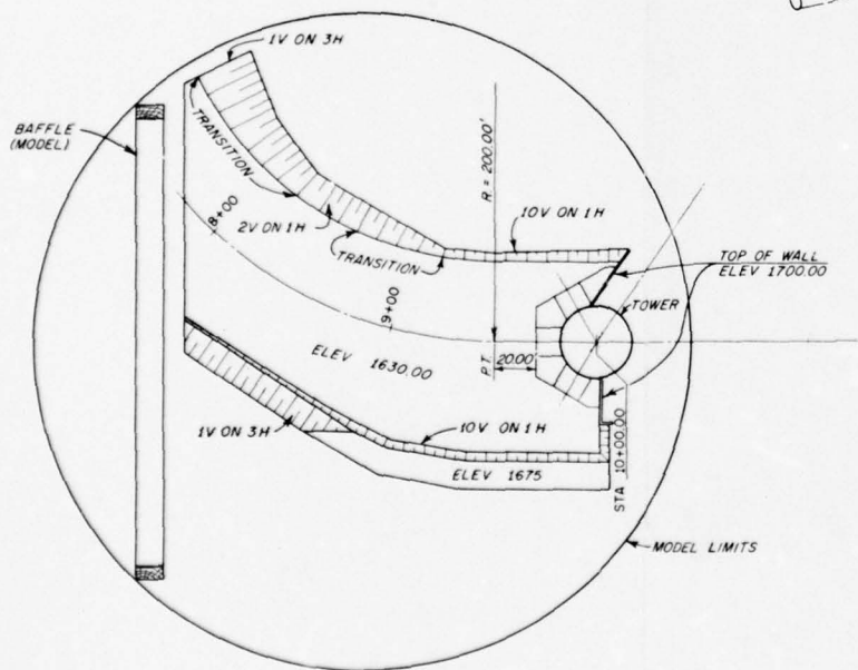
DETAIL B
