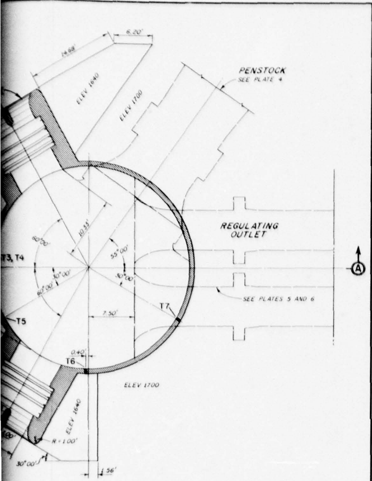
PLAN AT ELEVATION 1650 TIER NO. 1
