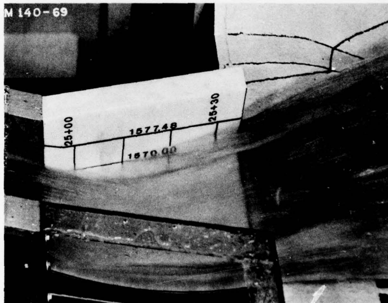
Discharge 12,000 cfs
