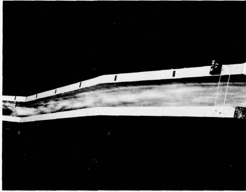
Discharge 12,000 cfs
