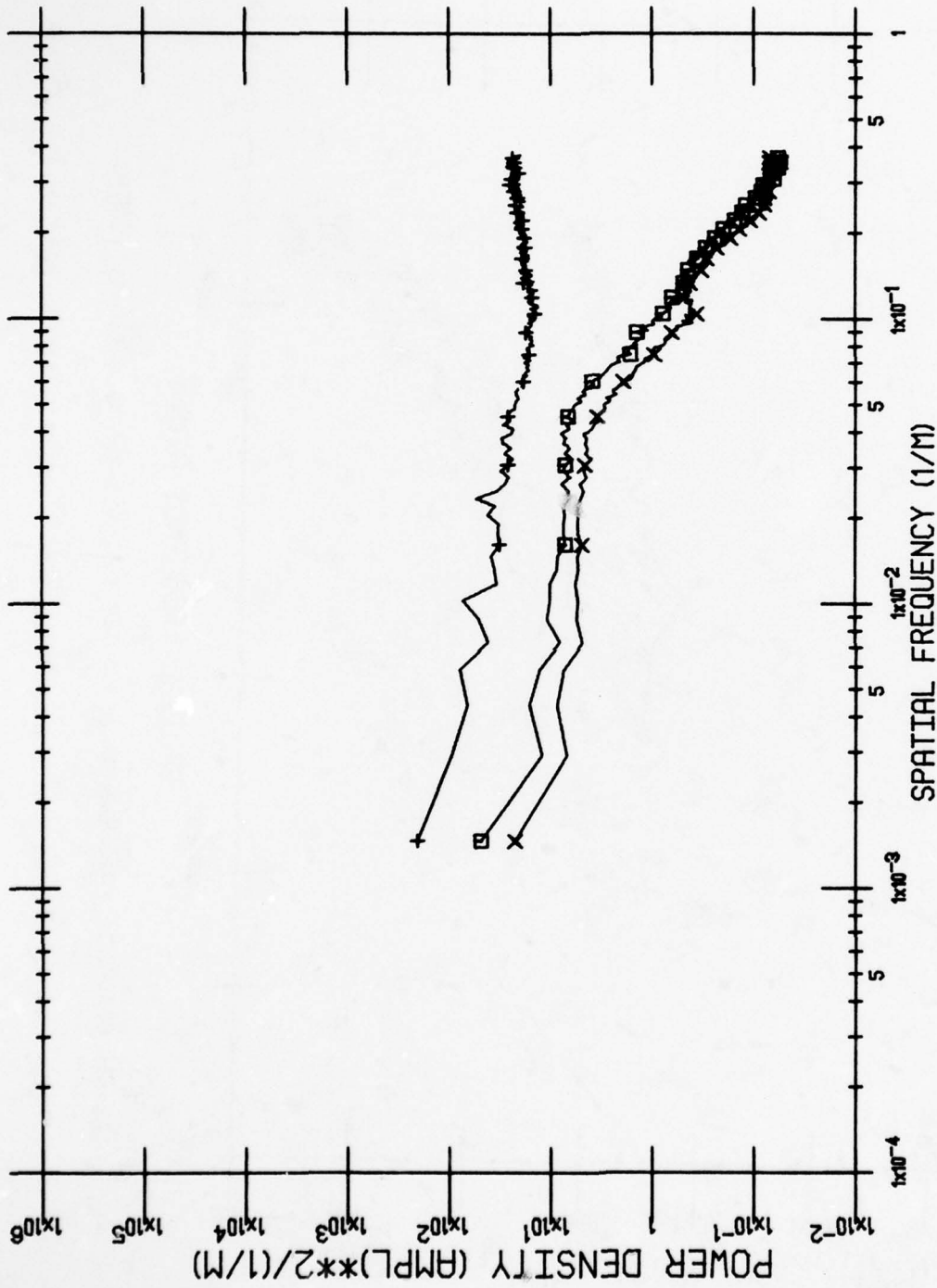
Area: FARMLAND Wavelength = 3.5-3.9 (+), 4.5-5.5 (x), 9.0-11.4 (□)
