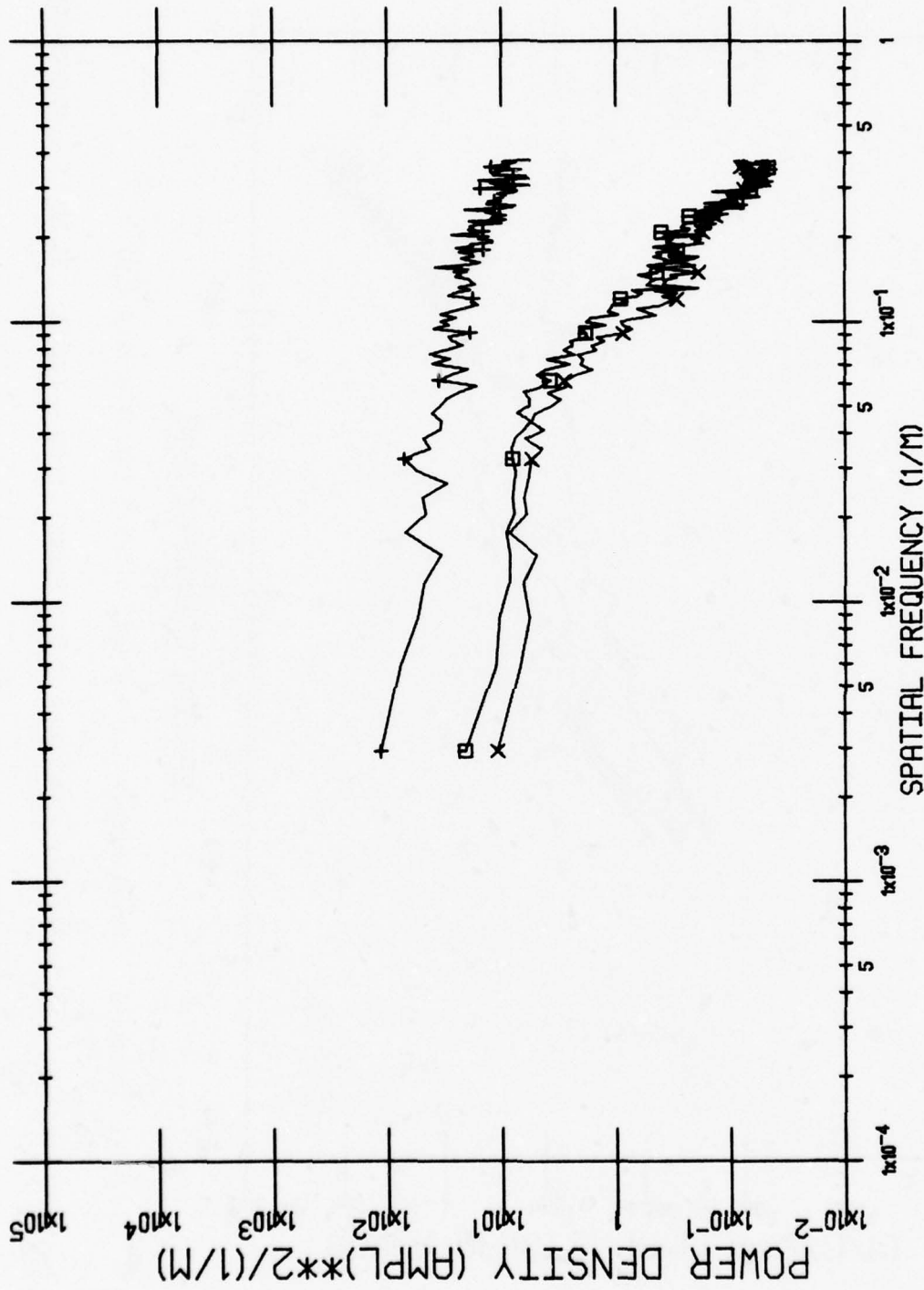
Area: FARMLAND Wavelength = 3.5-3.9 (+), 4.5-5.5 (x), 9.0-11.4 (□)
