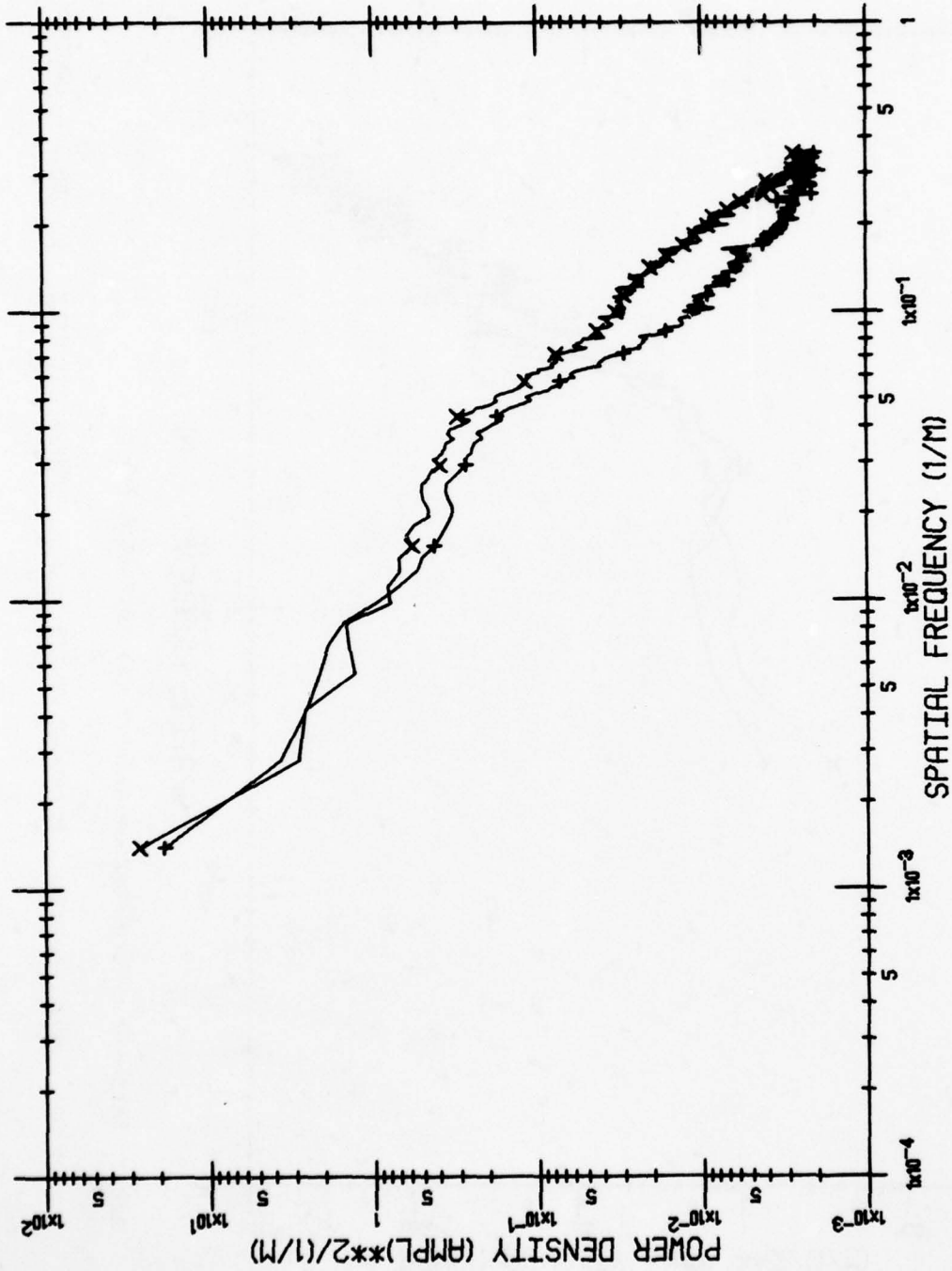
Area: FARMLAND Wavelength = 4.5-5.5 (+), 9.0-11.4 (X)
