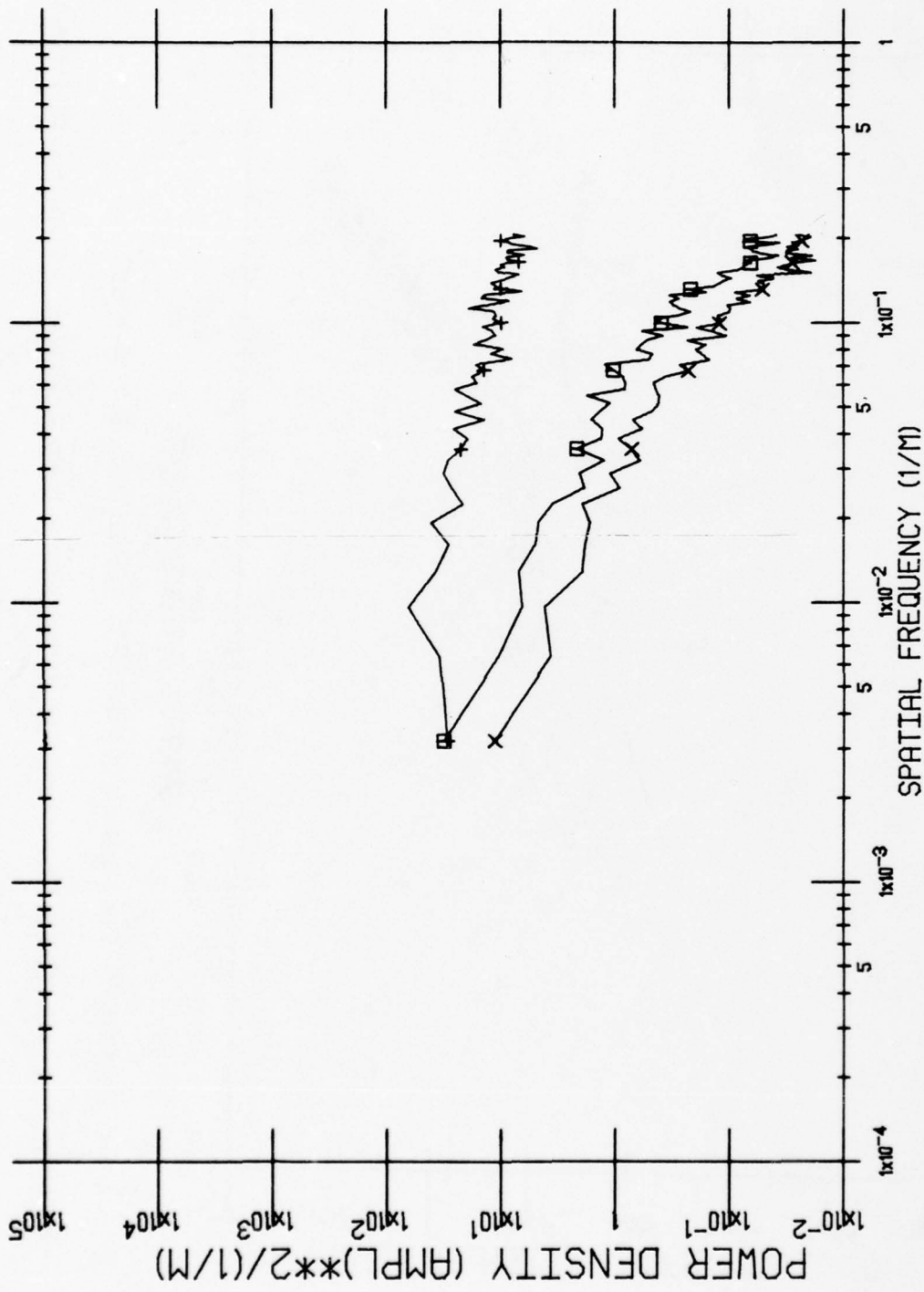
Area: CONIFERS Wavelength = 3.5-3.9 (+), 4.5-5.5 (x), 9.0-11.4 ( \square )
