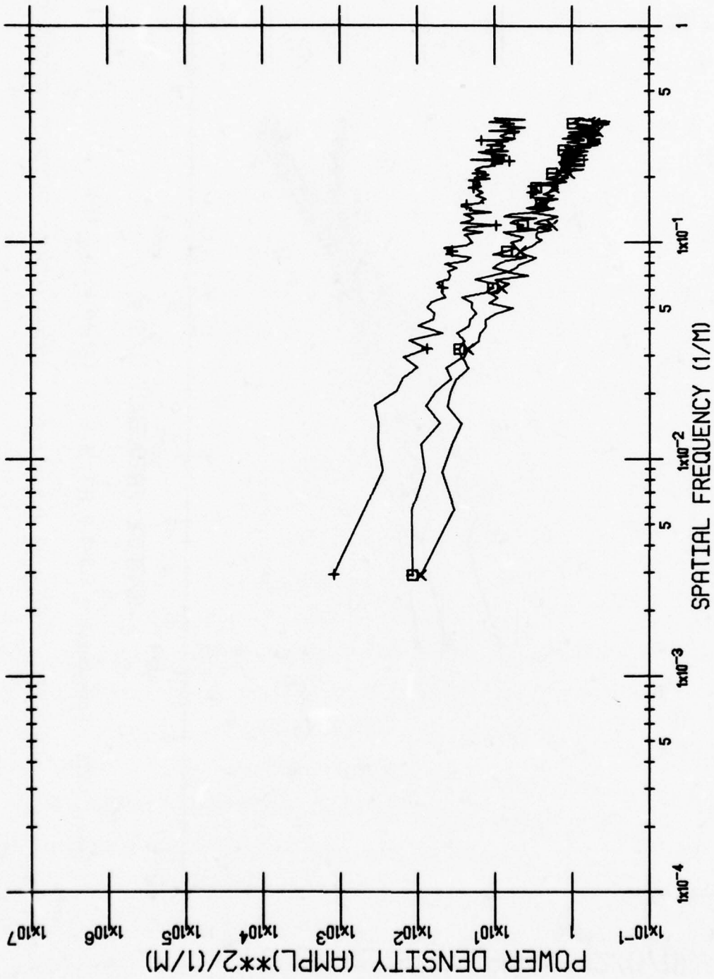
Area: CITY Wavelength = 3.5-3.9 (+), 4.5-5.5 (x), 9.0-11.4 (□)
