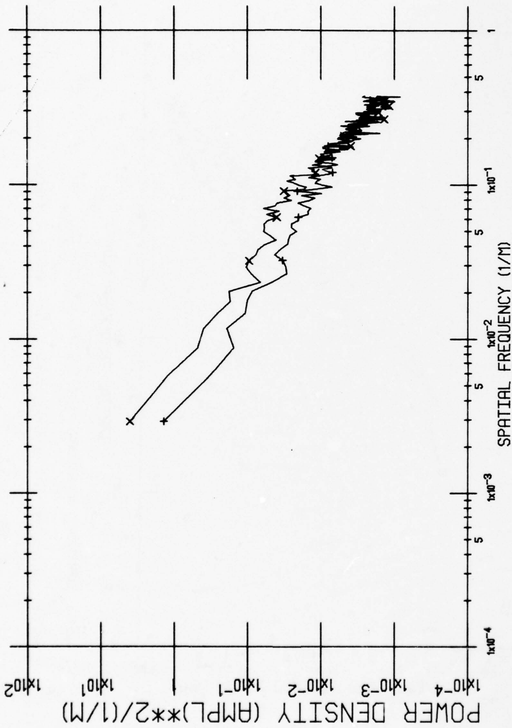
Area: CONIFERS Wavelength = 4.5-5.5 (+), 9.0-11.4 (x)
