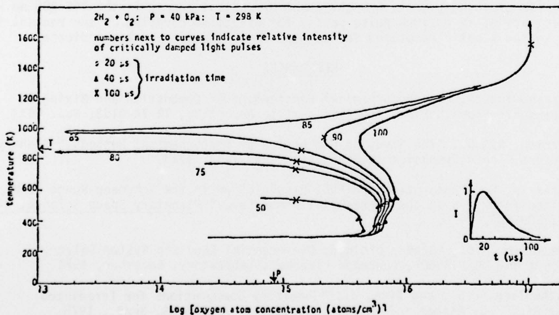
FIGURE 2 REACTANT MIXTURE PHASE PLANE PATHS DURING PULSED VACUUM ULTRAVIOLET IRRADIATION
