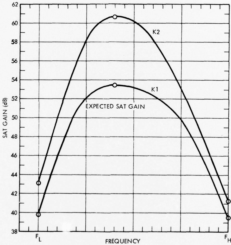
Figure 4-8. Expected Performance - SIM K1, K2.
