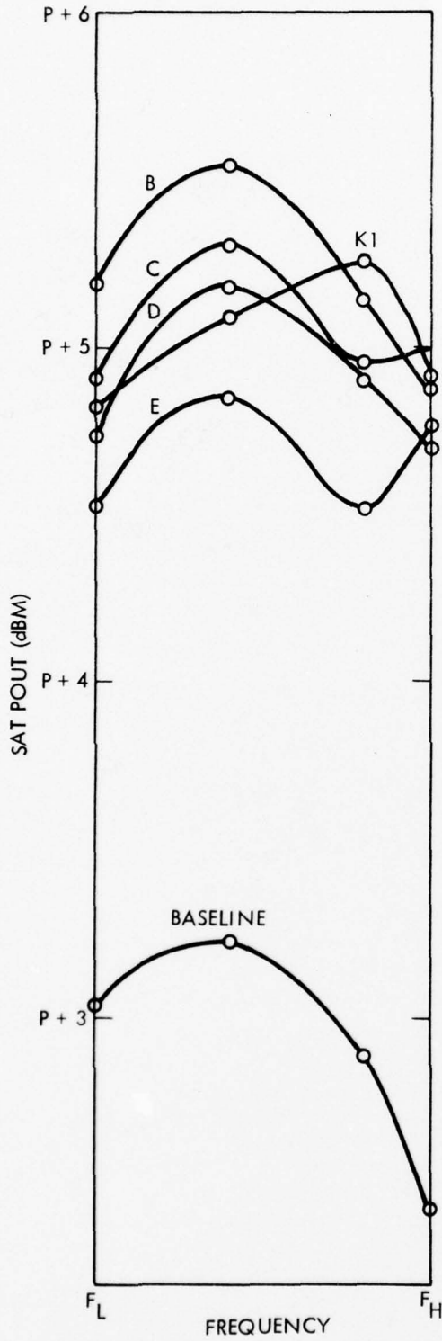
Figure 4-5. Computer Results - CW - Buffer Tail Variation.
