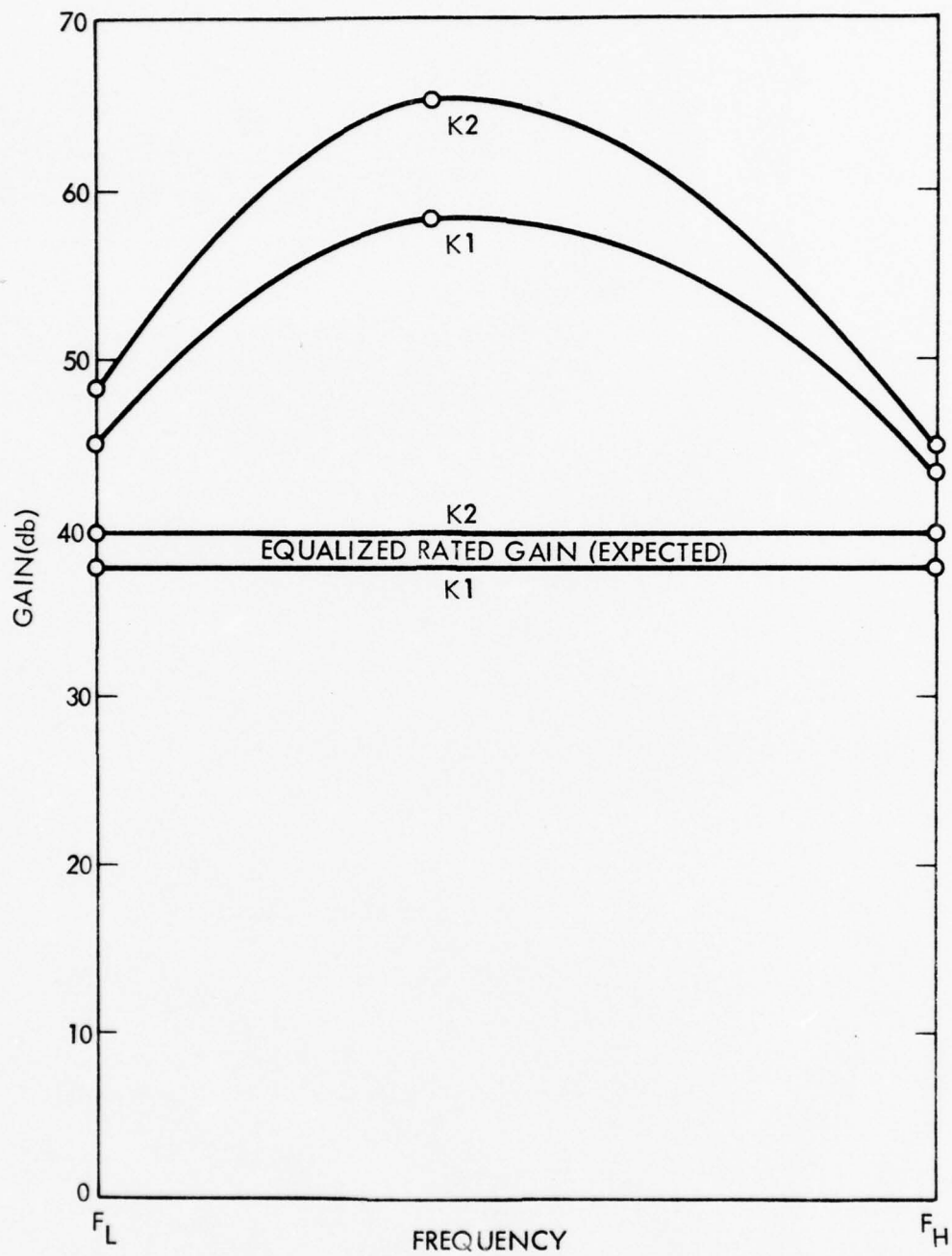
Figure 4-11. Saturated Gain.
