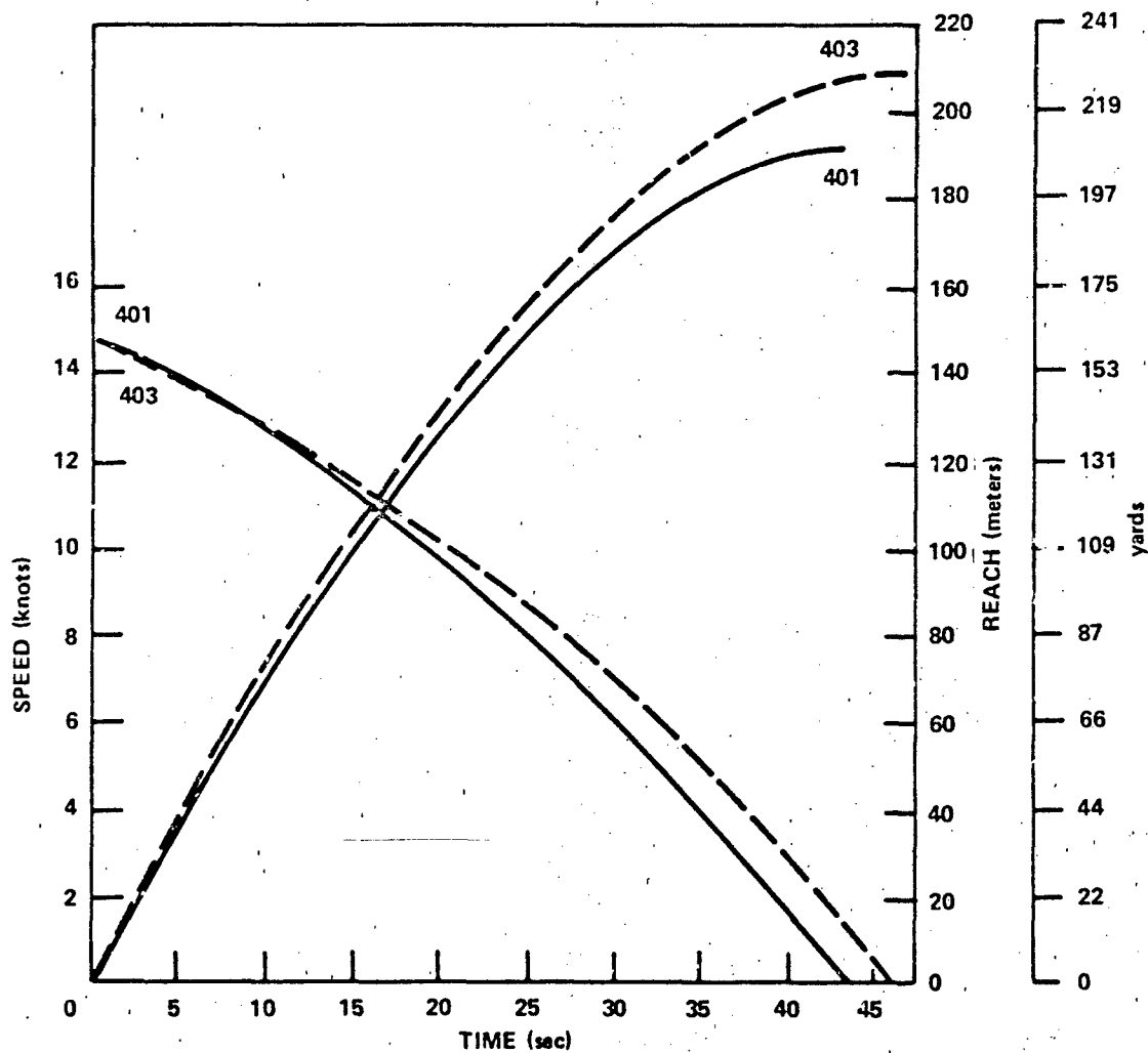
Figure 8 - CGC KATMAI BAY (WTG3-101) Deceleration from Full Ahead Power Using Full Power Astern
